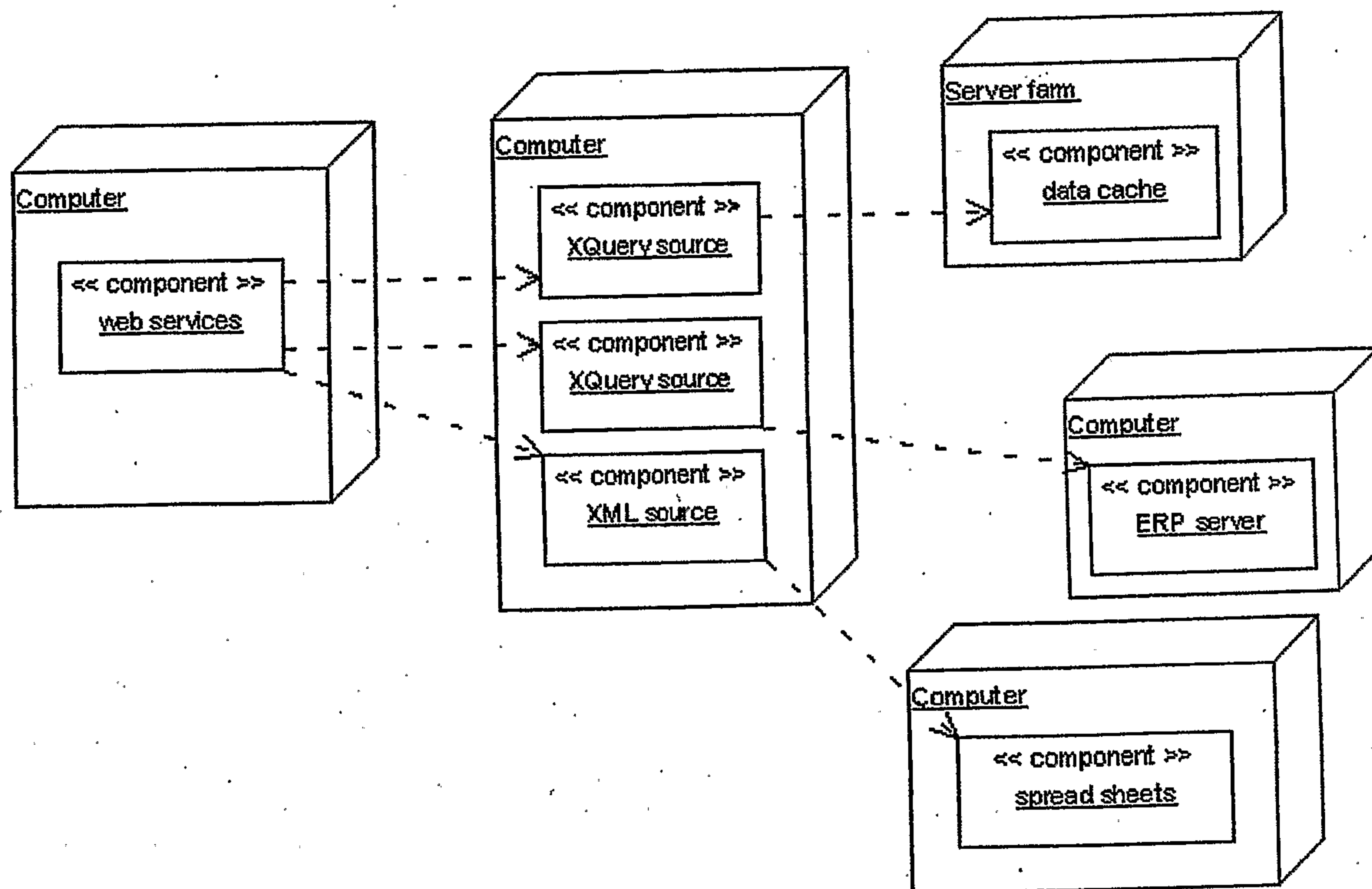
Fig. 5: information integration framework (UML component diagram)
