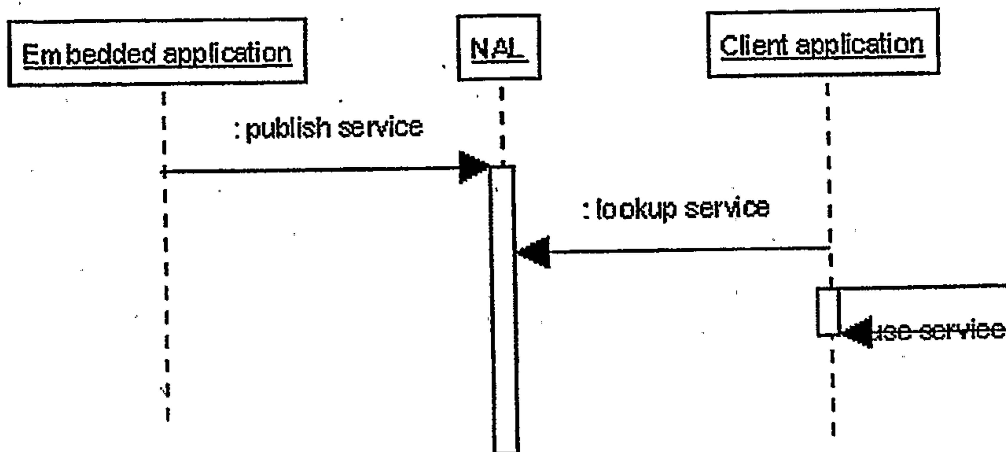
Fig. 7: Microkernel management (UML sequence diagram)
