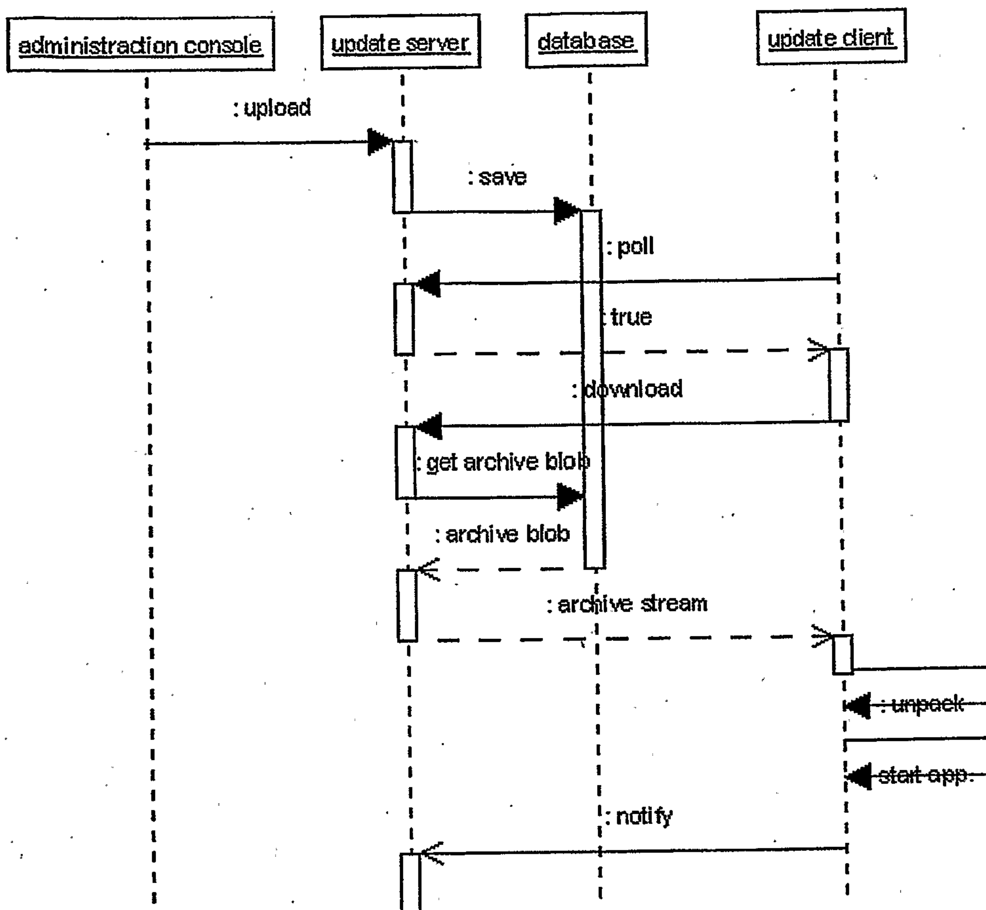
Fig. 9: Devices and data processing (UML sequence diagram)
