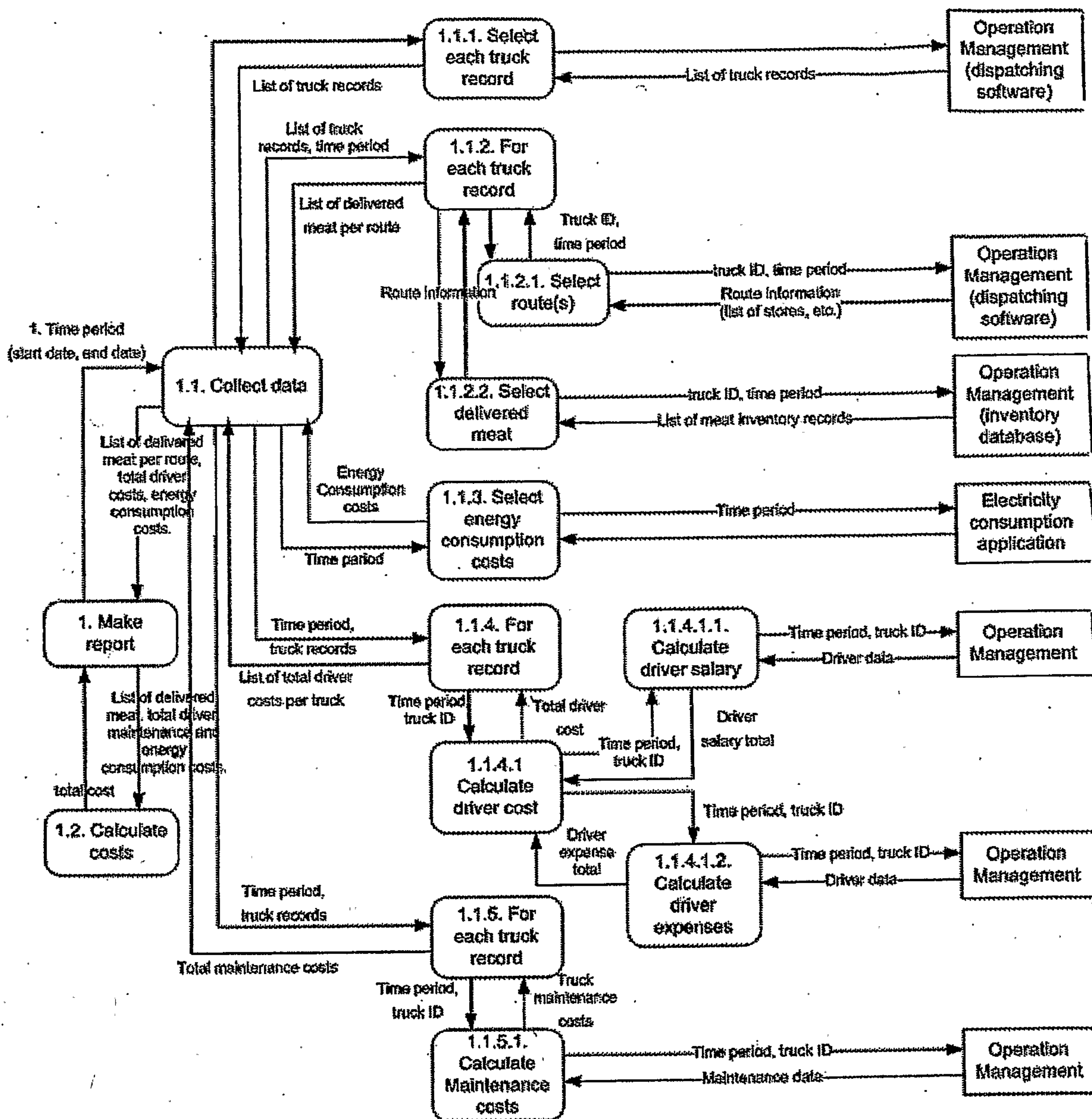
Fig. 12: is a data flow diagram of the enterprise asset management framework
