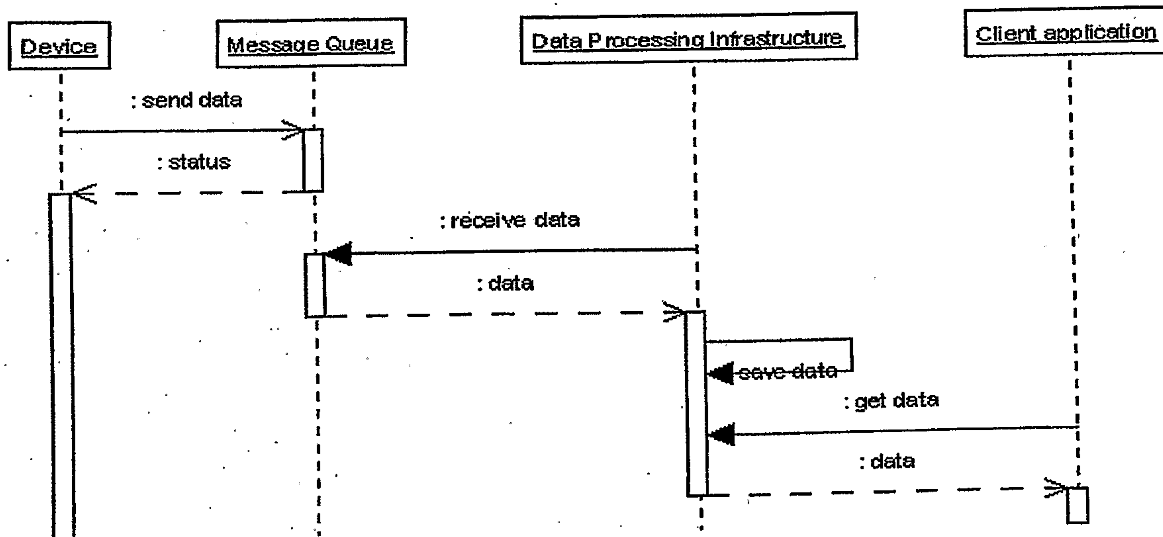
Fig. 9: Devices and data processing (UML sequence diagram)
