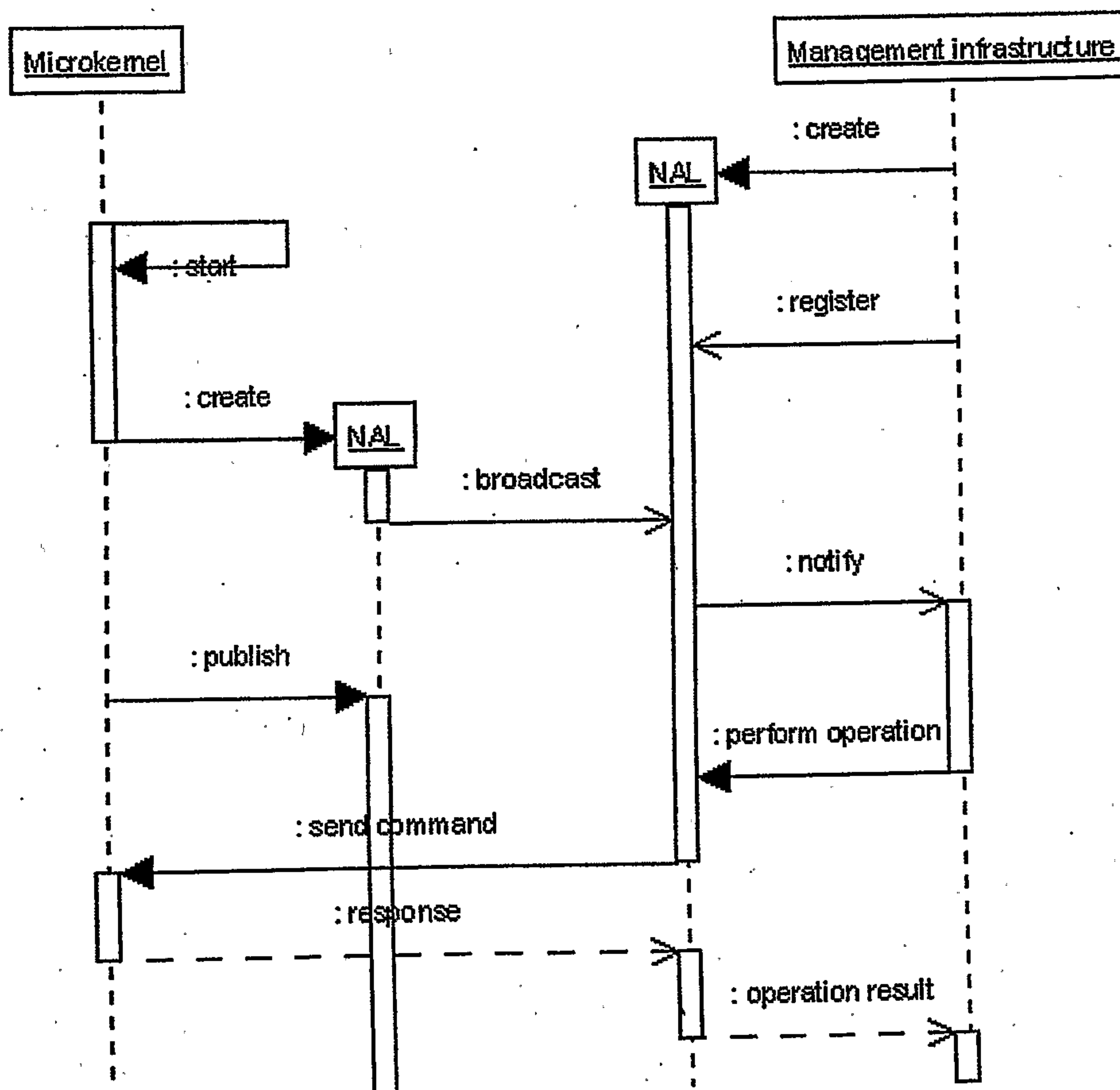
Fig. 7: Microkernel management (UML sequence diagram)
