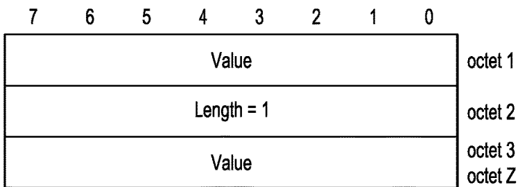
Figure 8.2.X.3-1: AT_APN_RESP attribute Value
