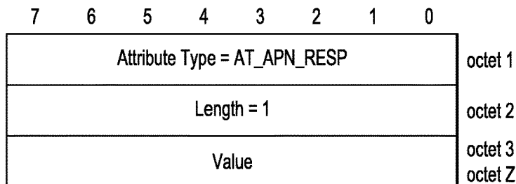
Figure 8.2.X.3-1: AT_APN_RESP attribute
