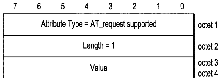
Figure 8.2.X.1-1: AT_APN_Request Supported attribute
