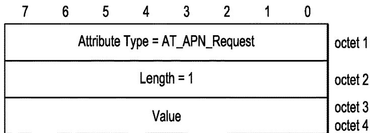
Figure 8.2.X.2-1: AT_APN_Request attribute
