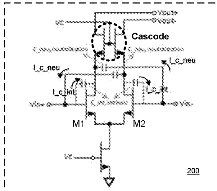
Cascode Amplifier with Neutralization
