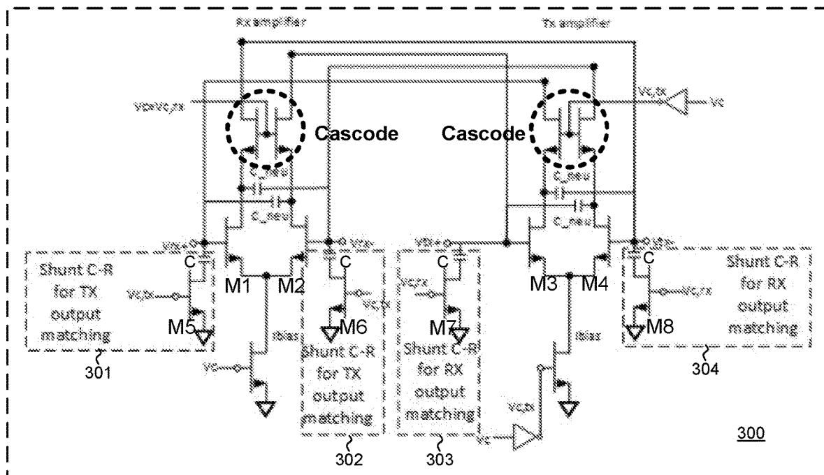
Cascode Bi-Directional Amplifier
