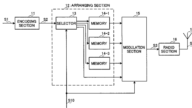
10 TRANSMITTING APPARATUS
