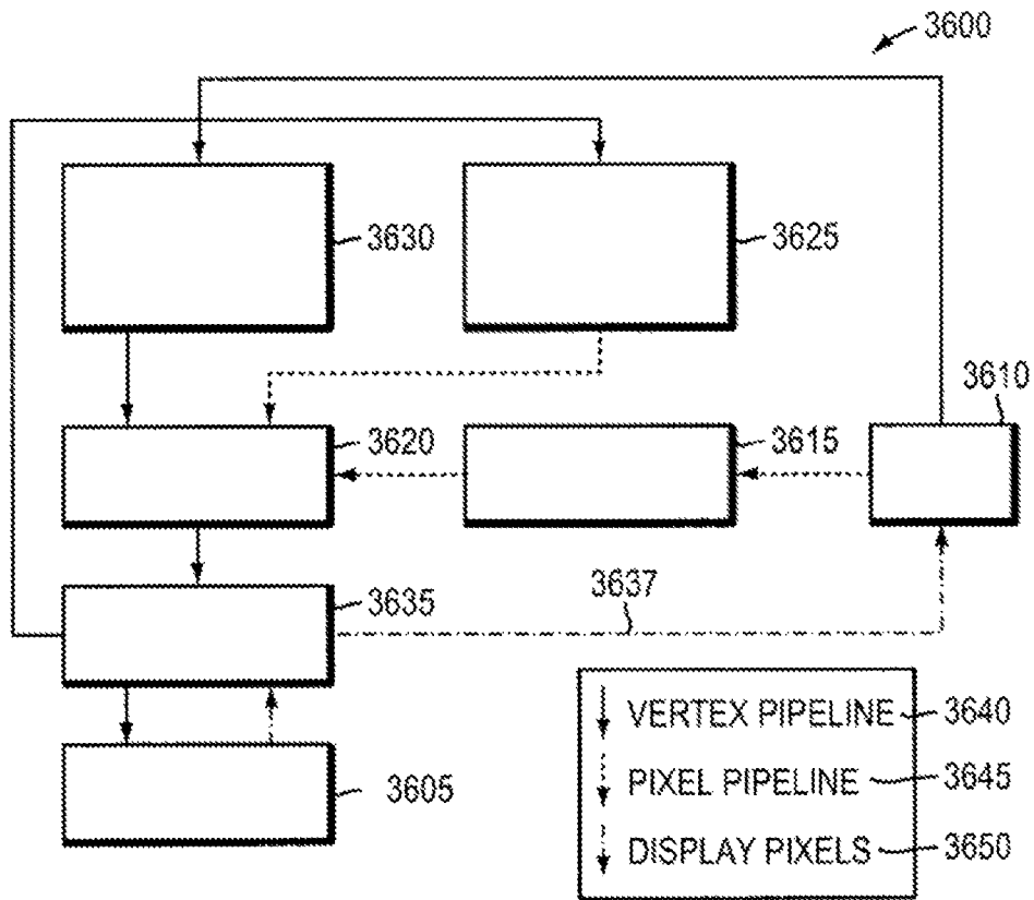
EXAMPLE OF MODERN GPU ARCHITECTURE (XBOX 360)
