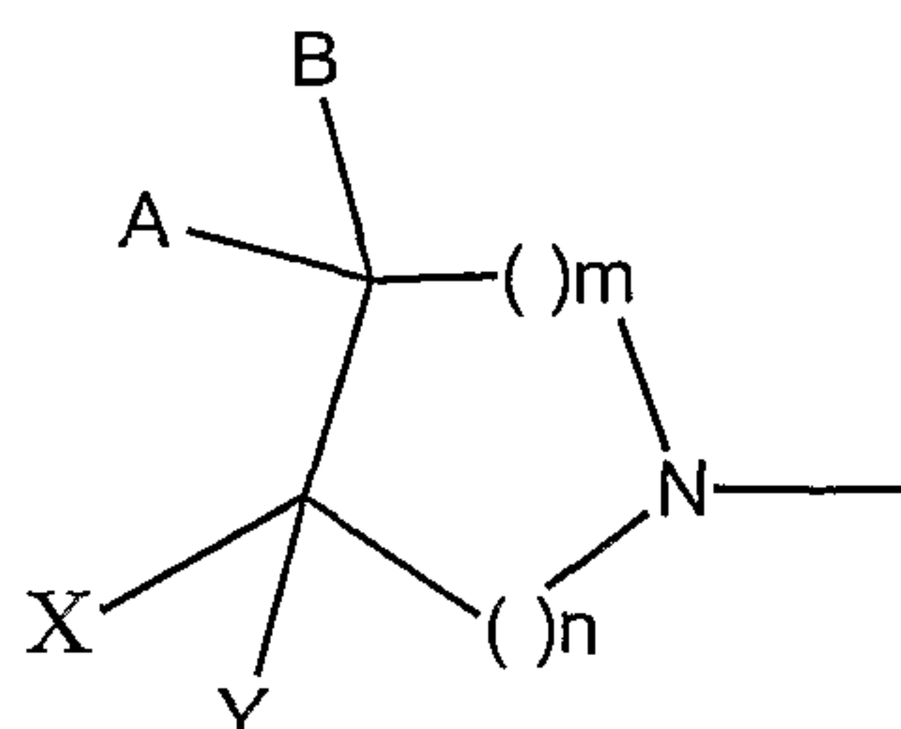
Formula II
