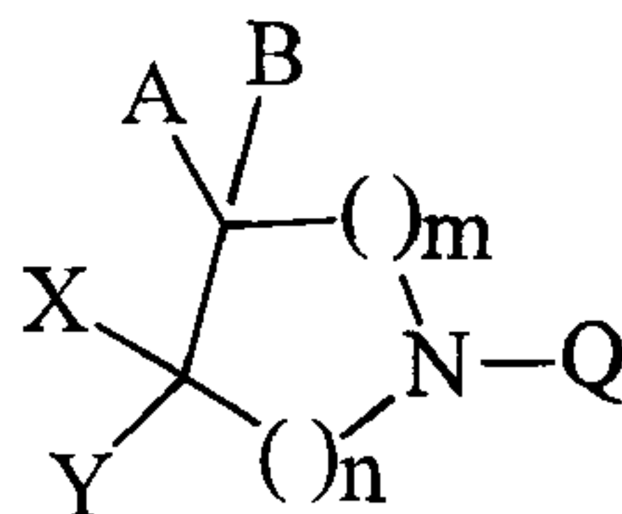
Formula I
