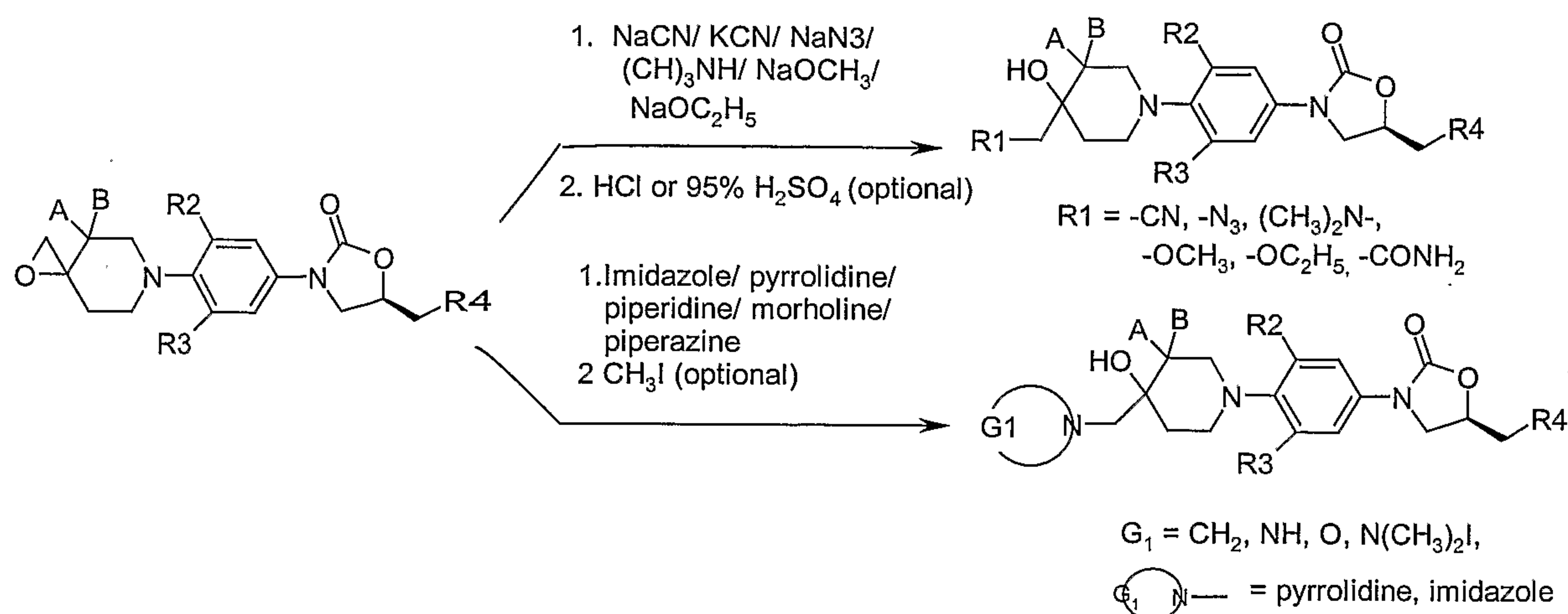
Scheme-9
