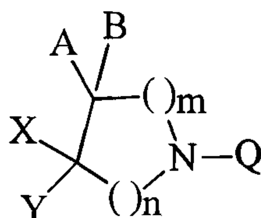
Formula I
