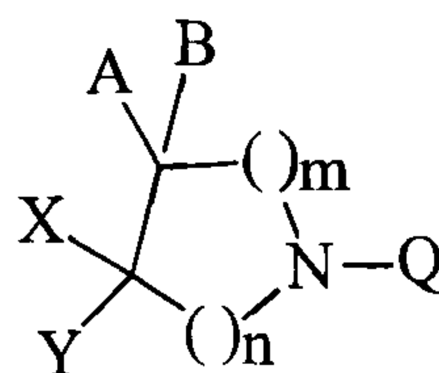
Formula I
