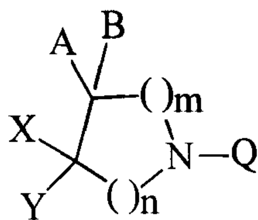
Formula I
