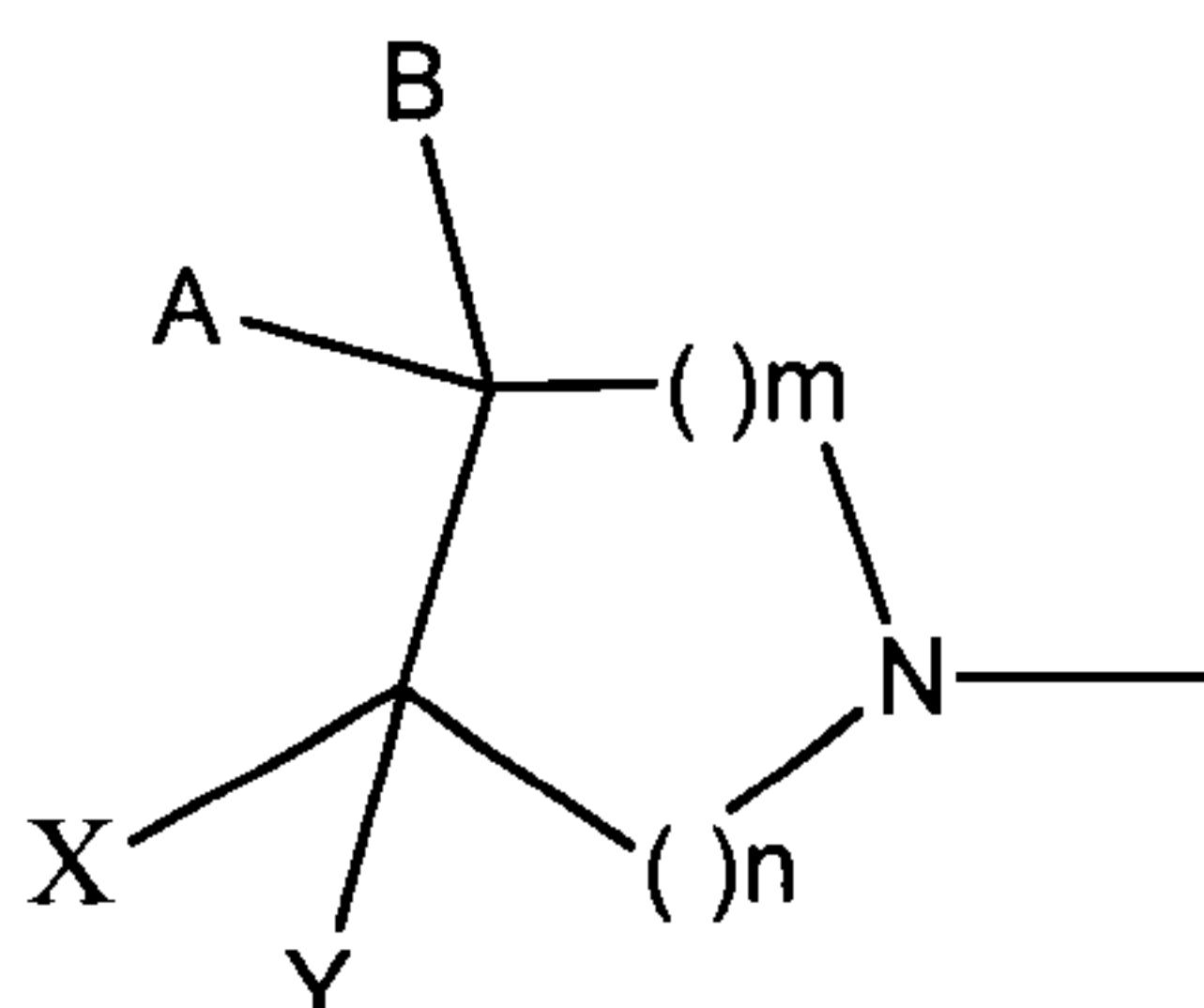
Formula II
