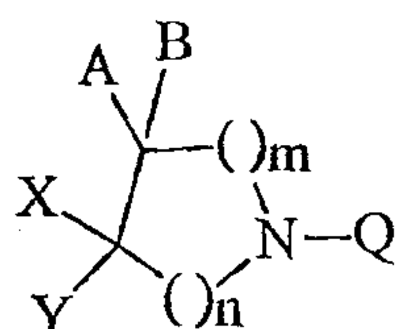
Formula I
