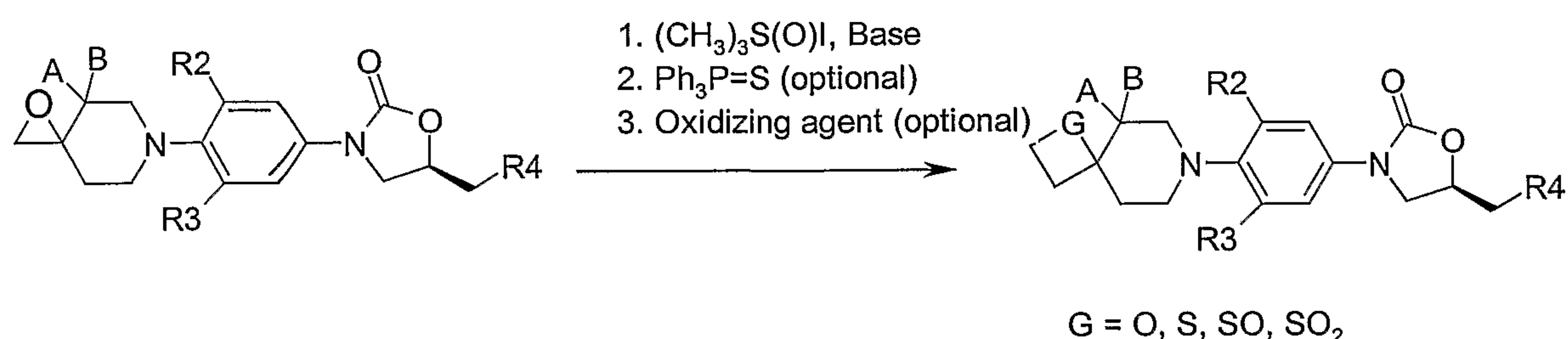
Scheme -2
