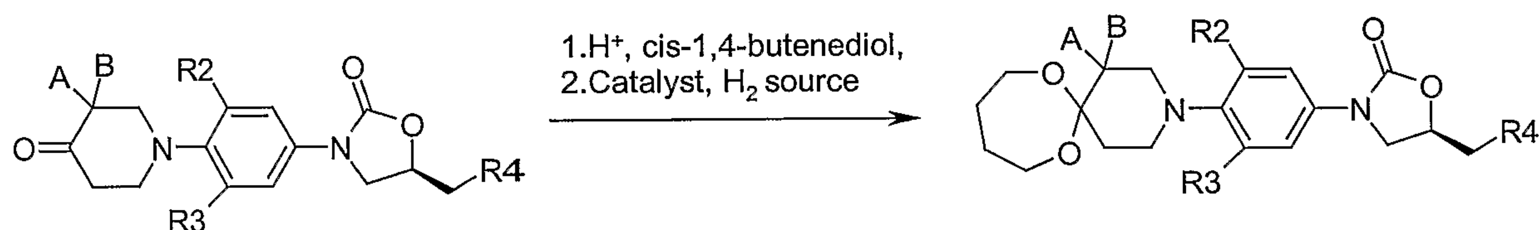
Scheme-7
