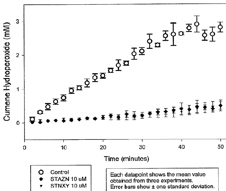
Autooxidation of Cumene (80% cumene in C 6 D 6 )
