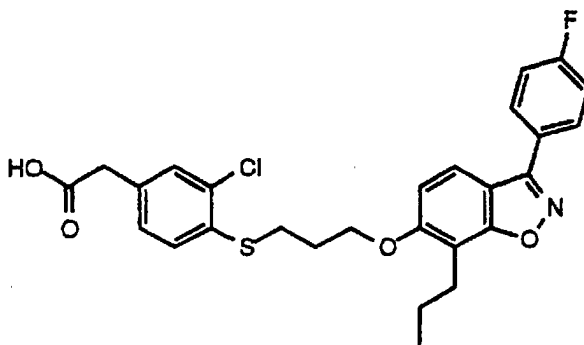
3-Chloro-4-(3-(3-(4-fluorophenyl)-7-propyl-6-benz-[4,5]-isoxazoloxy)-propylthio)phenylacetic acid
