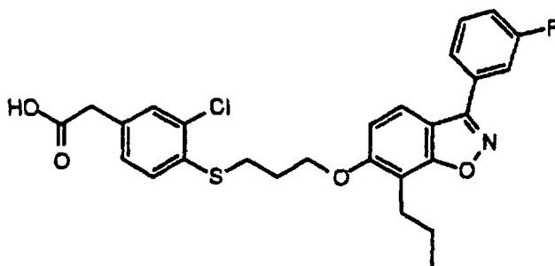
3-Chloro-4-(3-(3-(3-fluorophenyl)-7-propyl-6-benz-[4,5]-isoxazoloxy)-propylthio)phenylacetic acid
