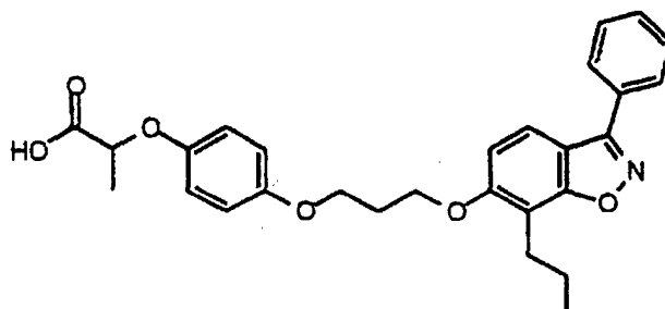
2-(4-(3-(3-phenyl-7-propyl-6-benz-[4,5]-isoxazoloxy)propyloxy)) phenoxypropionic acid
