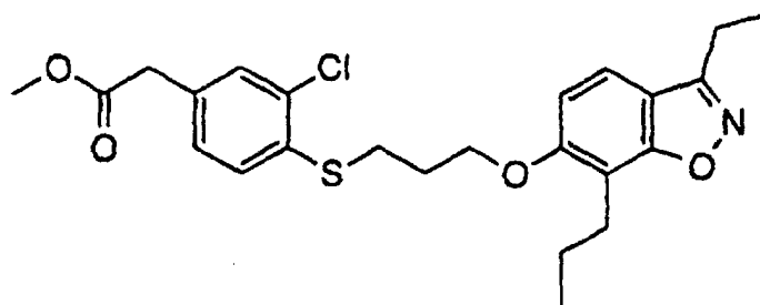
Methyl 3-chloro-4-(3-(3-ethyl-7-propyl-6-benz-[4,5]-isoxazoloxy)-propylthio)phenylacetate
