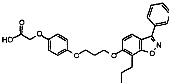
4-(3-(3-phenyl-7-propyl-6-benz[4,5]isoxazole)oxy)propyloxy phenoxy acetic acid
