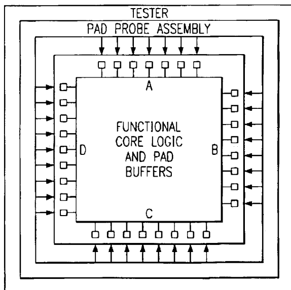
FIG. 4 (PRIOR ART)
