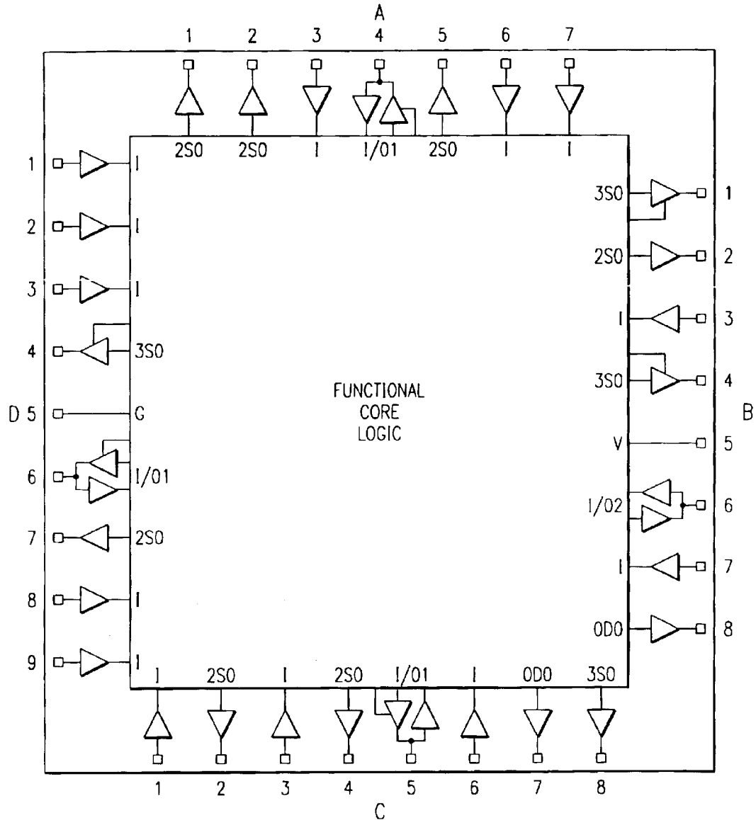
FIG. 1 (PRIOR ART)
