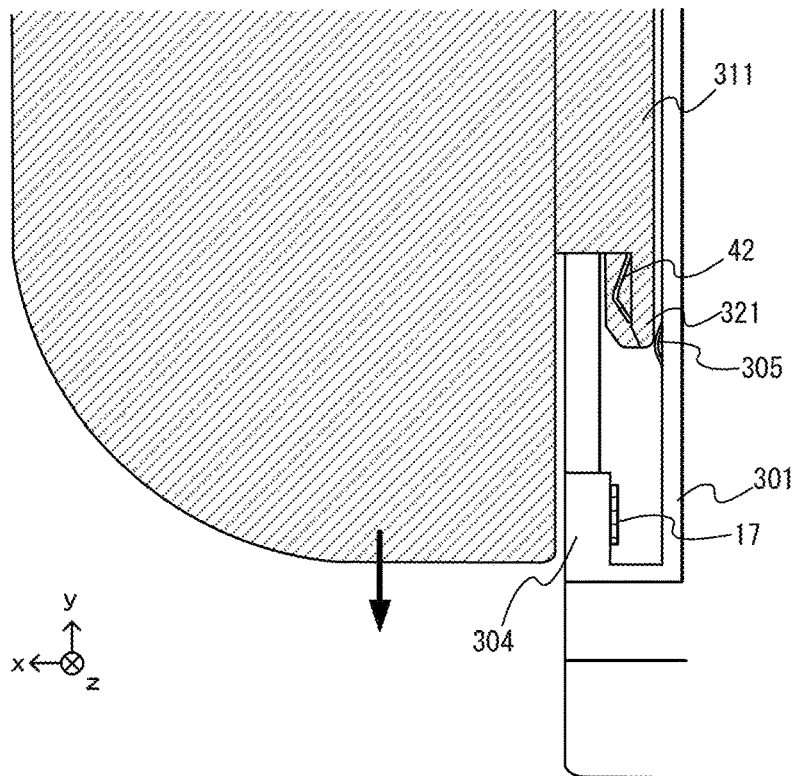
Fig. 26(b) ATTACHED STATE
