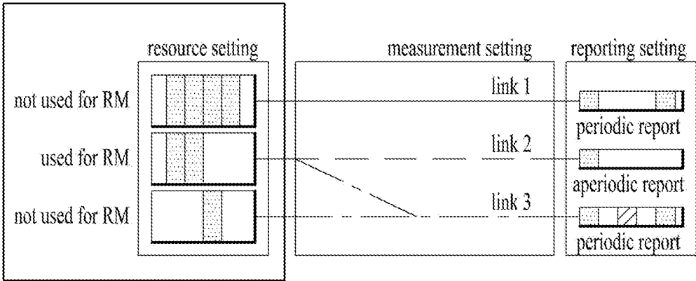
CSI acquisition/beam management framework
