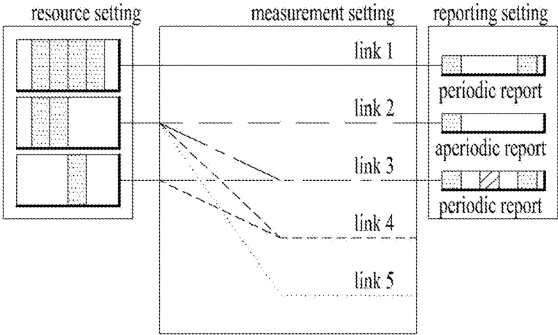
CSI acquisition/beam management framework
