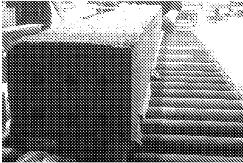
FIG. 6. A photograph of an actual railroad tie (without reinforcing bar) according to an embodiment of the invention
