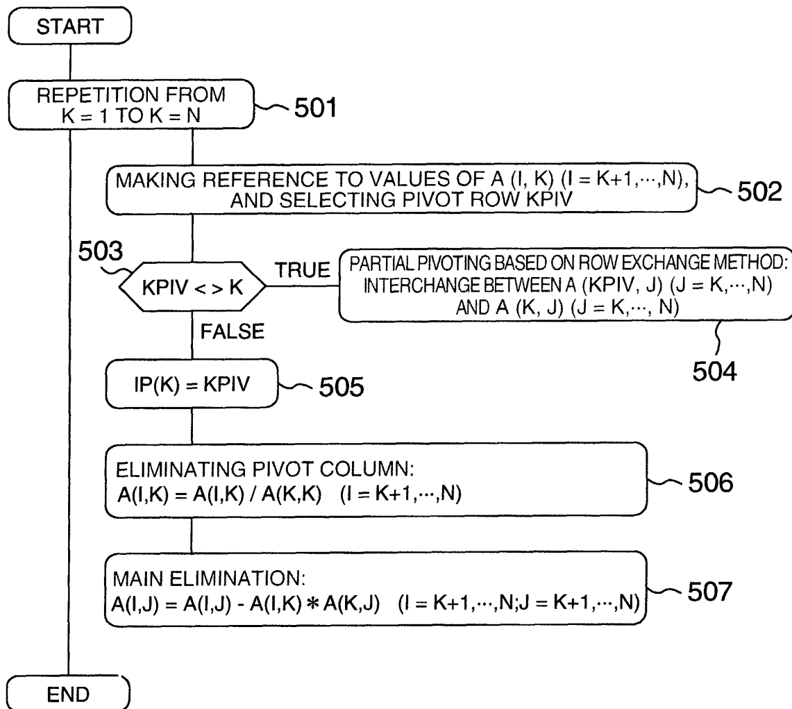
FIG.5 PRIOR ART
