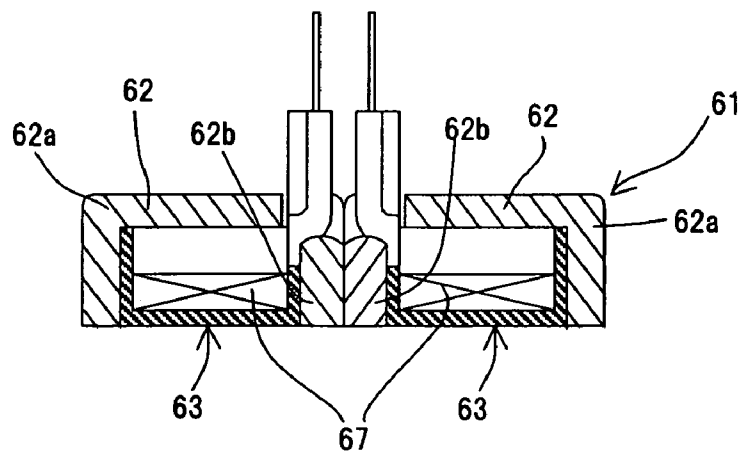
FIG.10 PRIOR ART
