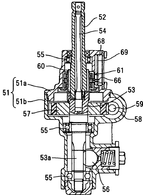
FIG.9 PRIOR ART
