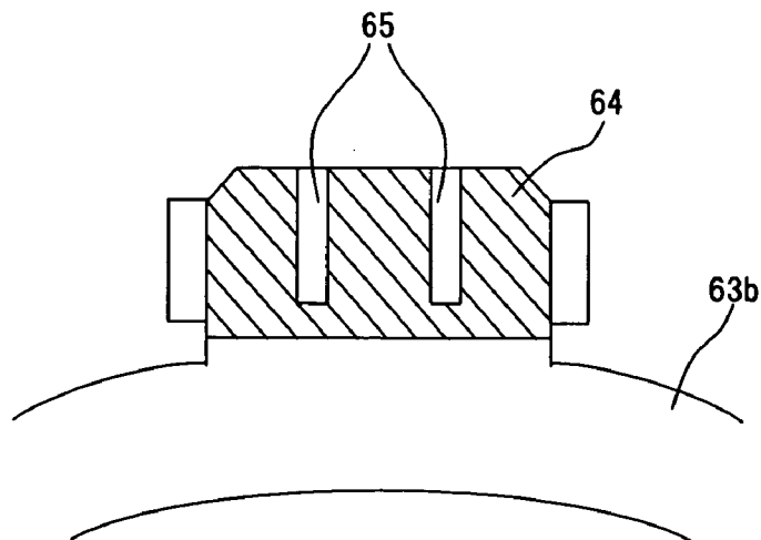
FIG.12 PRIOR ART
