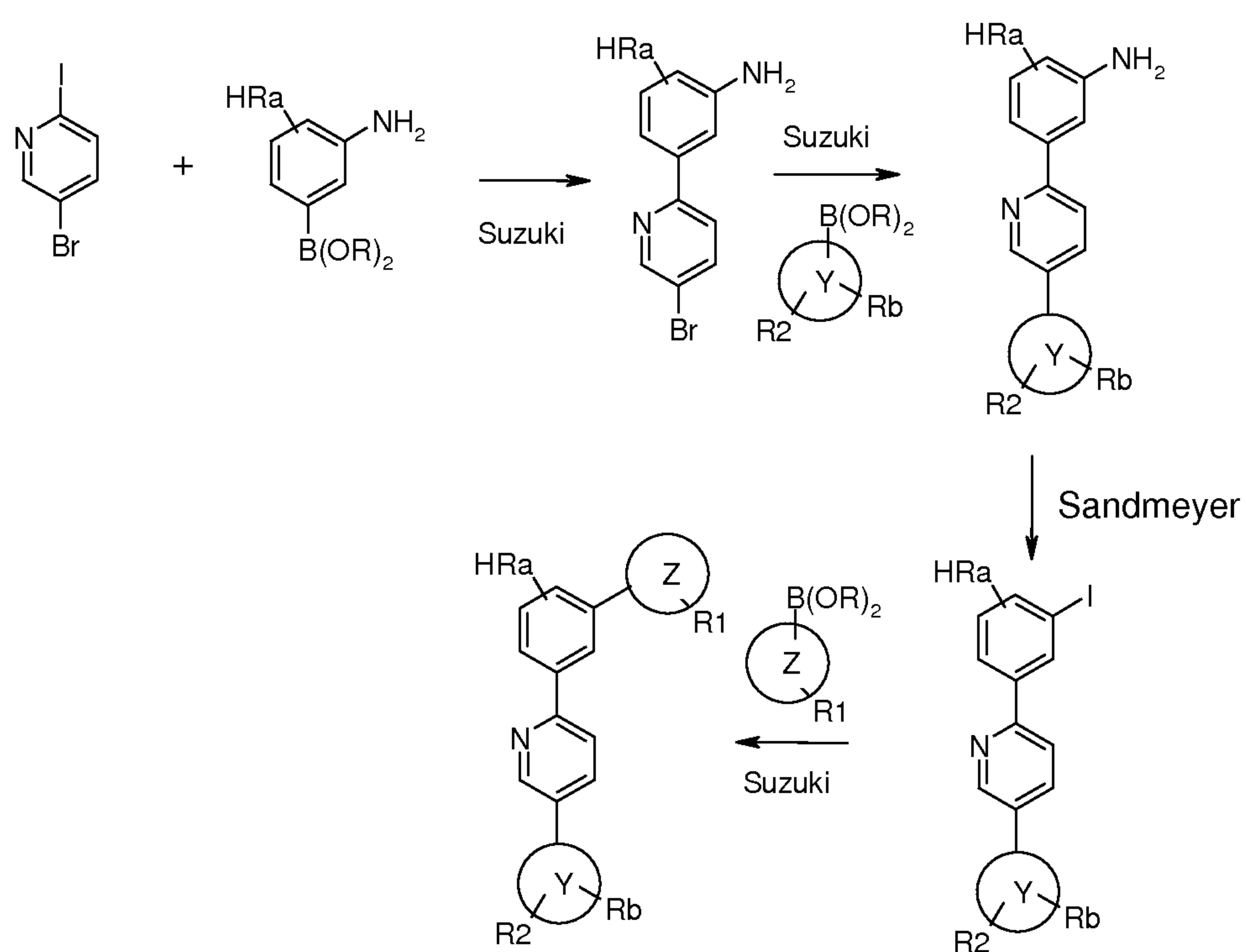
Scheme 2: Example of synthetic route for pyridinyl-pyridines
