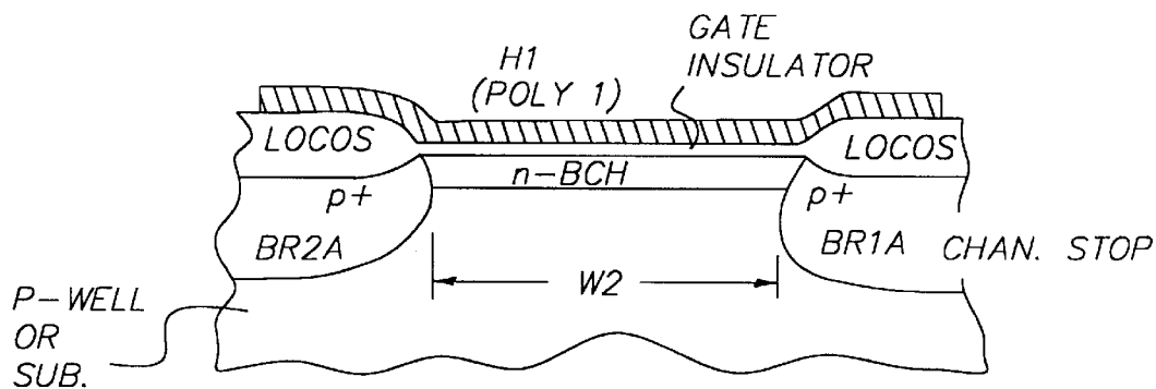
FIG. 4 (PRIOR ART)
