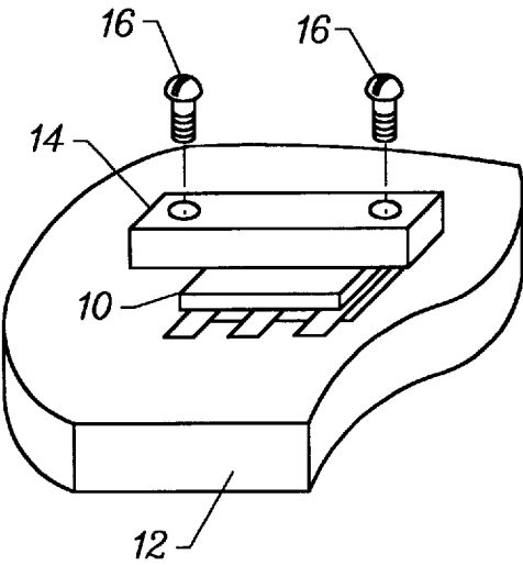
FIG. 1 PRIOR ART
