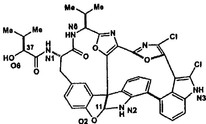
(-)-diazonamide A (revised Structure)
