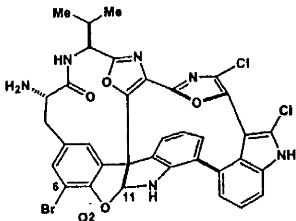
(-)-diazonamide B (revised Structure)
