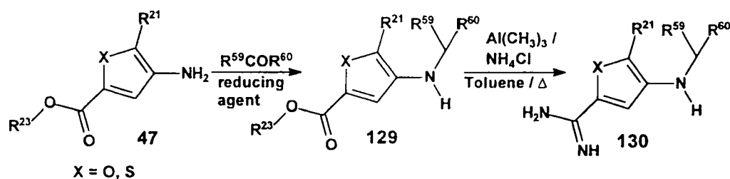
Scheme 12
