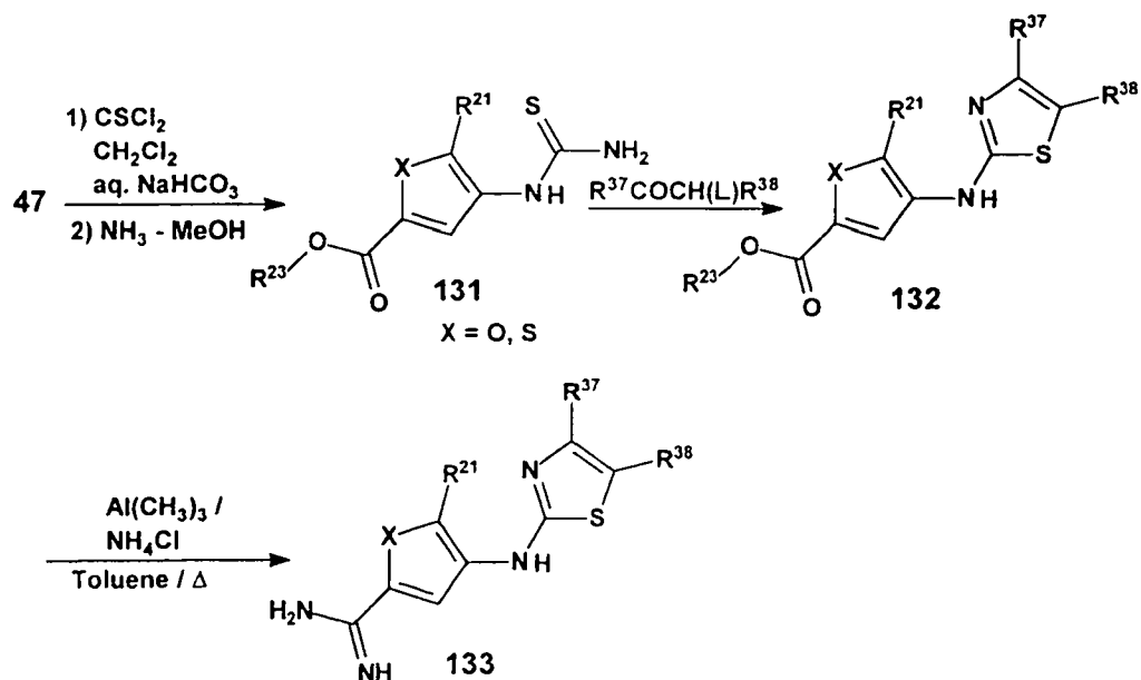
Scheme 13
