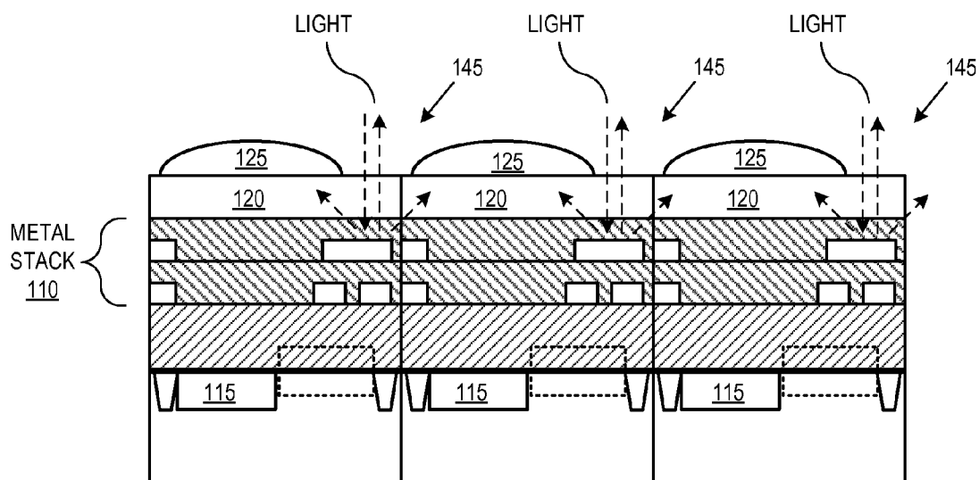
FIG. 1C (PRIOR ART)
