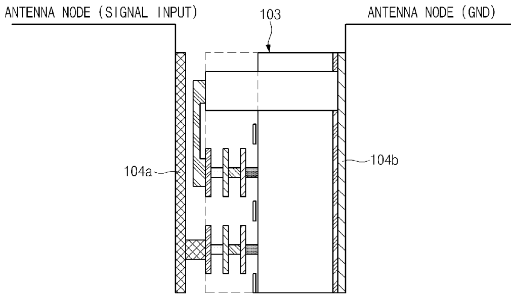
(a)CHIP-ANTENNA CONNECTION STRUCTURE METHOD
