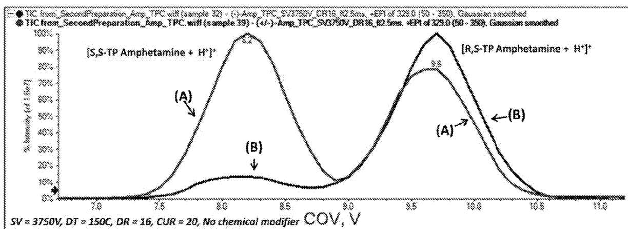
(A) Mixture of S,S- and R,S-TP Amphetamine (555 ng/mL) -- From Racemic Amphetamine (B) R,S-TP Amphetamine (555 ng/mL) -- From Pure R-Amphetamine
