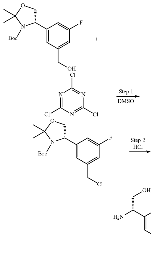
Scheme 73
