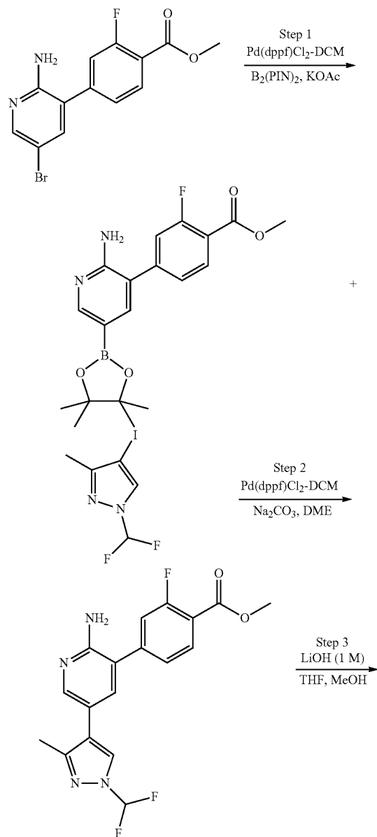
Scheme 97
