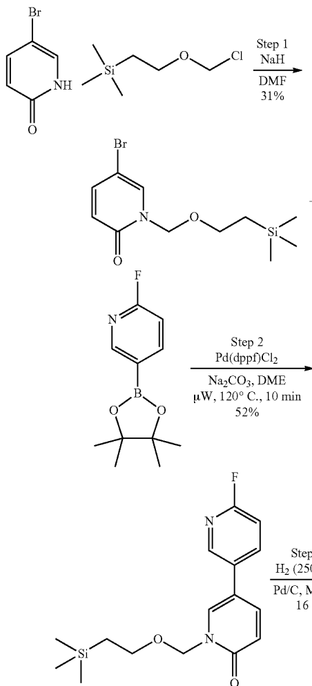
Scheme 47
