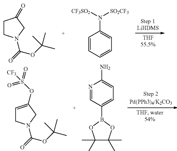
Scheme 14
