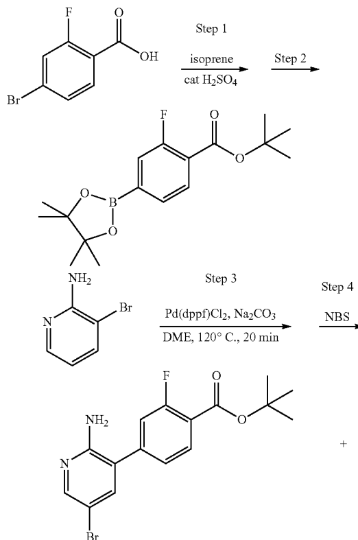
Scheme 103
