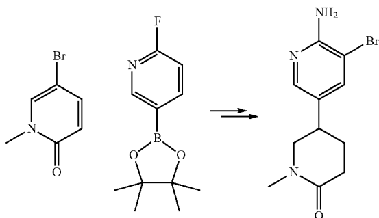
Scheme 49
