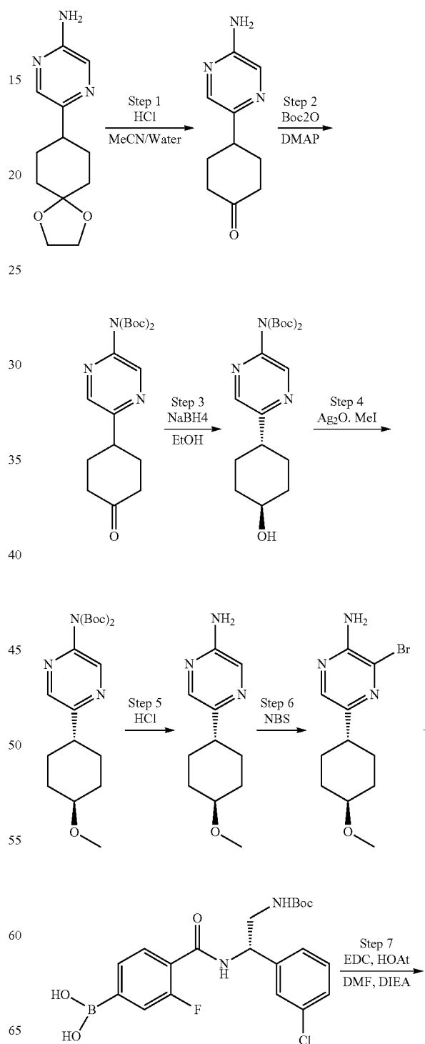
Scheme 36
