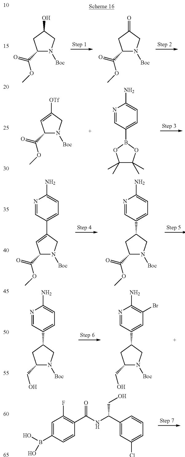
Scheme 16
