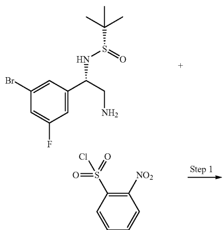
Scheme 83
