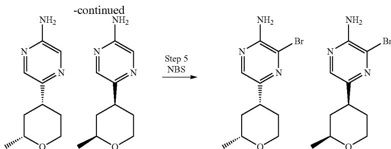
Step 4. 5-((2R,4R)-2-methyltetrahydro-2H-pyran-4-yl)pyrazin-2-amine
