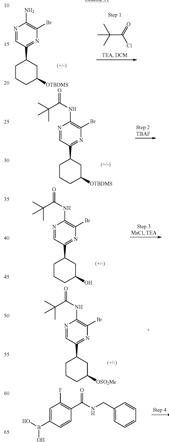
Scheme 31
