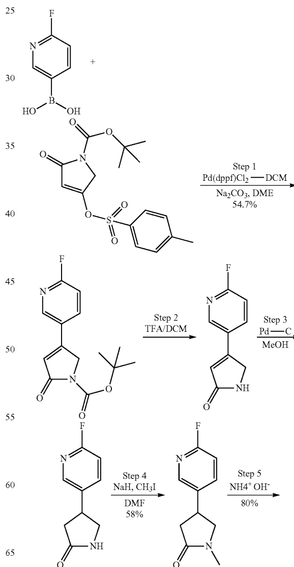
Scheme 50
