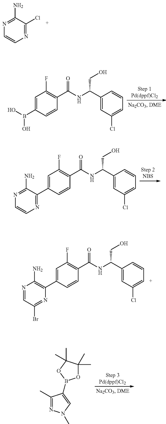
Scheme 53
