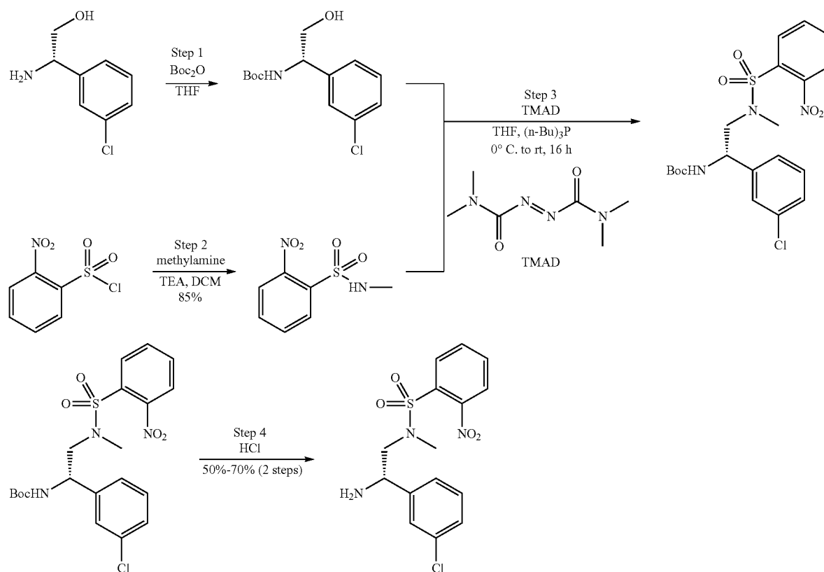
Scheme 65
