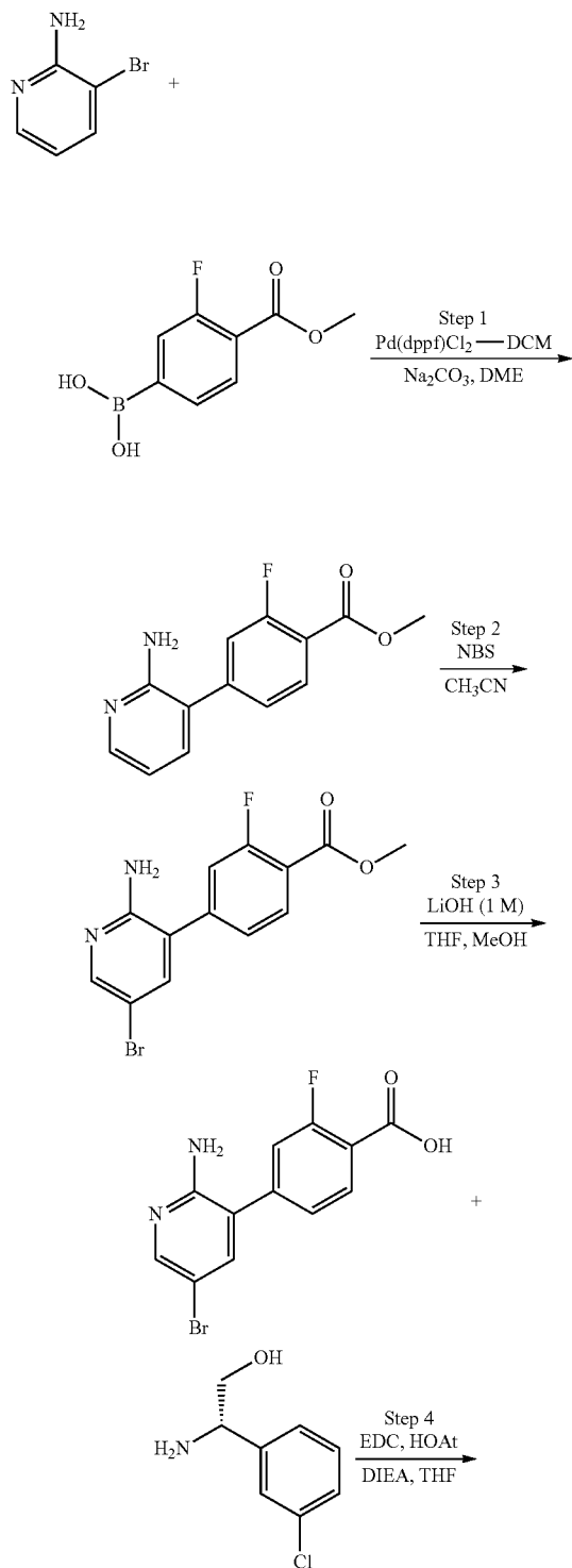
Scheme 54
