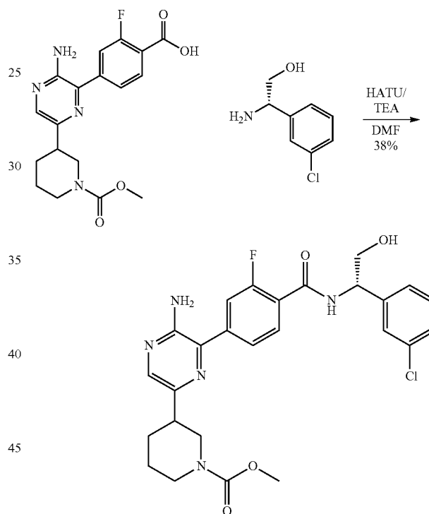
Scheme 107
