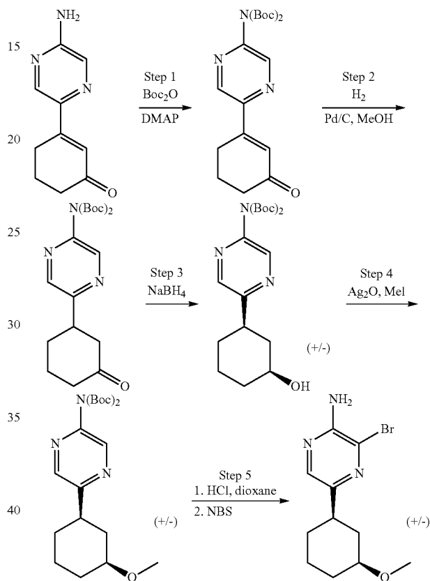
Scheme 30
