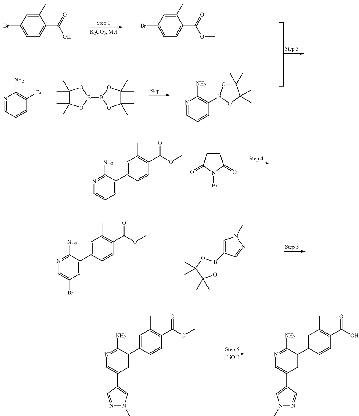
Scheme 102
