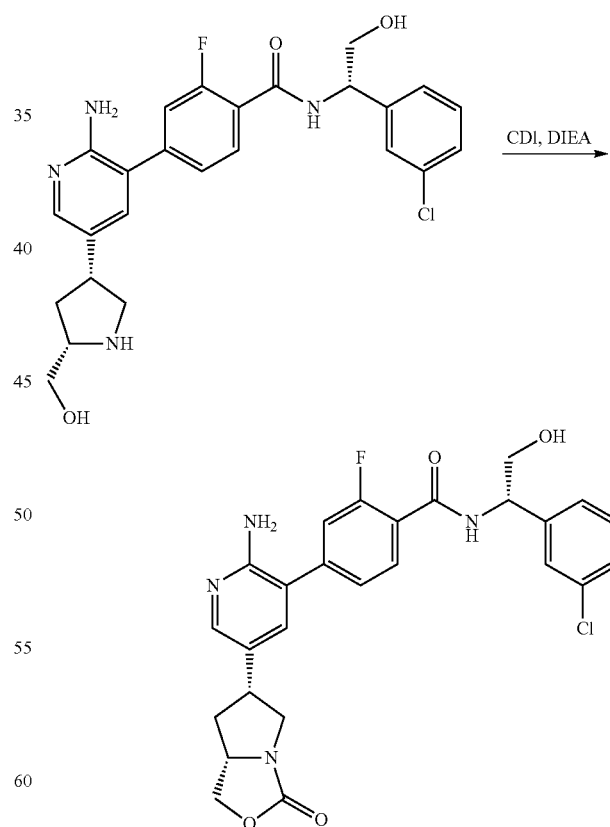
Scheme 18
