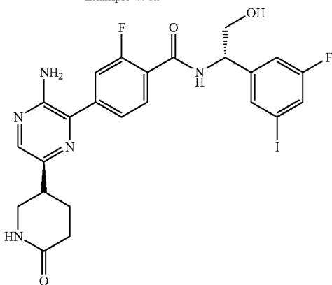
Example 478b
