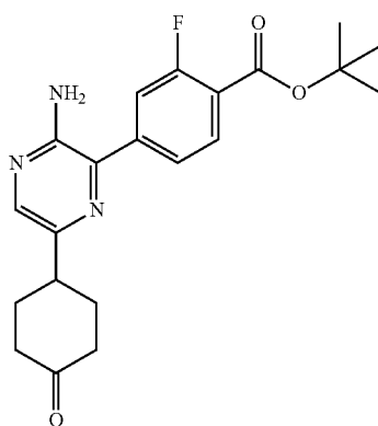
Scheme 84
