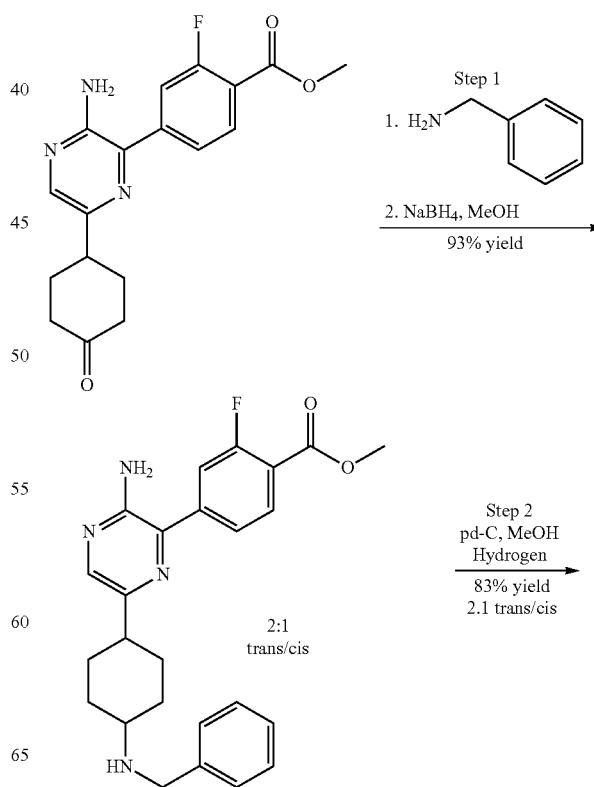
Scheme 90
