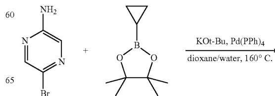
Scheme 23
