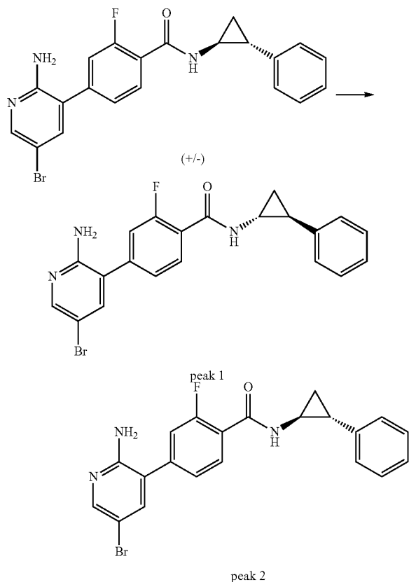
Scheme 57
