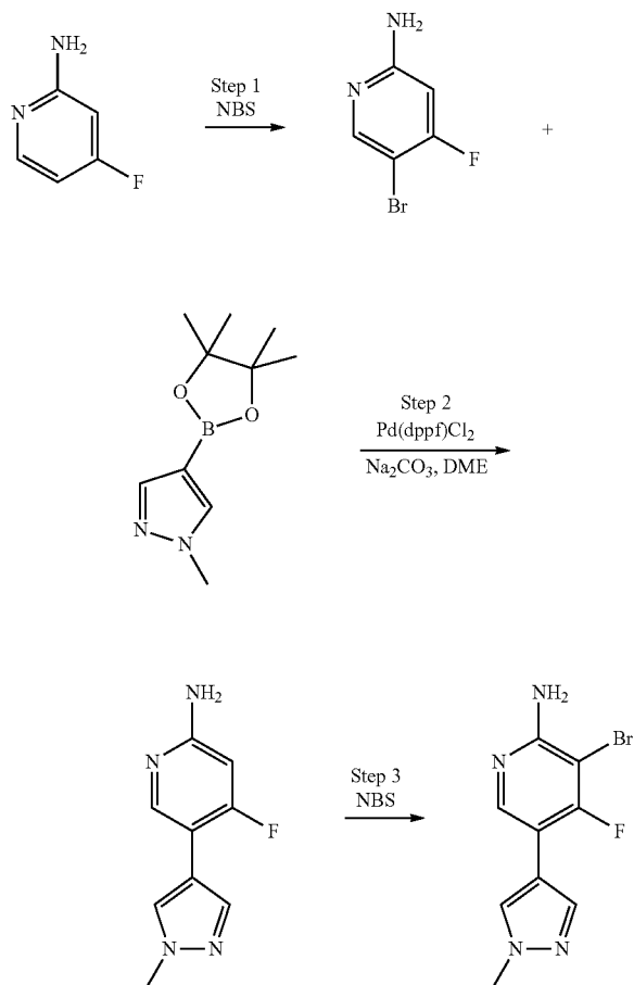
Scheme 27
