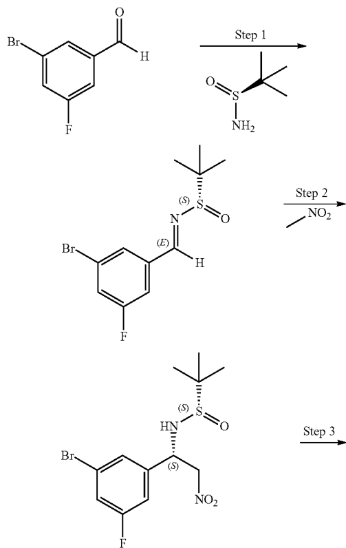
Scheme 78
