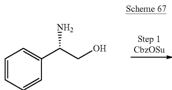
Scheme 67
