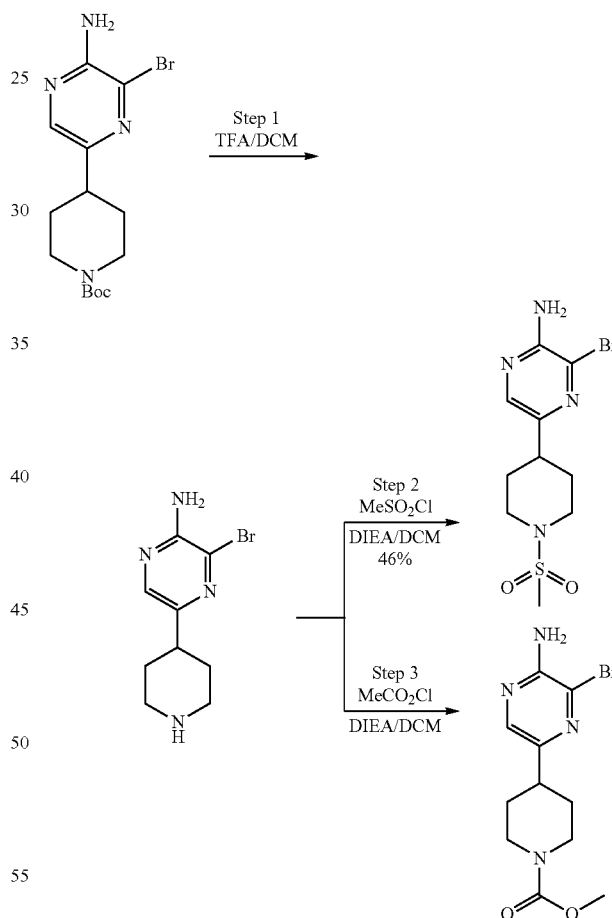
Scheme 11
