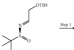
Scheme 71
