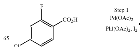
Scheme 95
