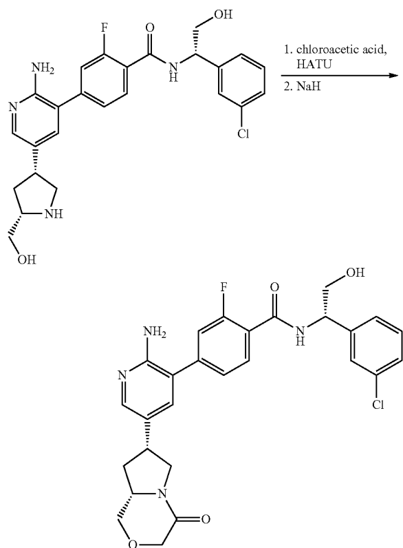
Scheme 17
