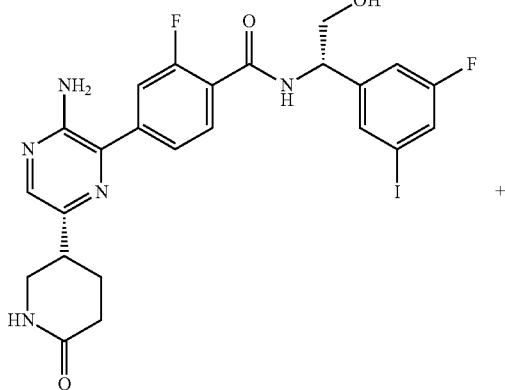
Example 478a
