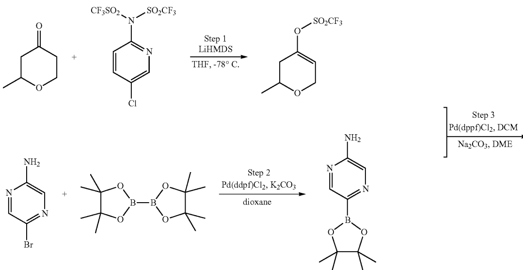
Scheme 22
