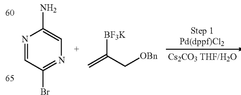
Scheme 44
