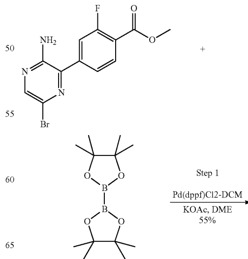
Scheme 113
