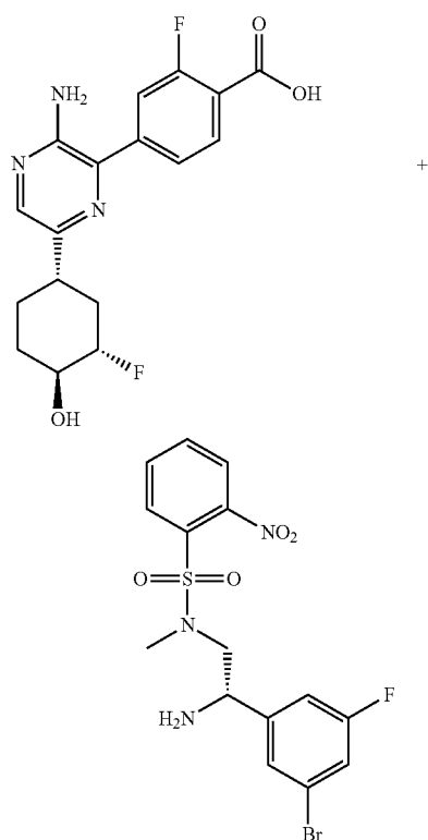
Scheme 86
