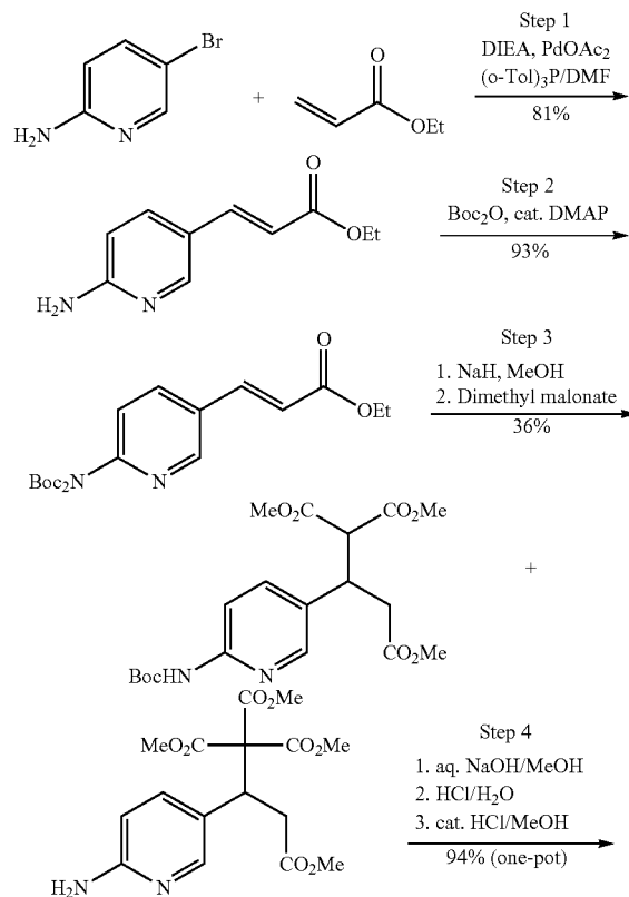
Scheme 96
