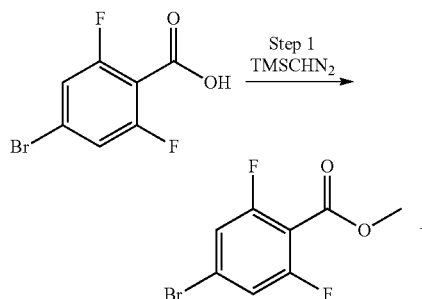
Scheme 56
