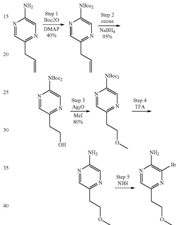
Scheme 40
