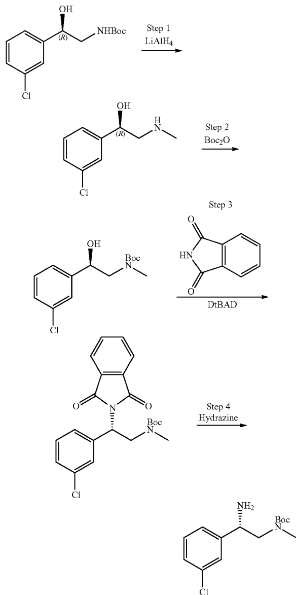
Scheme 70
