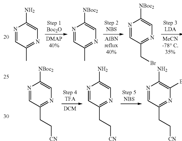
Scheme 45
