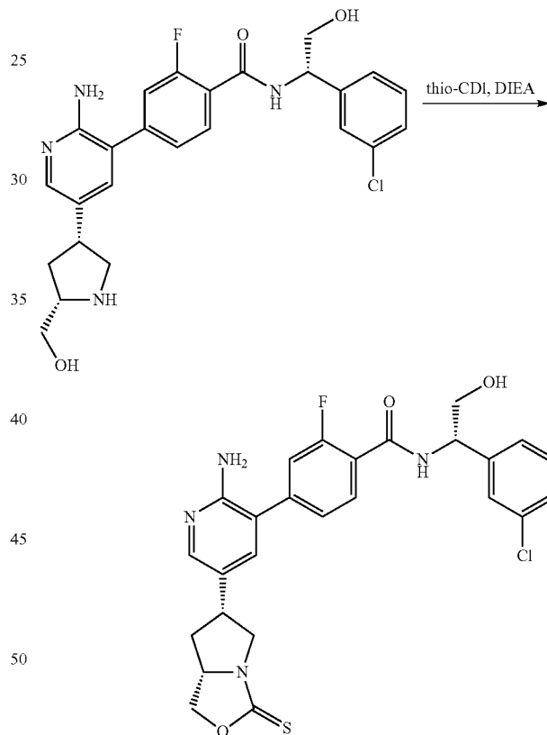
Scheme 20
