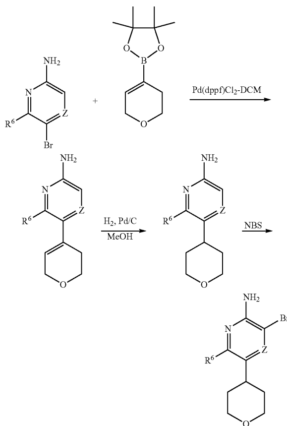
Scheme C.
