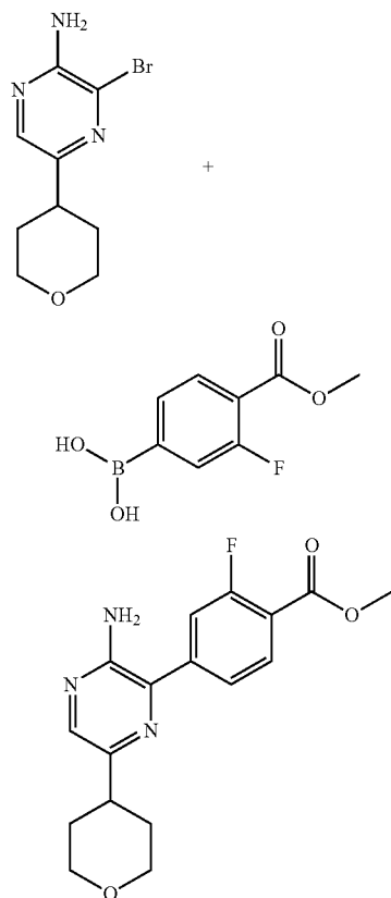
Scheme 62
