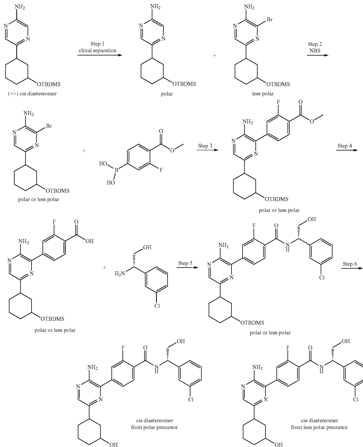
Scheme 92
