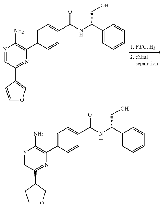
Scheme 61
