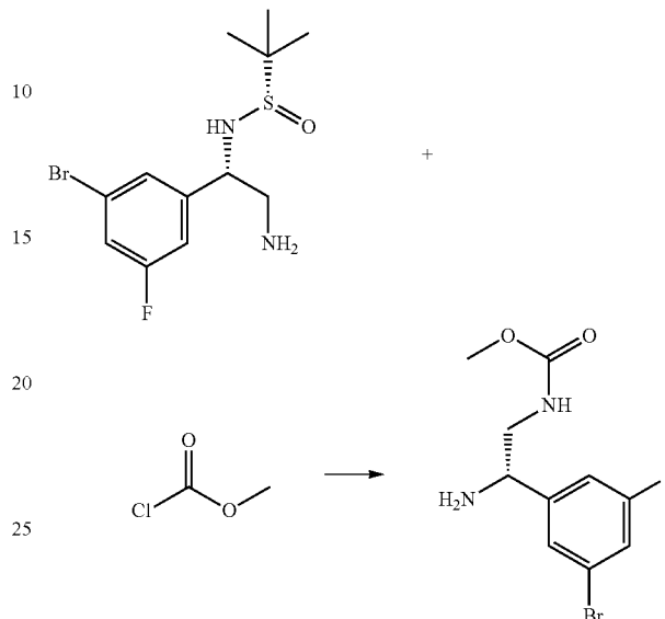
Scheme 79
