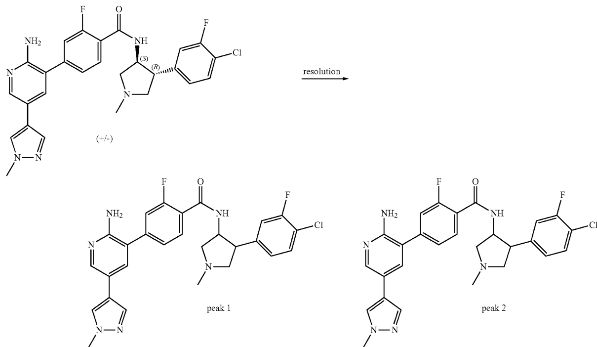
Scheme 99
