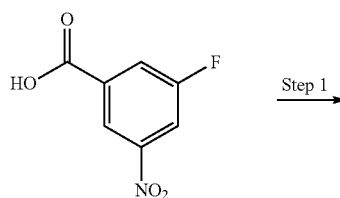
Scheme 76
