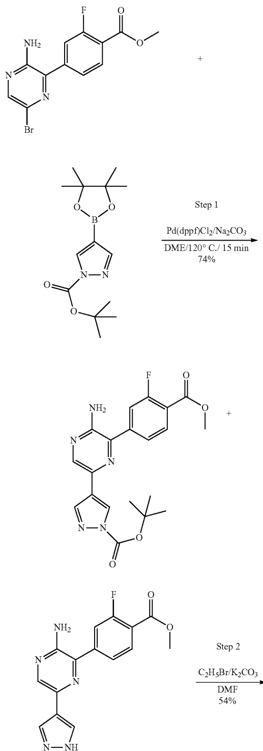
Scheme 108
