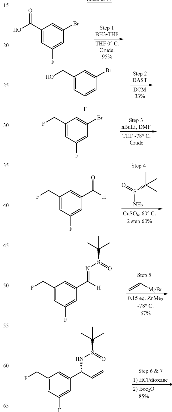
Scheme 74
