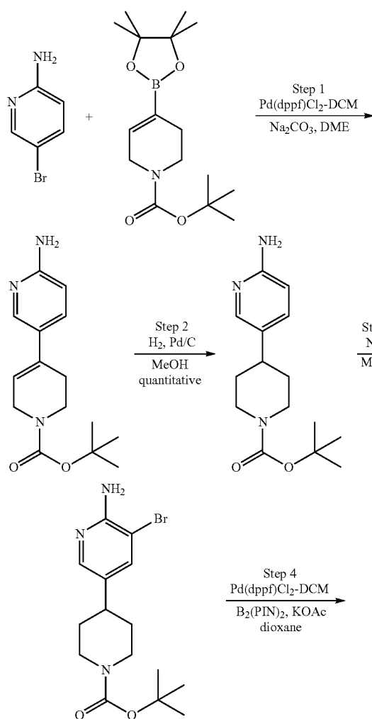
Scheme 10
