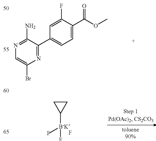
Scheme 100
