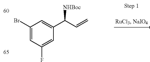
Scheme 117
