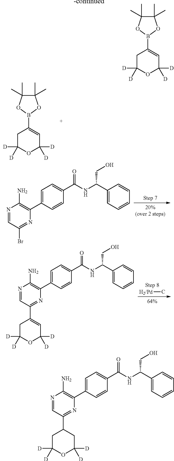
Step 1. diethyl 2,2'-(1,3-dioxolane-2,2-diyl)diacetate
