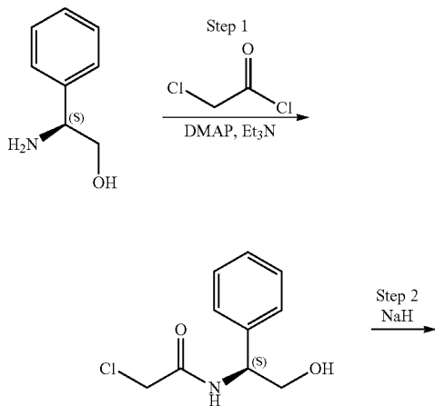
Scheme 69
