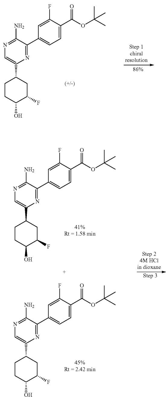
Scheme 87
