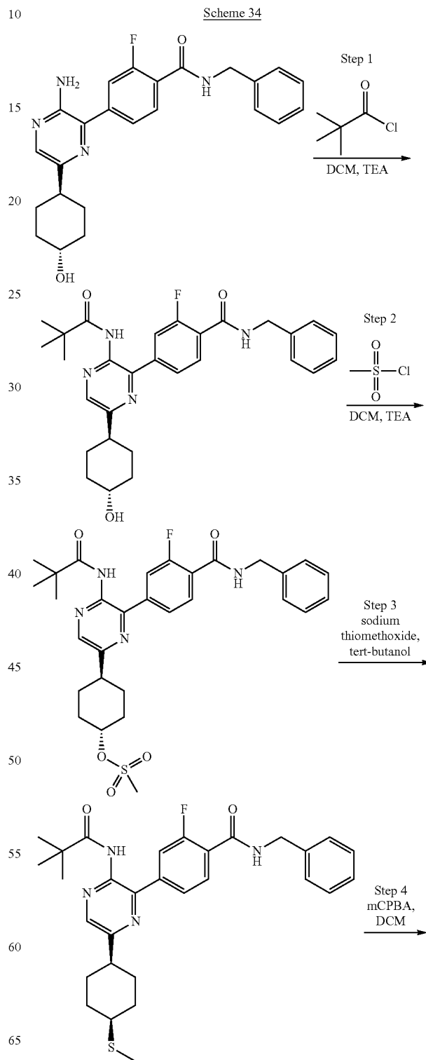
Scheme 34
