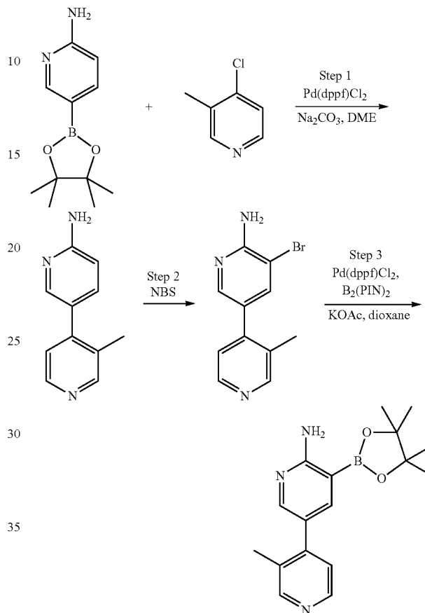
Scheme 24
