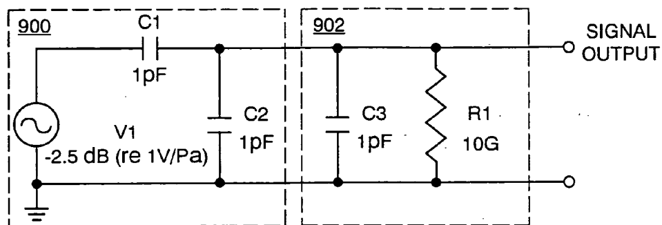
FIG. 25 (PRIOR ART)
