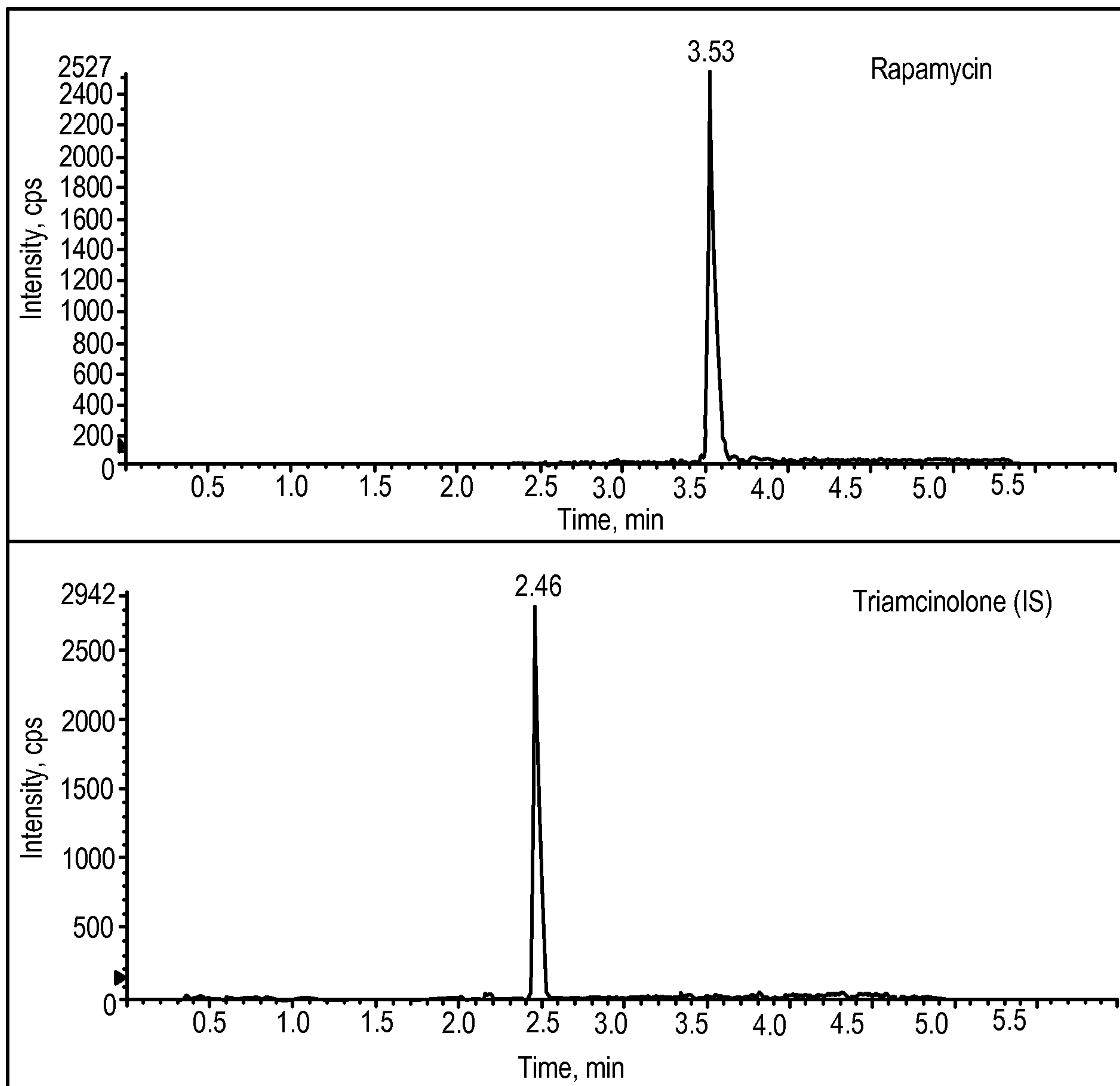
LC-MS/MS Chromatogram of 10.6 ng/mL Rapamycin (top) and Internal Standard (bottom) in Mouse Blood
