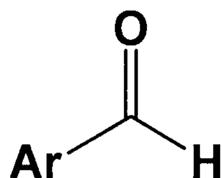
Formula III
