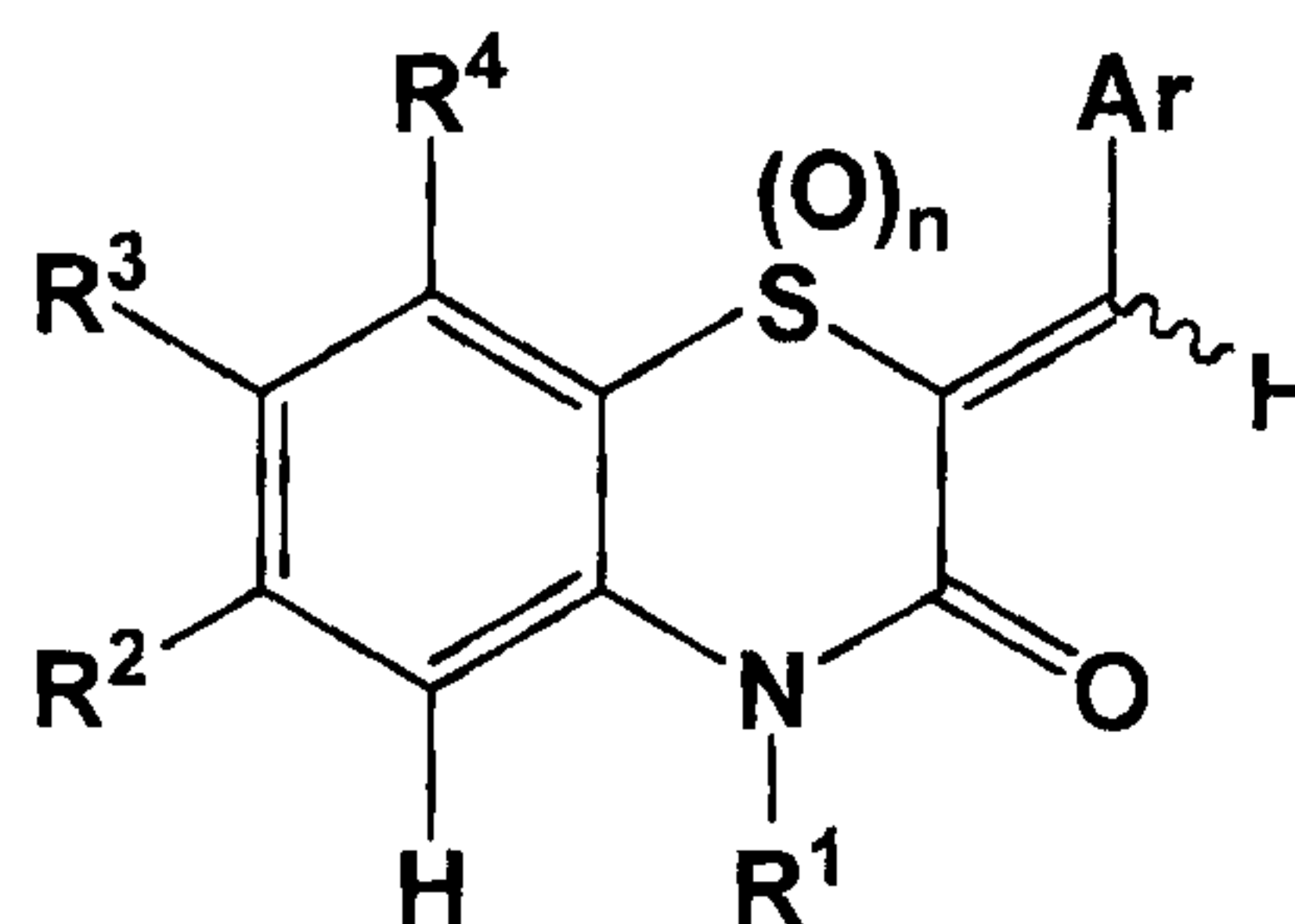
Formula I
