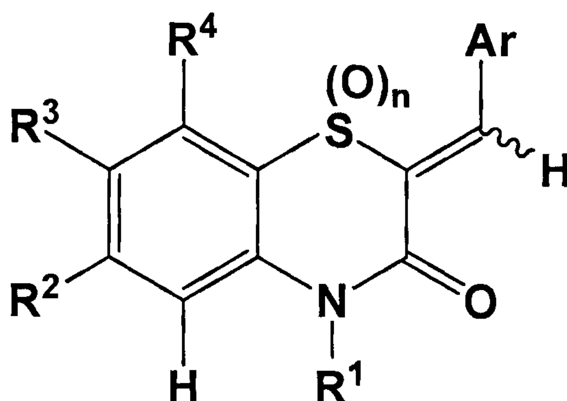
Formula I
