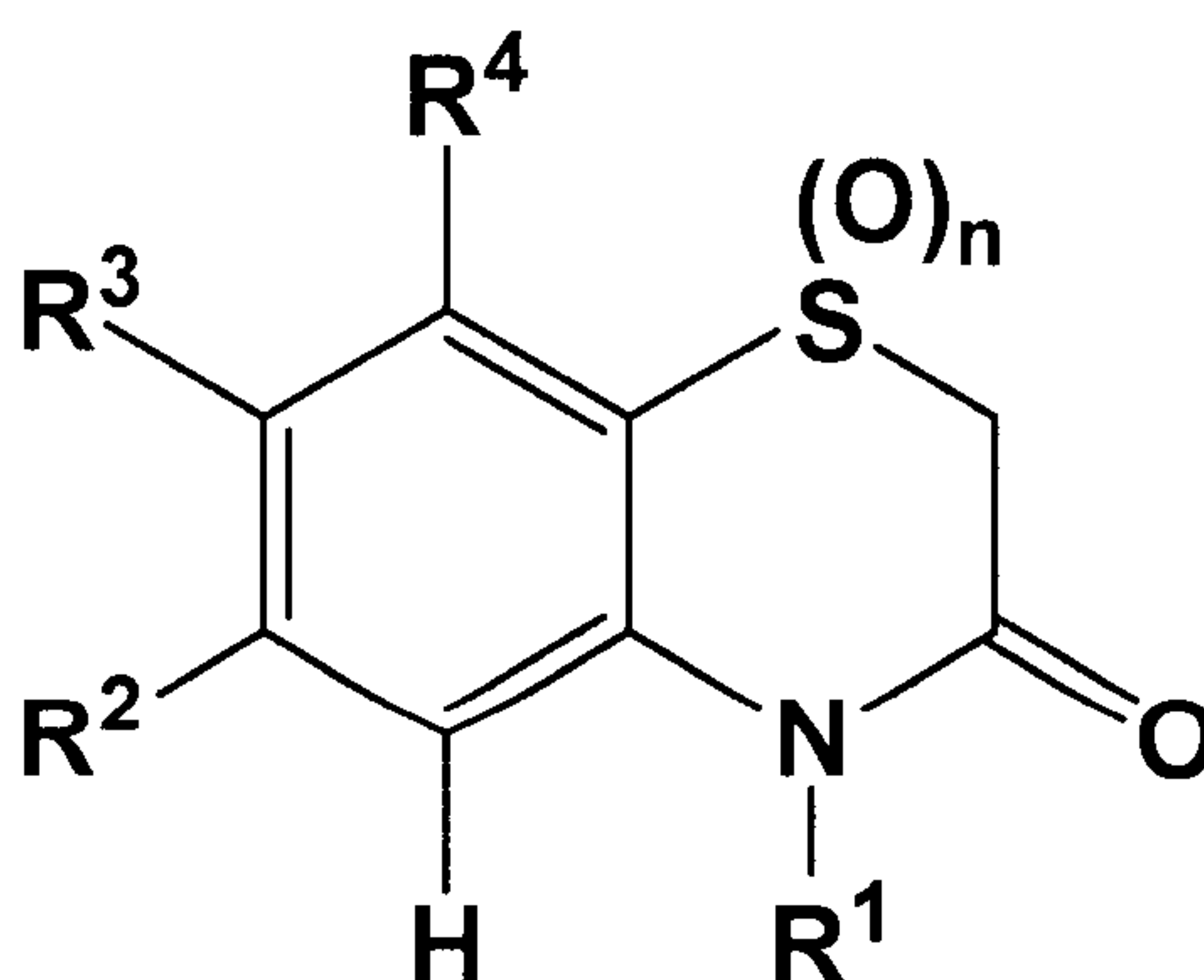
Formula IV
