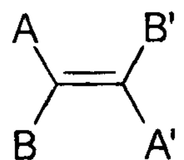
( E ) isomer
