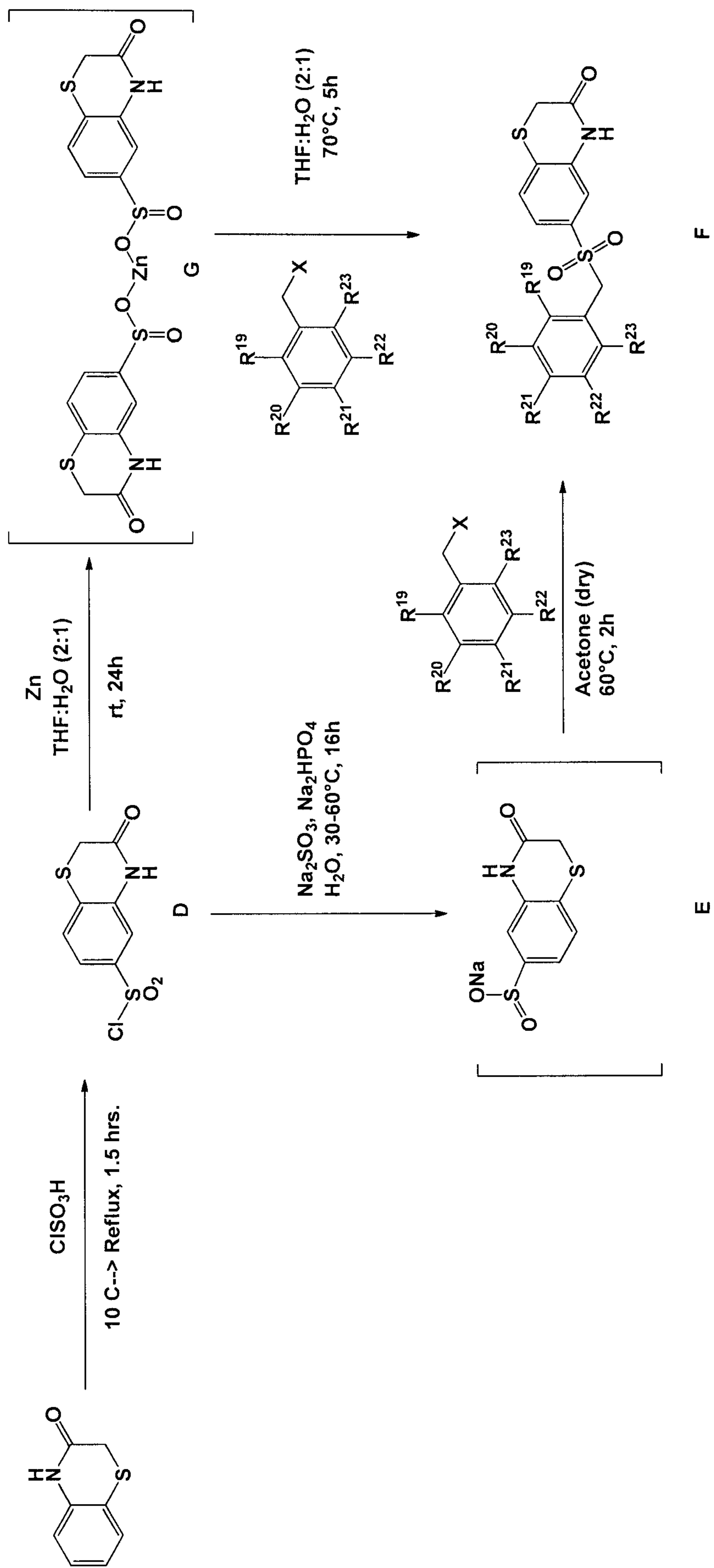
Scheme 2
