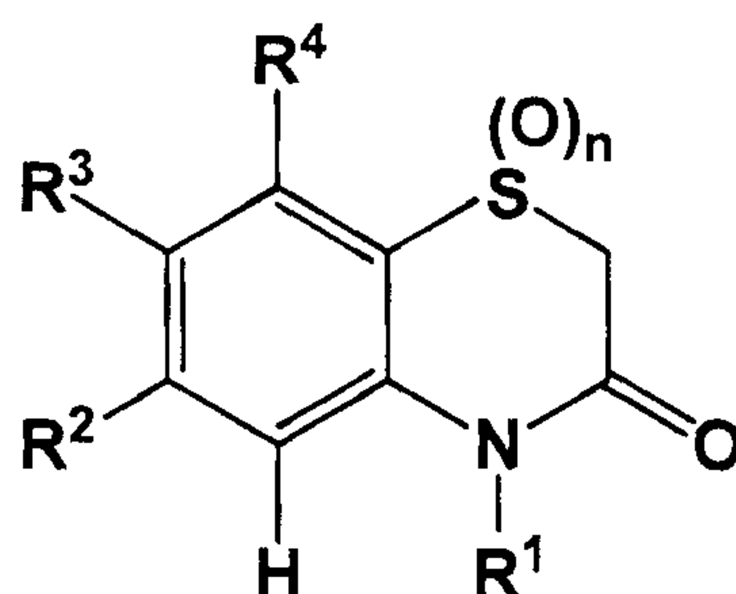
Formula IV
