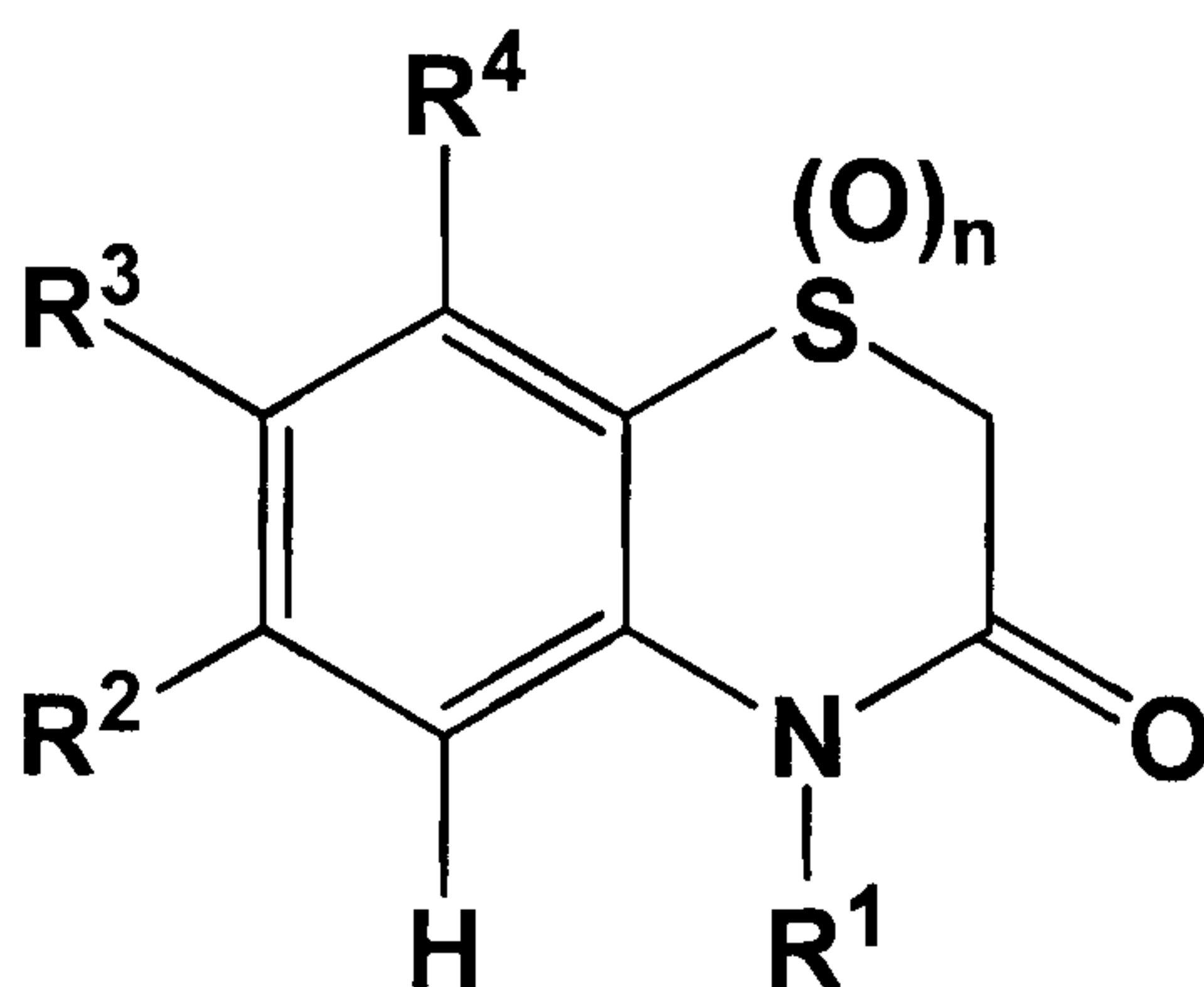
Formula IV
