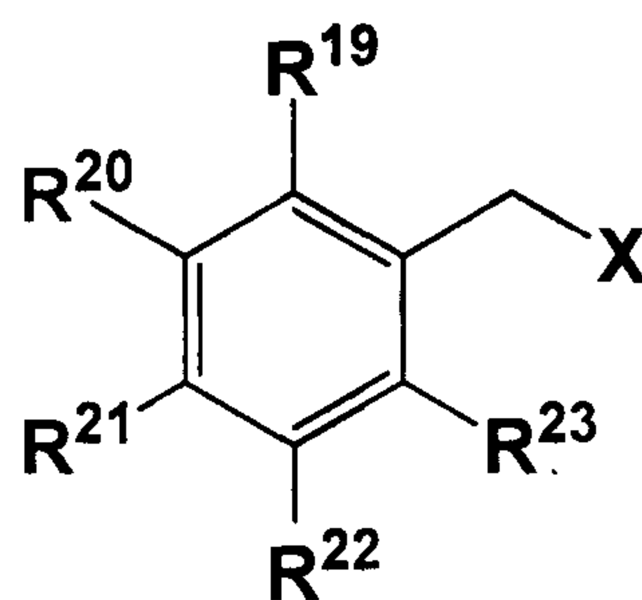
Formula V
