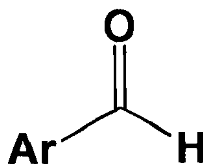
Formula III
