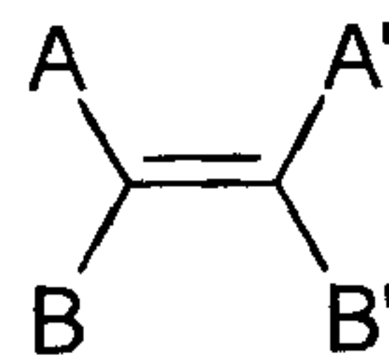
( Z ) isomer
