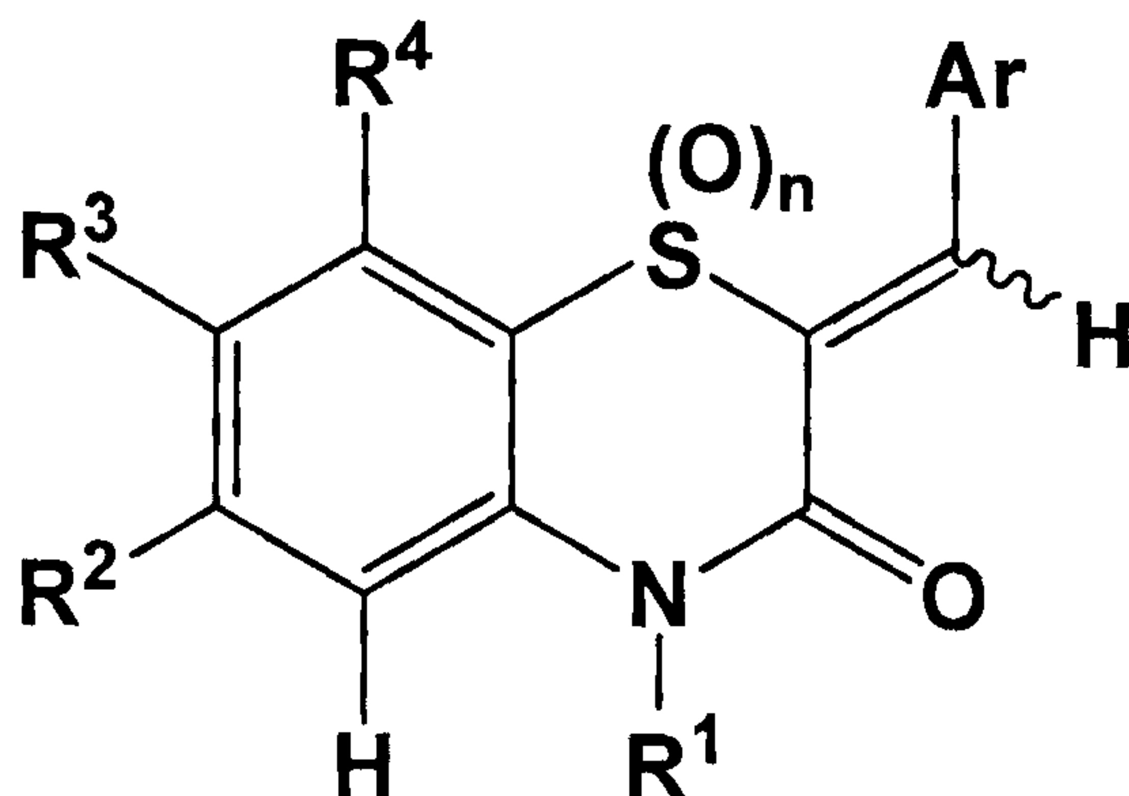
Formula I
