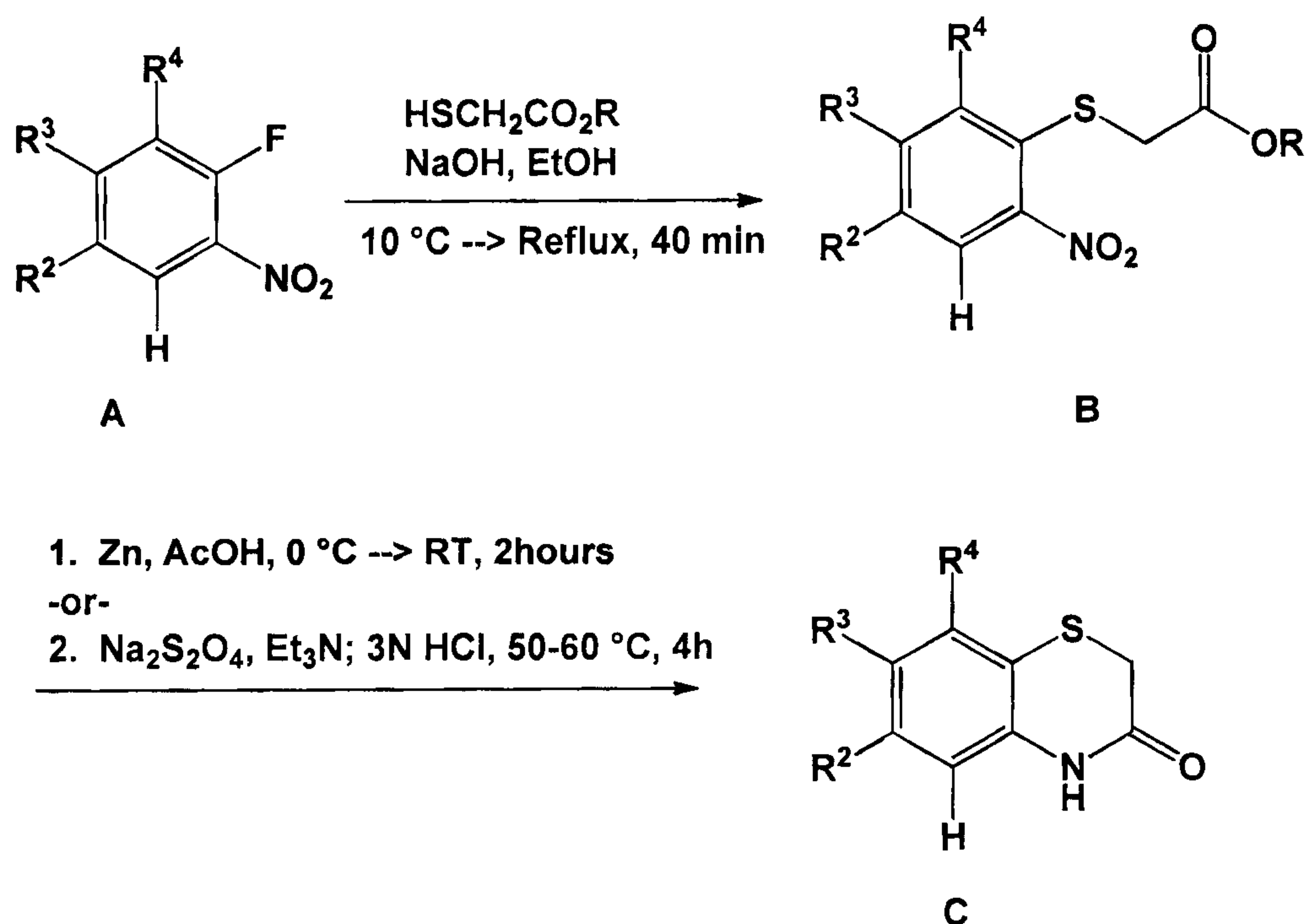
Scheme 1
