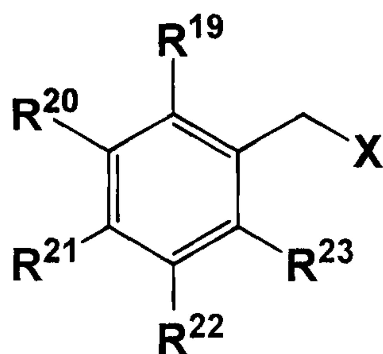
Formula V
