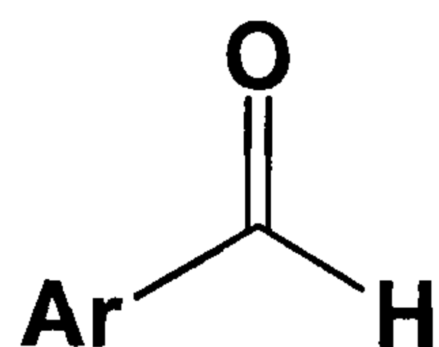
Formula III
