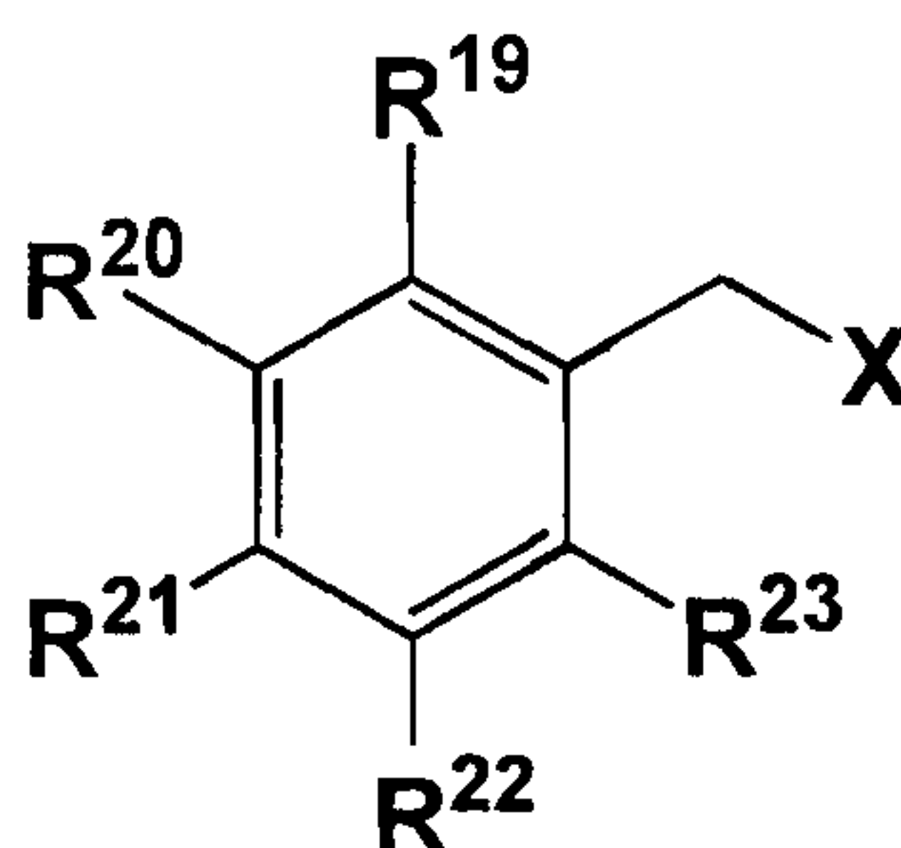
Formula V
