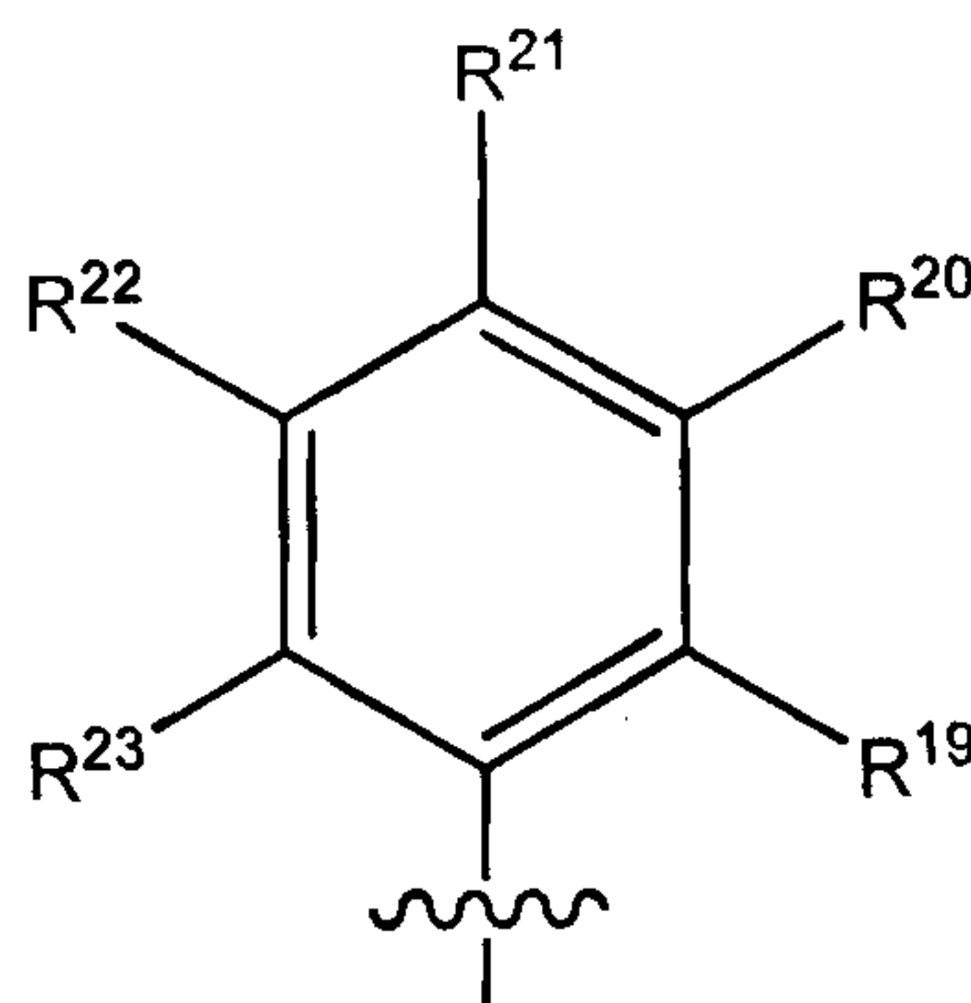
Formula II
