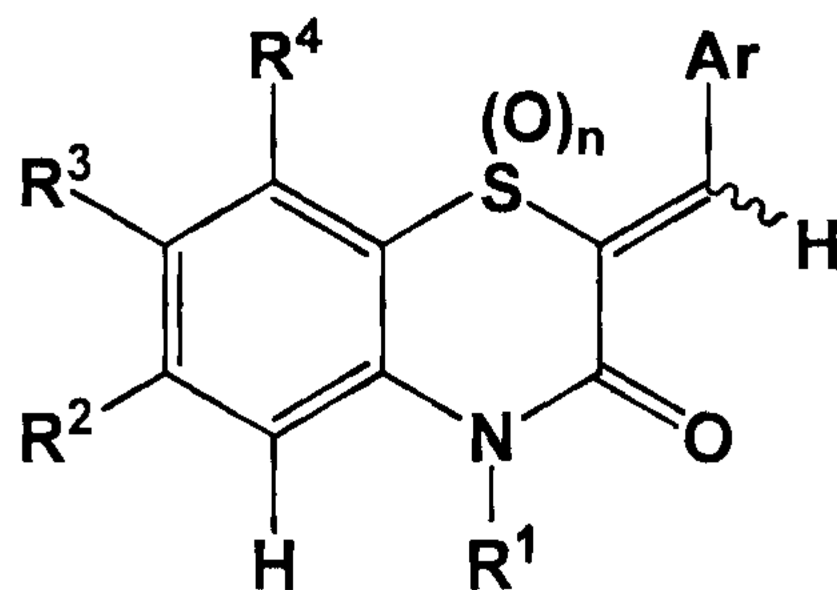
Formula I
