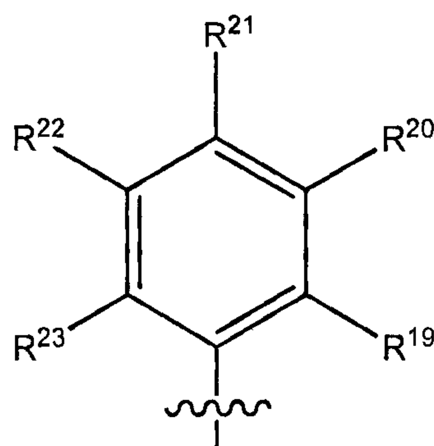
Formula II
