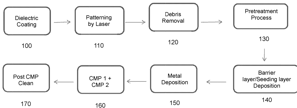
FIG. 1: Conventional Process
