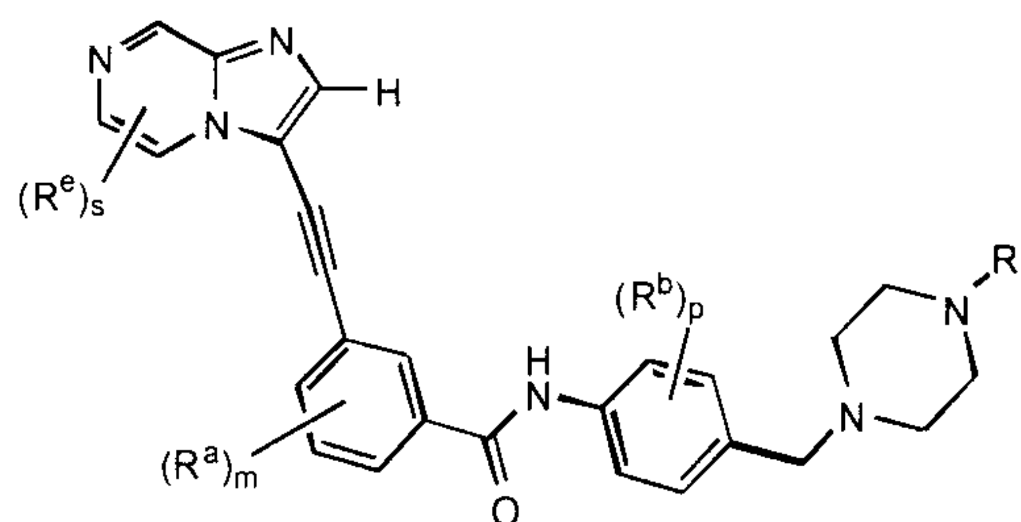
Formula IIIa
