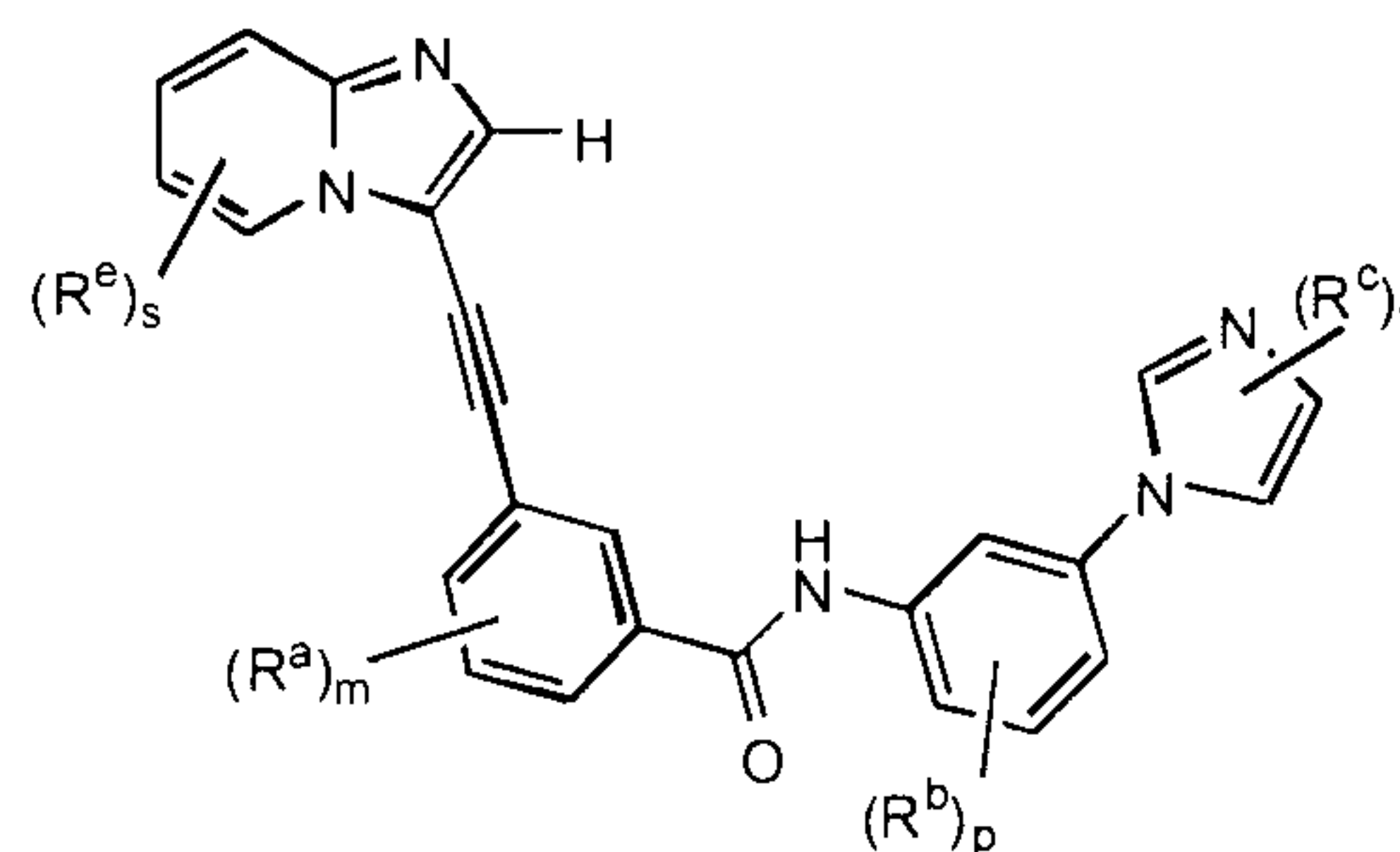
Formula IIb
