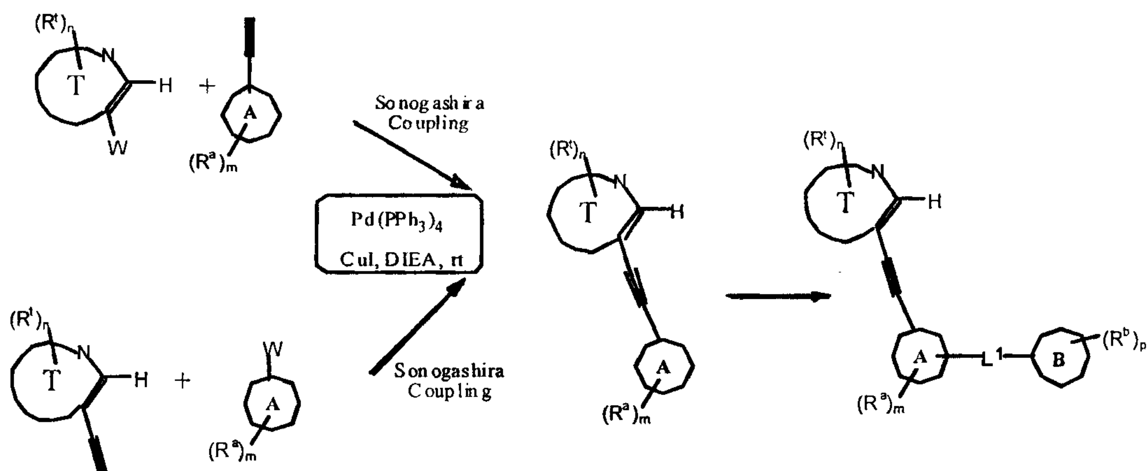
Scheme XVI
