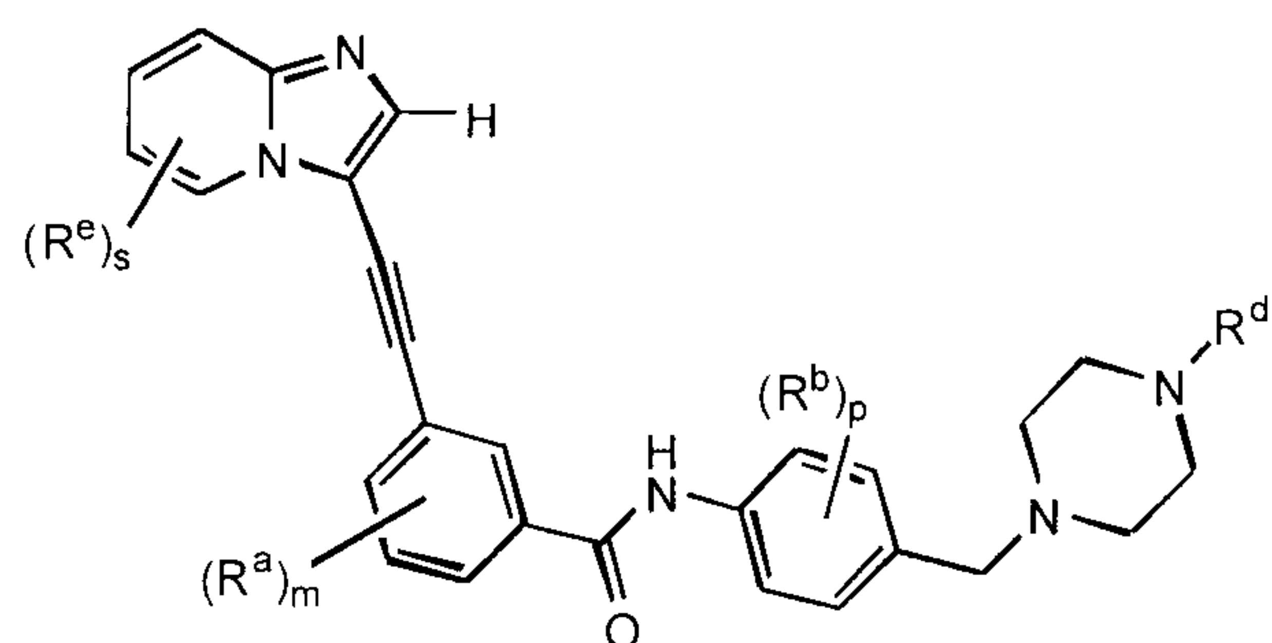
Formula IIIb
