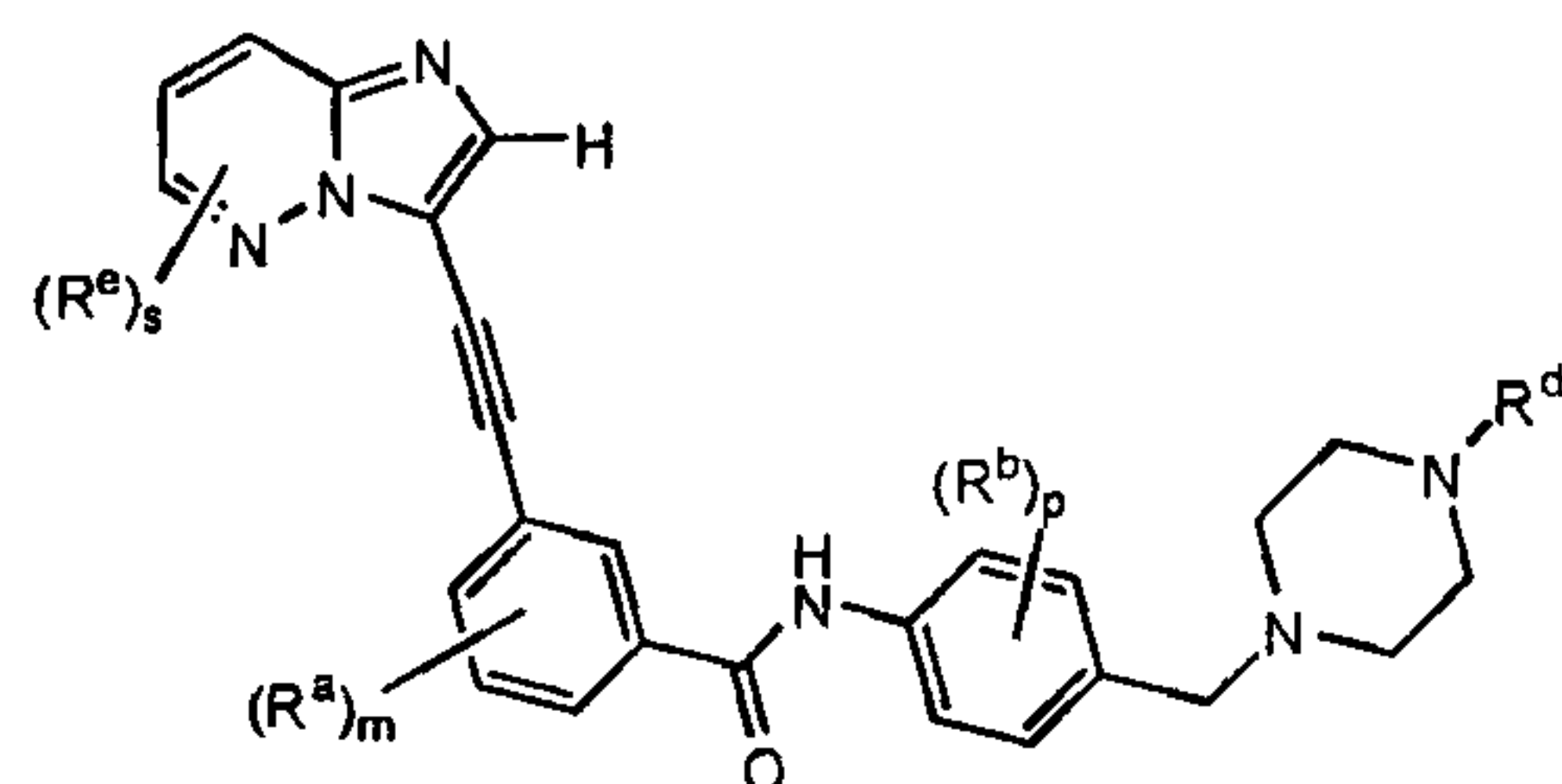
Formula IIIc
