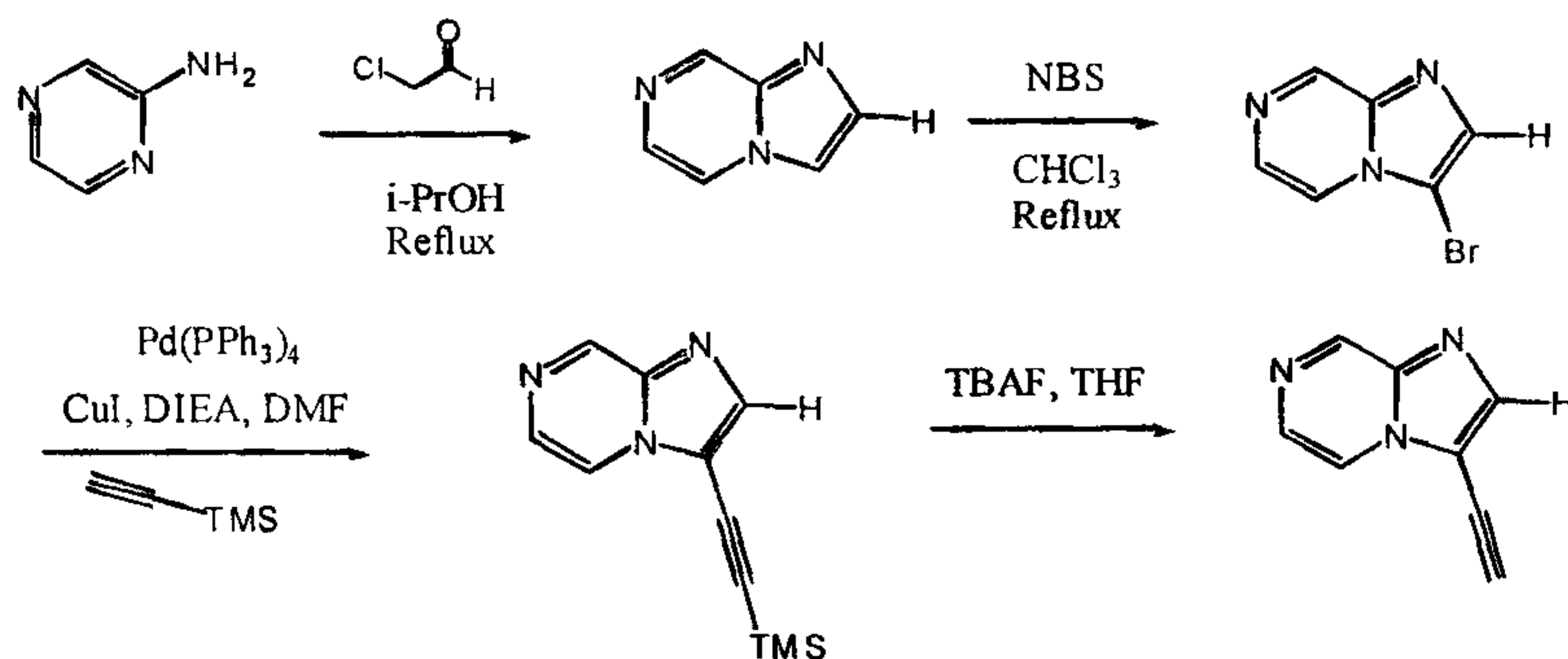
Scheme III: Preparation of 3-Ethynylimidazo[1,2-a]pyrazine
