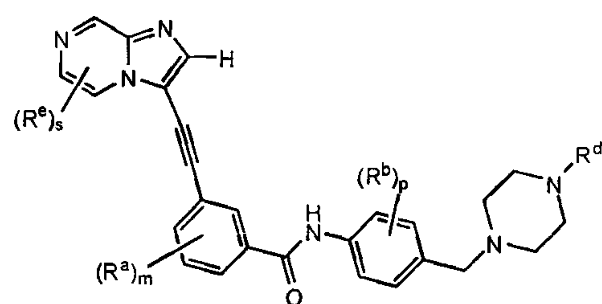
Formula IIIa
