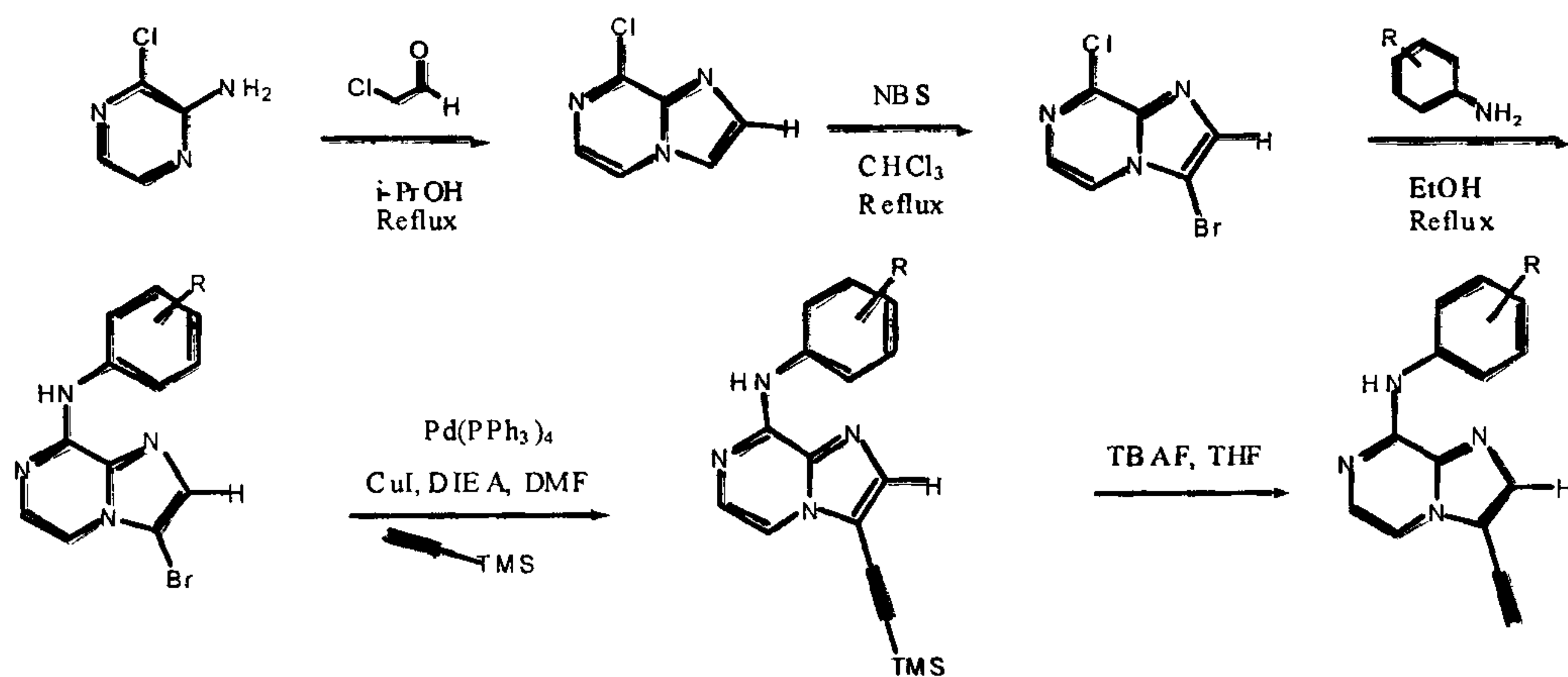
Scheme IV: Preparation of C-8 Substituted 3-Ethynylimidazo[1,2-a]pyrazines
