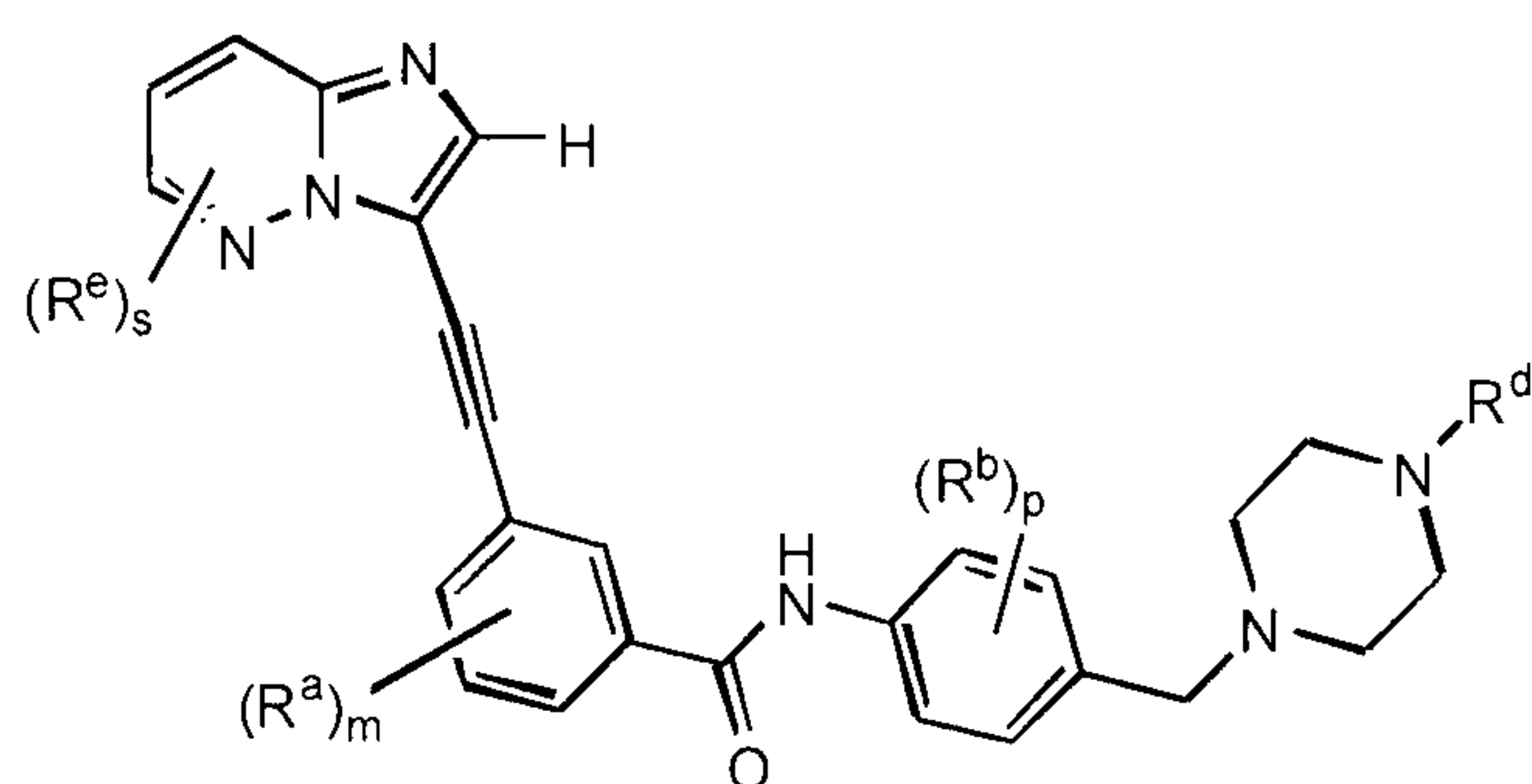
Formula IIIc.
