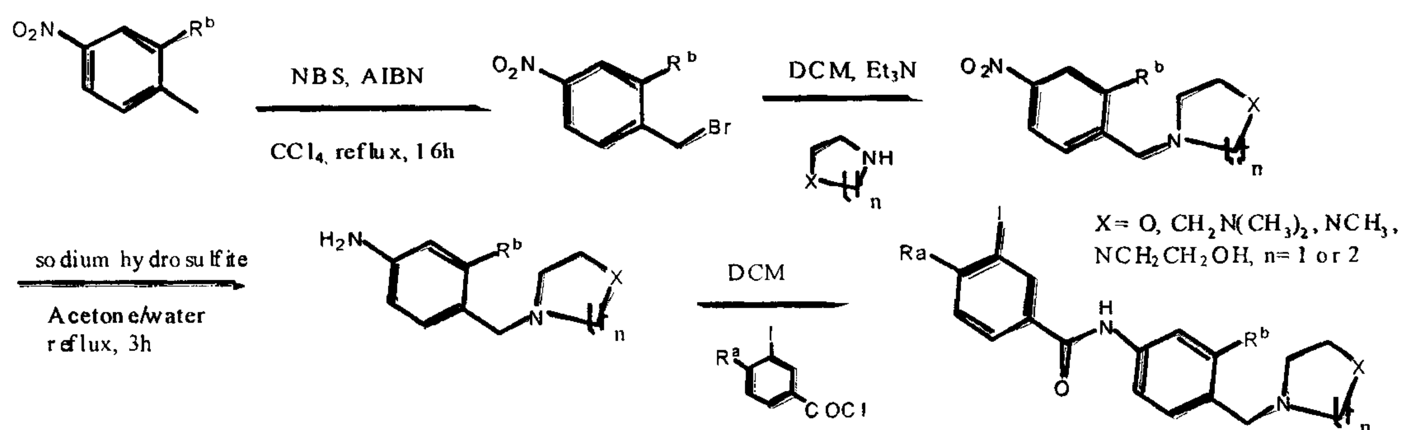
Scheme XIII
