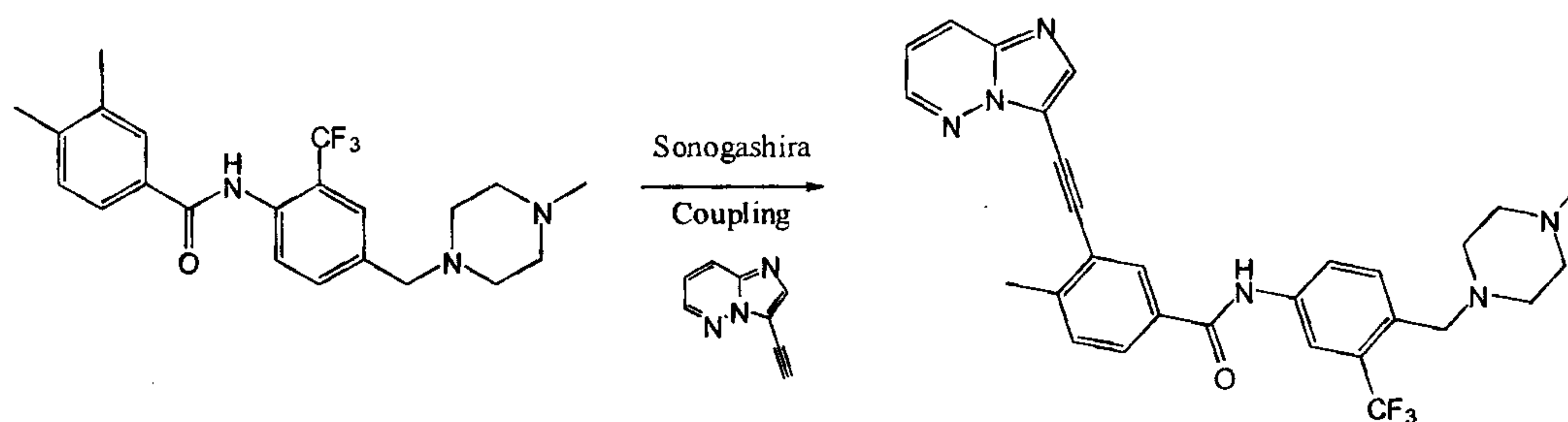
Scheme XIV
