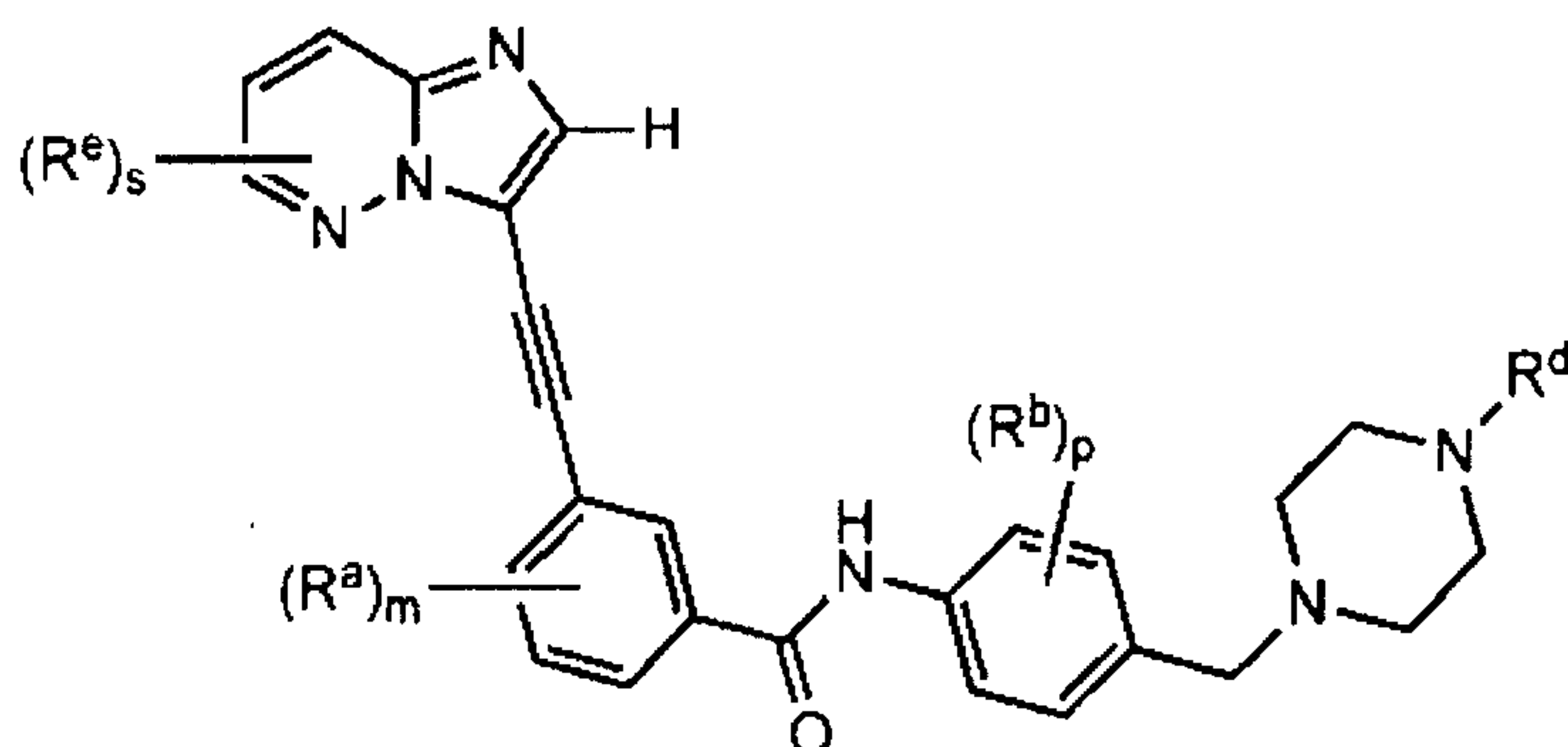
Formula IIIc
