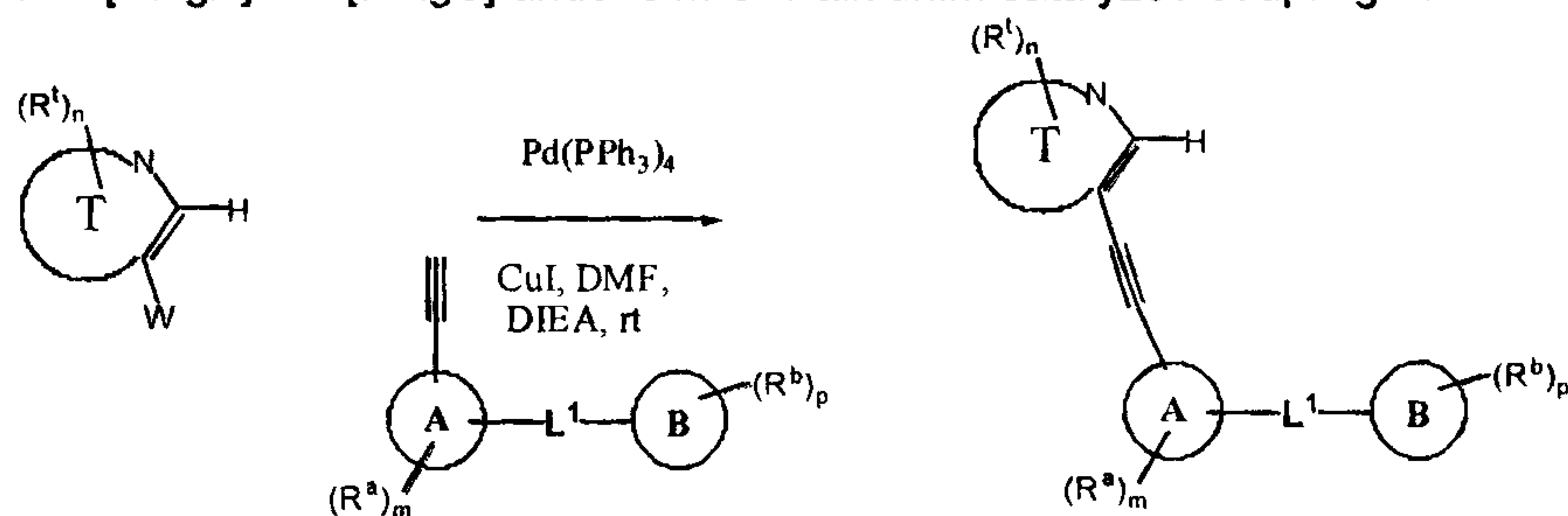
Scheme II: Alternative Sonogashira Coupling Reaction
