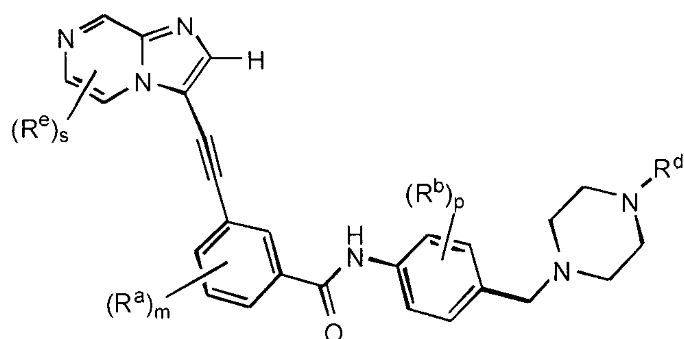
Formula IIIa
