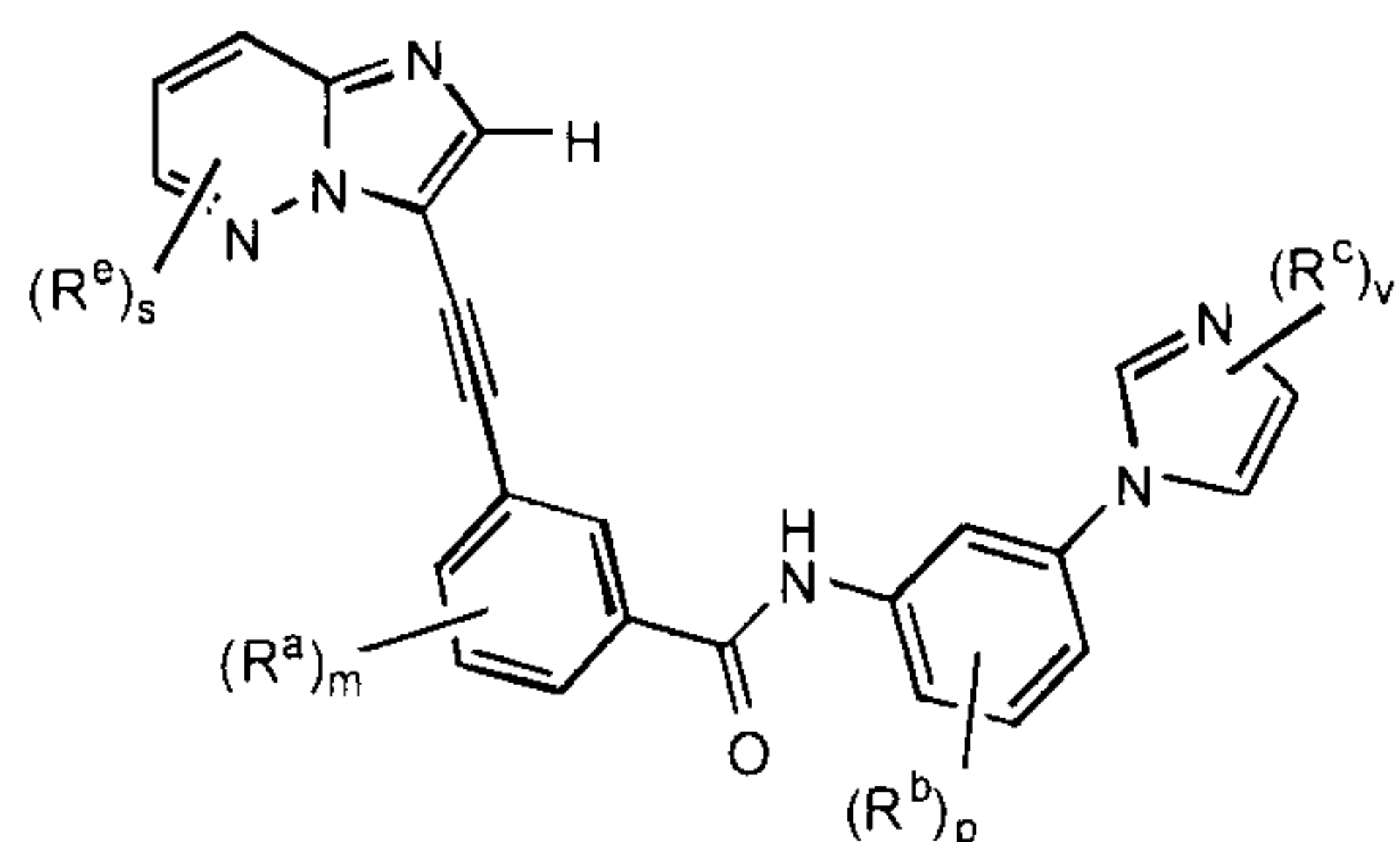
Formula IIc
