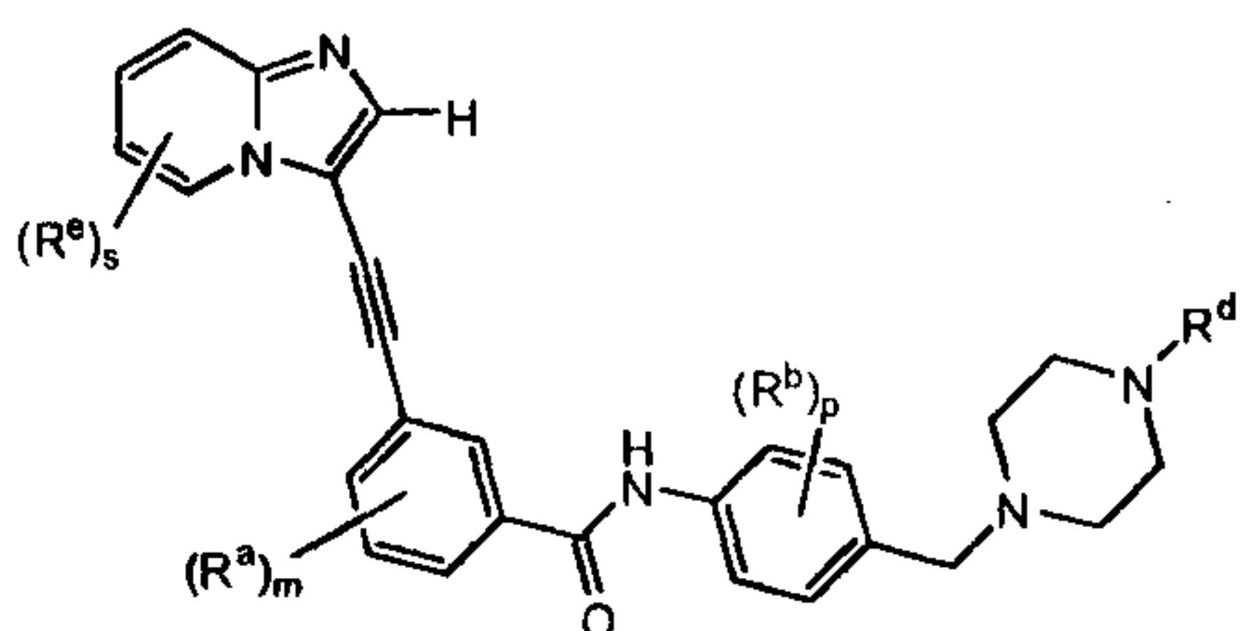
Formula IIIb
