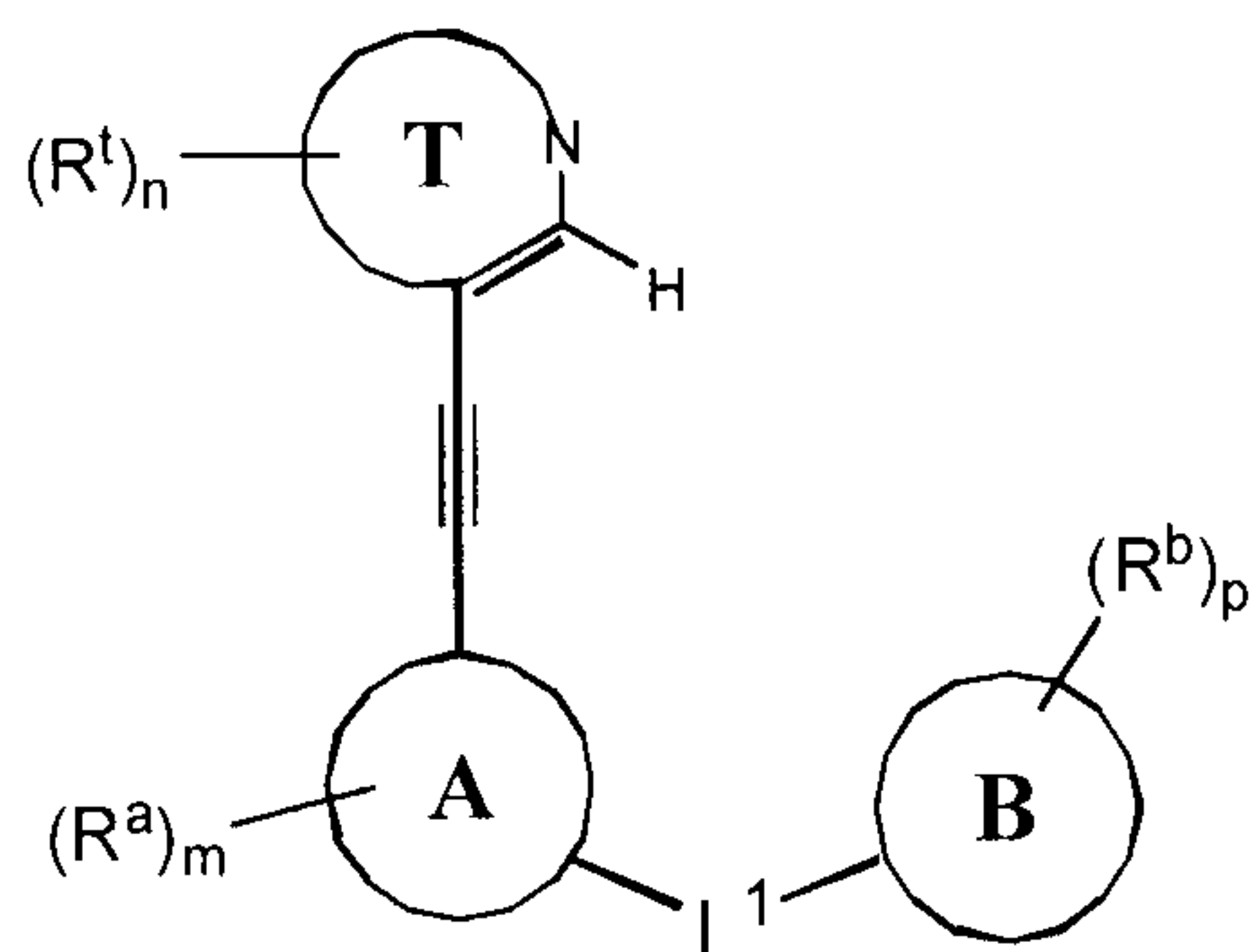
Formula I
