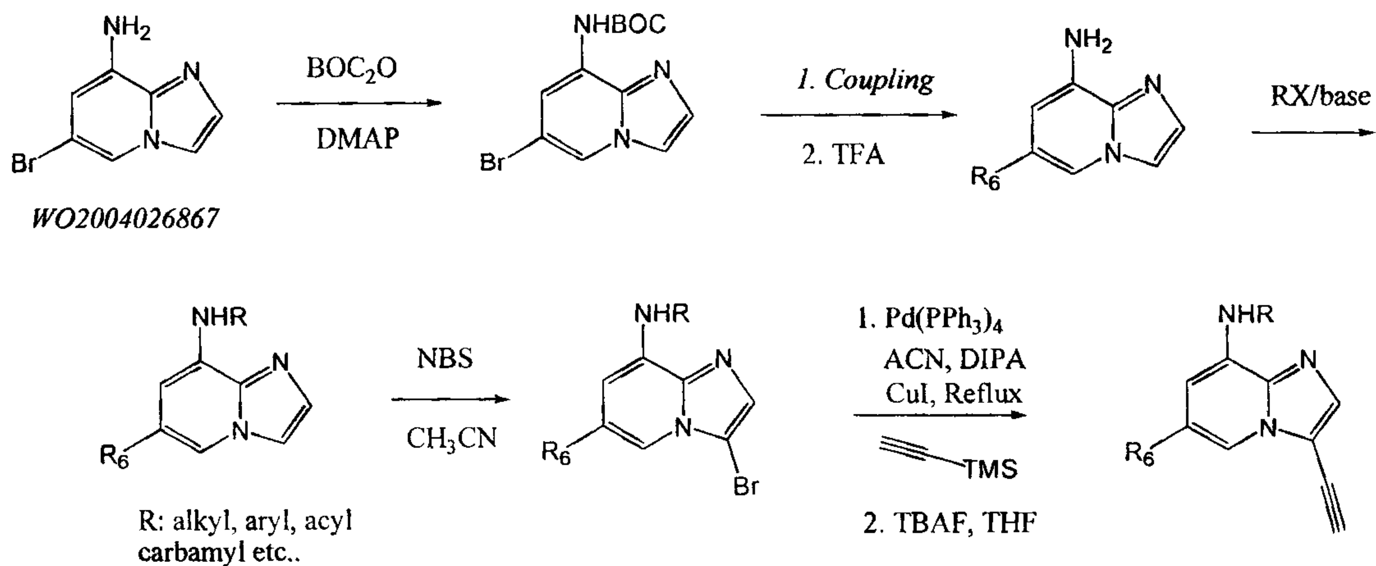
Scheme VIII: Preparation of C-6 and C-8 Substituted 3-Ethynylimidazo [1,2-a] pyridines.
