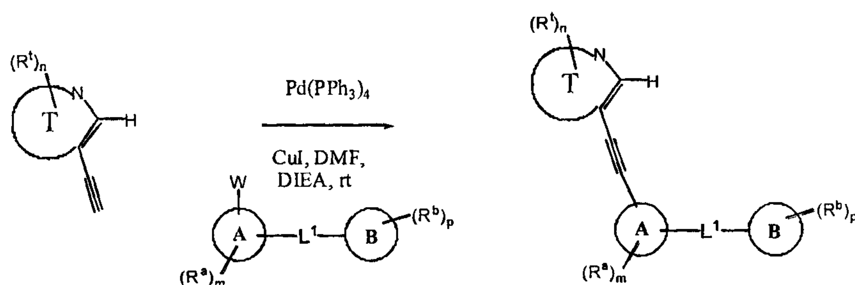
Scheme I: Sonogashira Coupling Reaction
