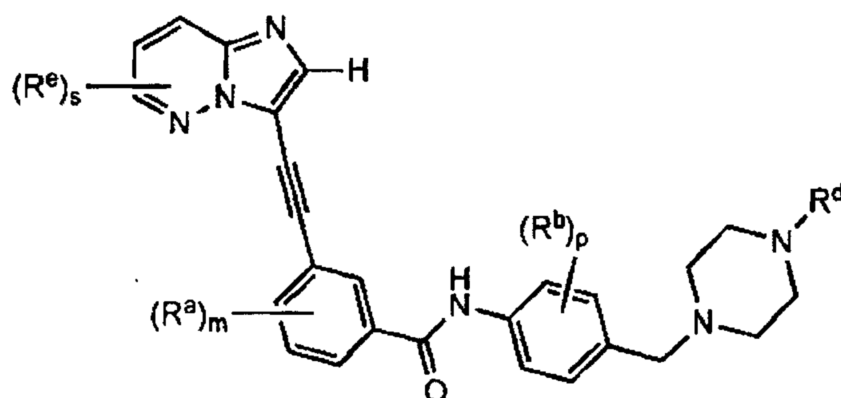
Formula IIIc
