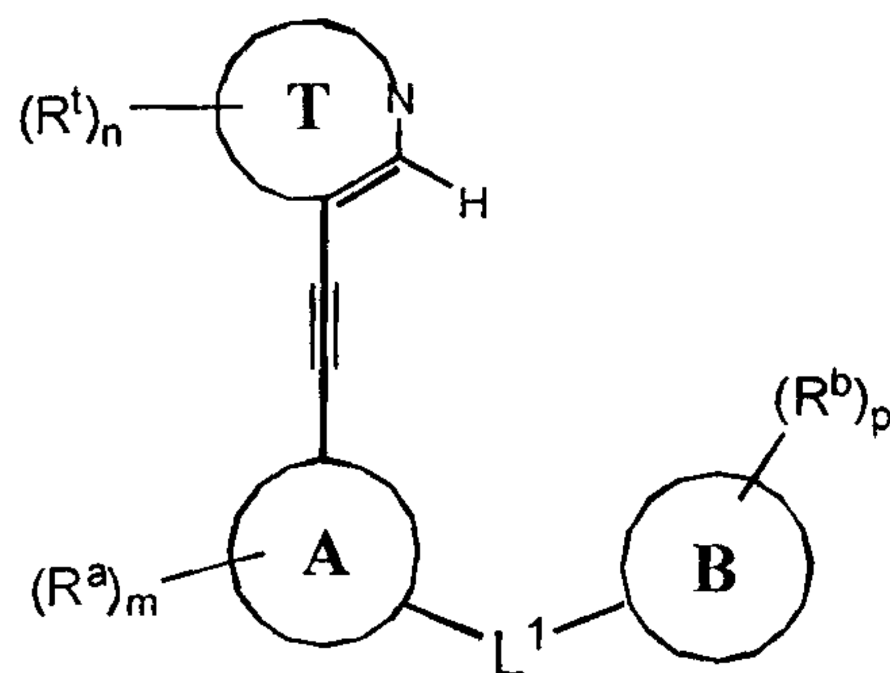
Formula I
