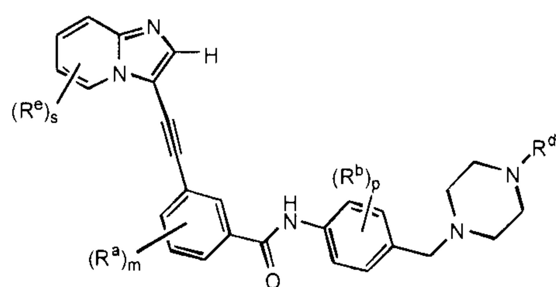
Formula IIIb
