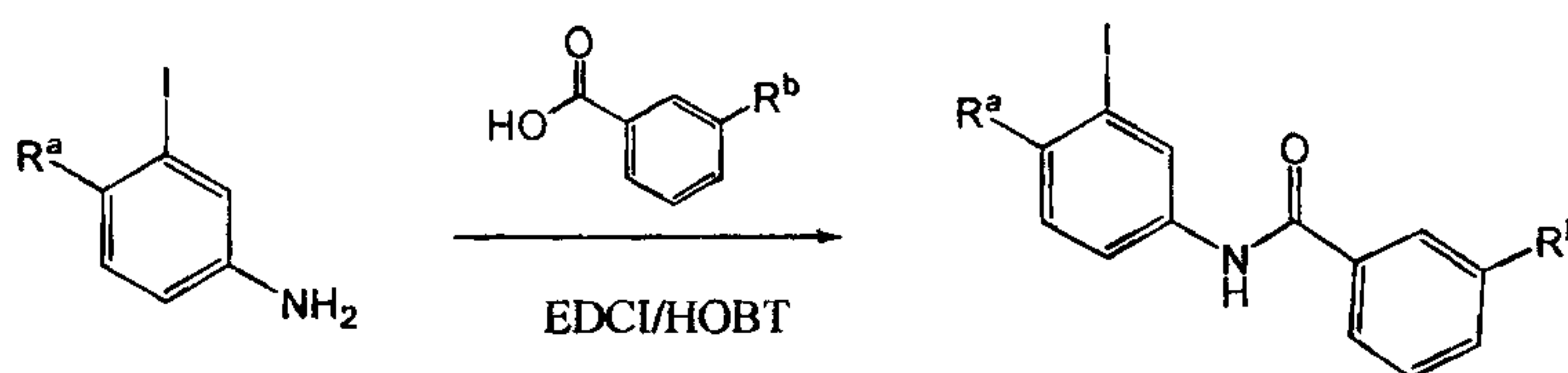
Scheme IX
