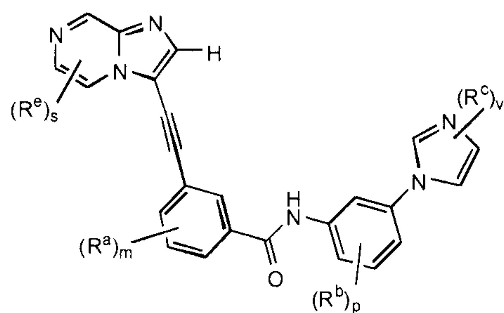
Formula IIa
