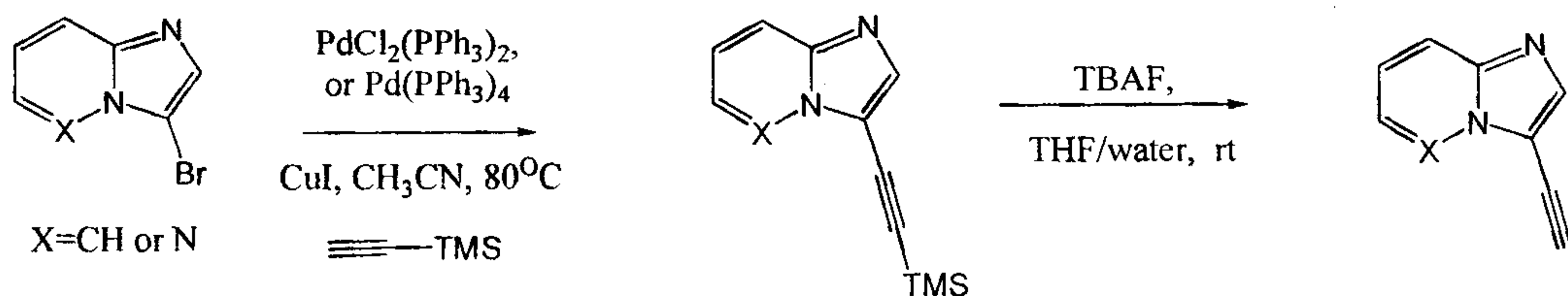
Scheme V: Preparation of 3-Ethynylimidazo[1,2-a]pyridine or 3-Ethynylimidazo[1,2-b]pyridazine
