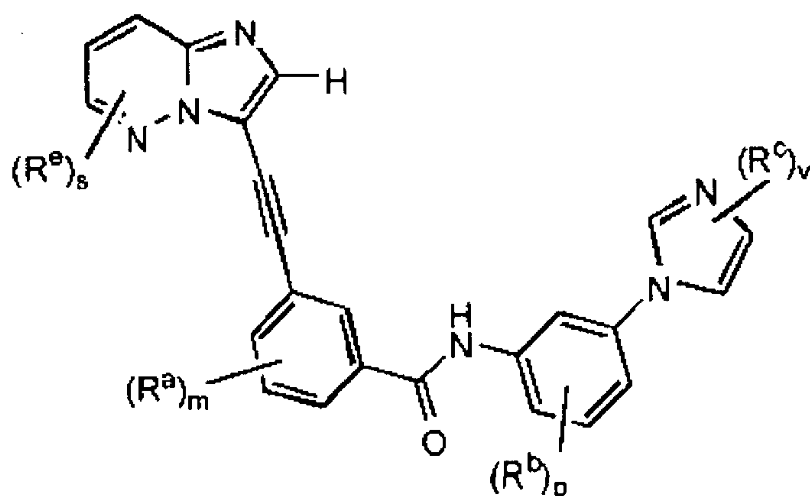
Formula IIc
