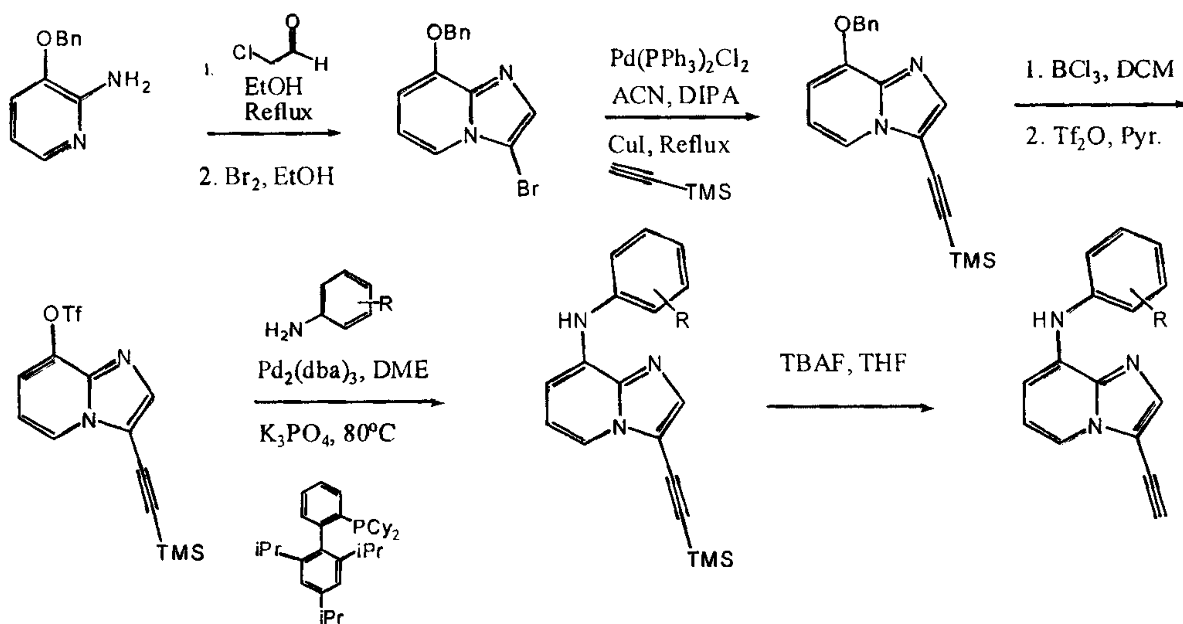
Scheme VI: Preparation of C-8 Amino Substituted 3-Ethynylimidazo[1,2-a]pyridines
