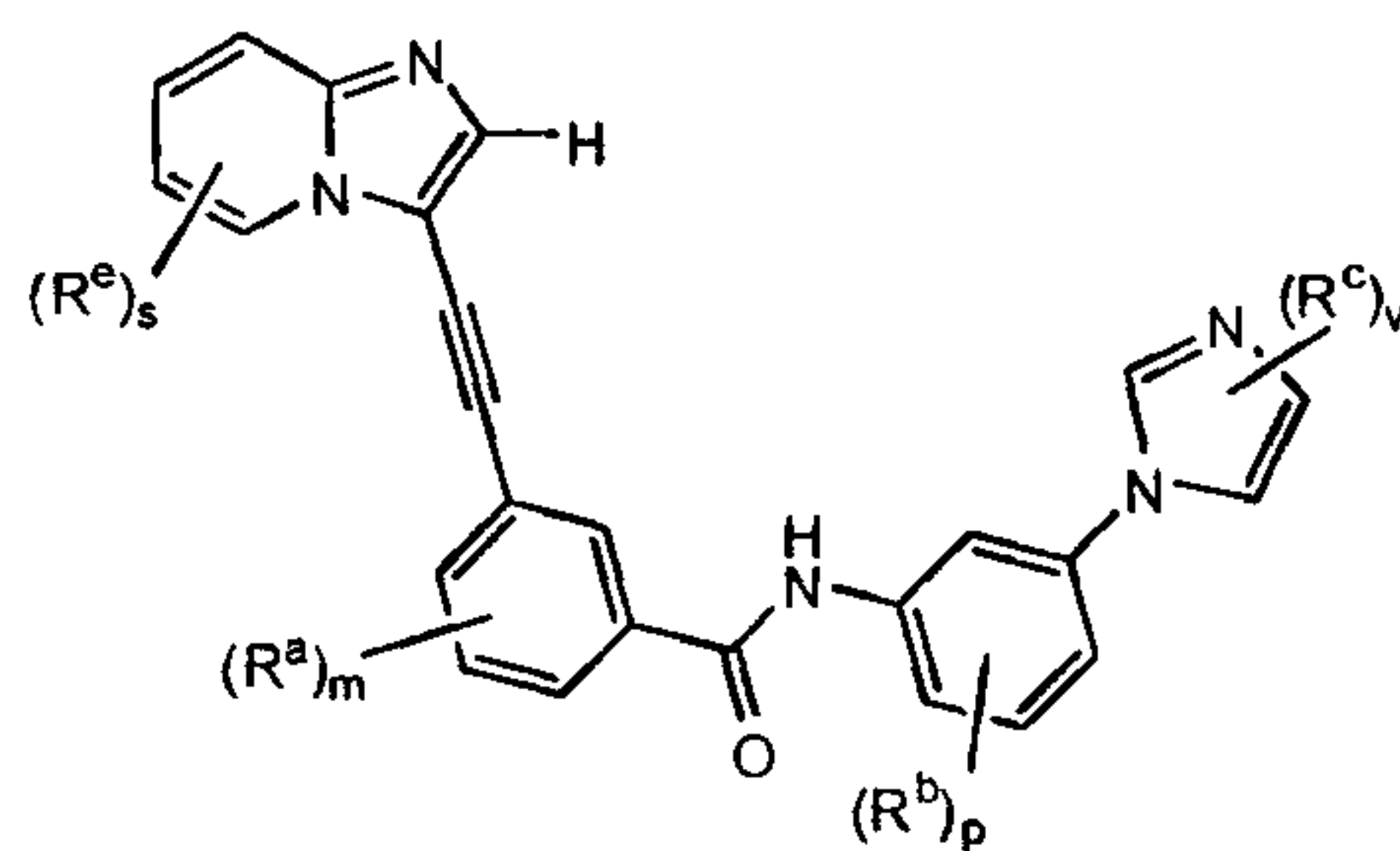
Formula IIb
