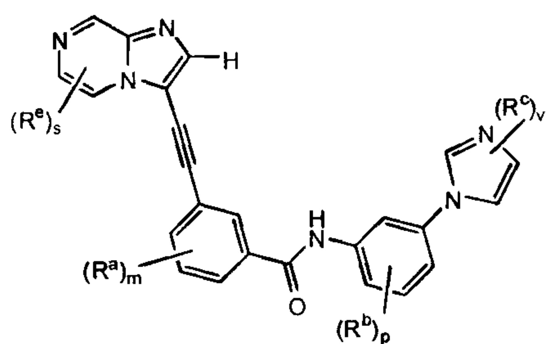
Formula IIa
