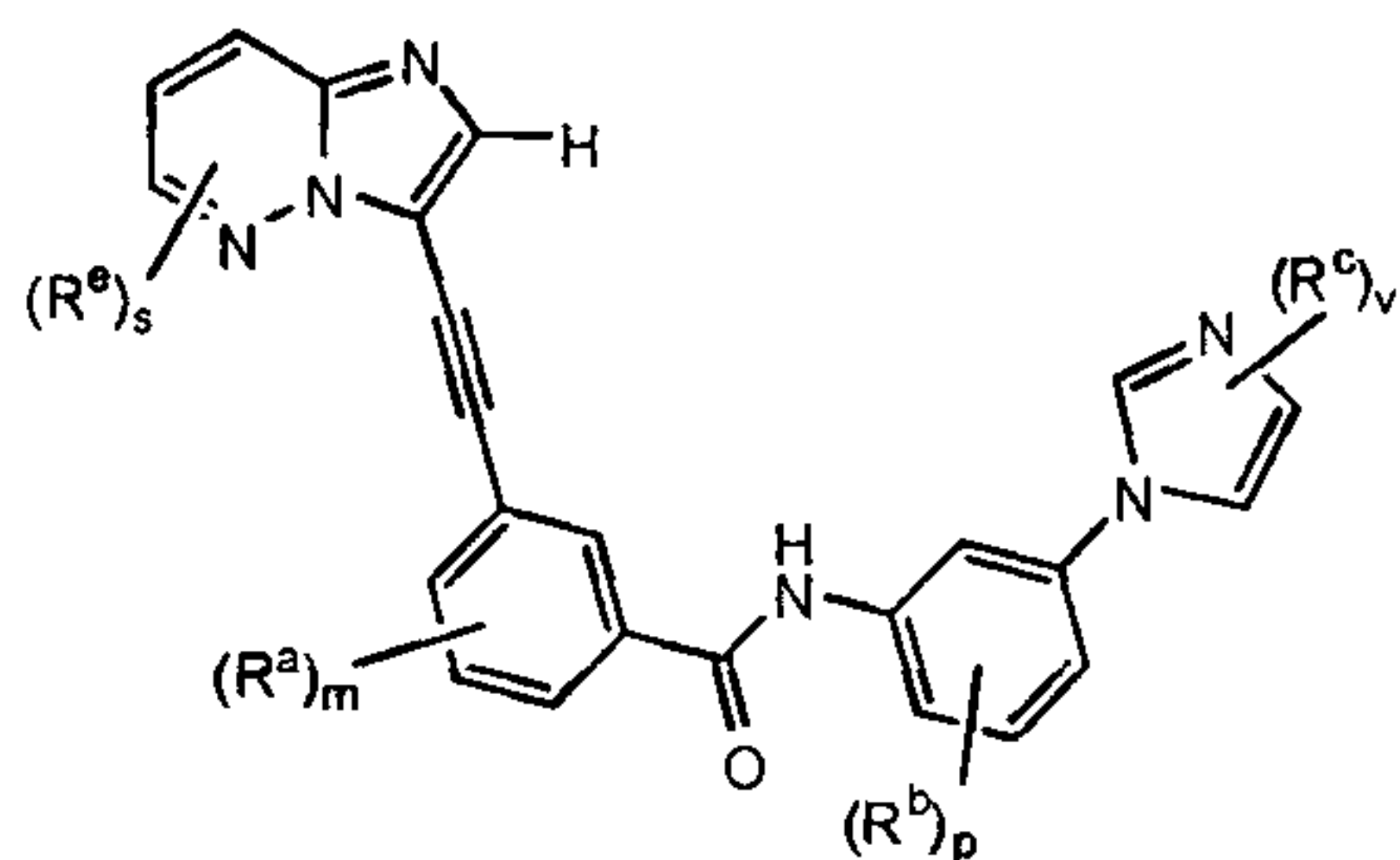
Formula IIc
