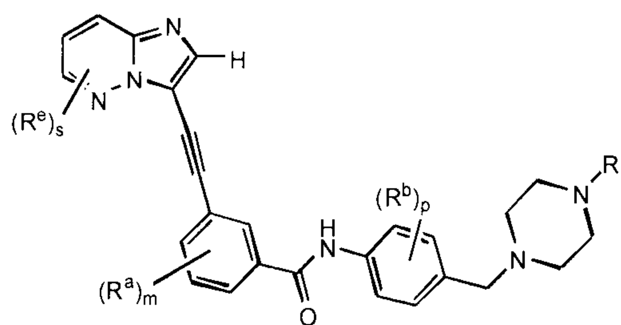
Formula IIIc
