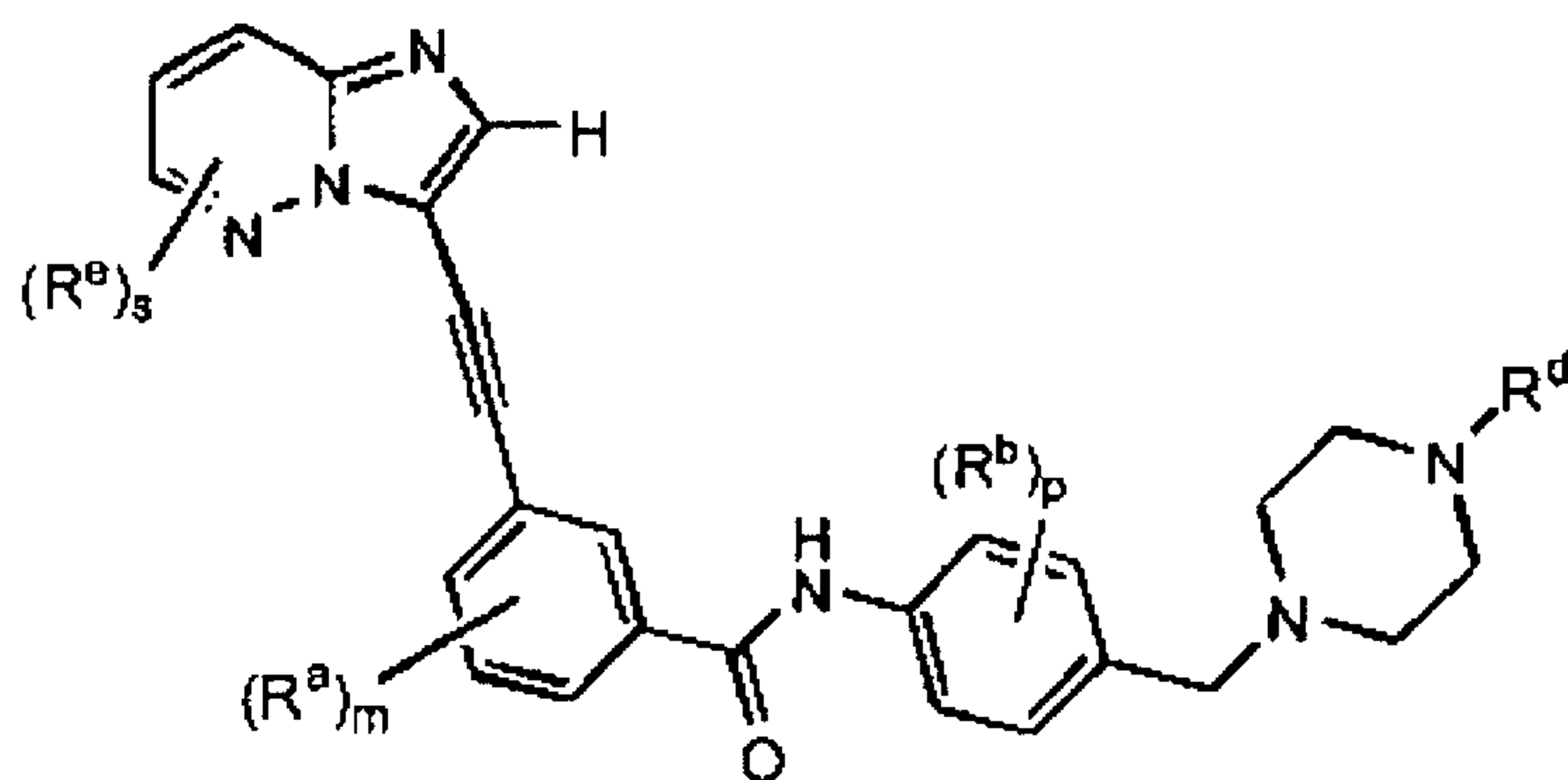
Formula IIIc
