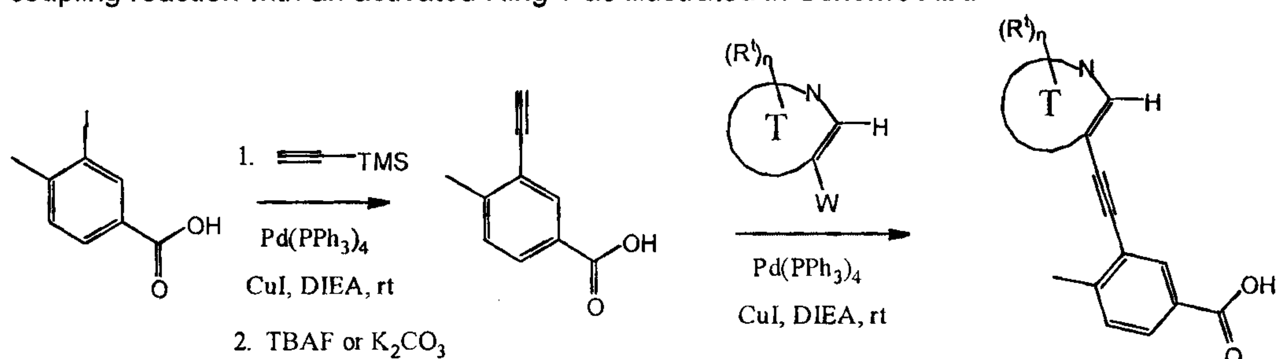
Scheme XIX
