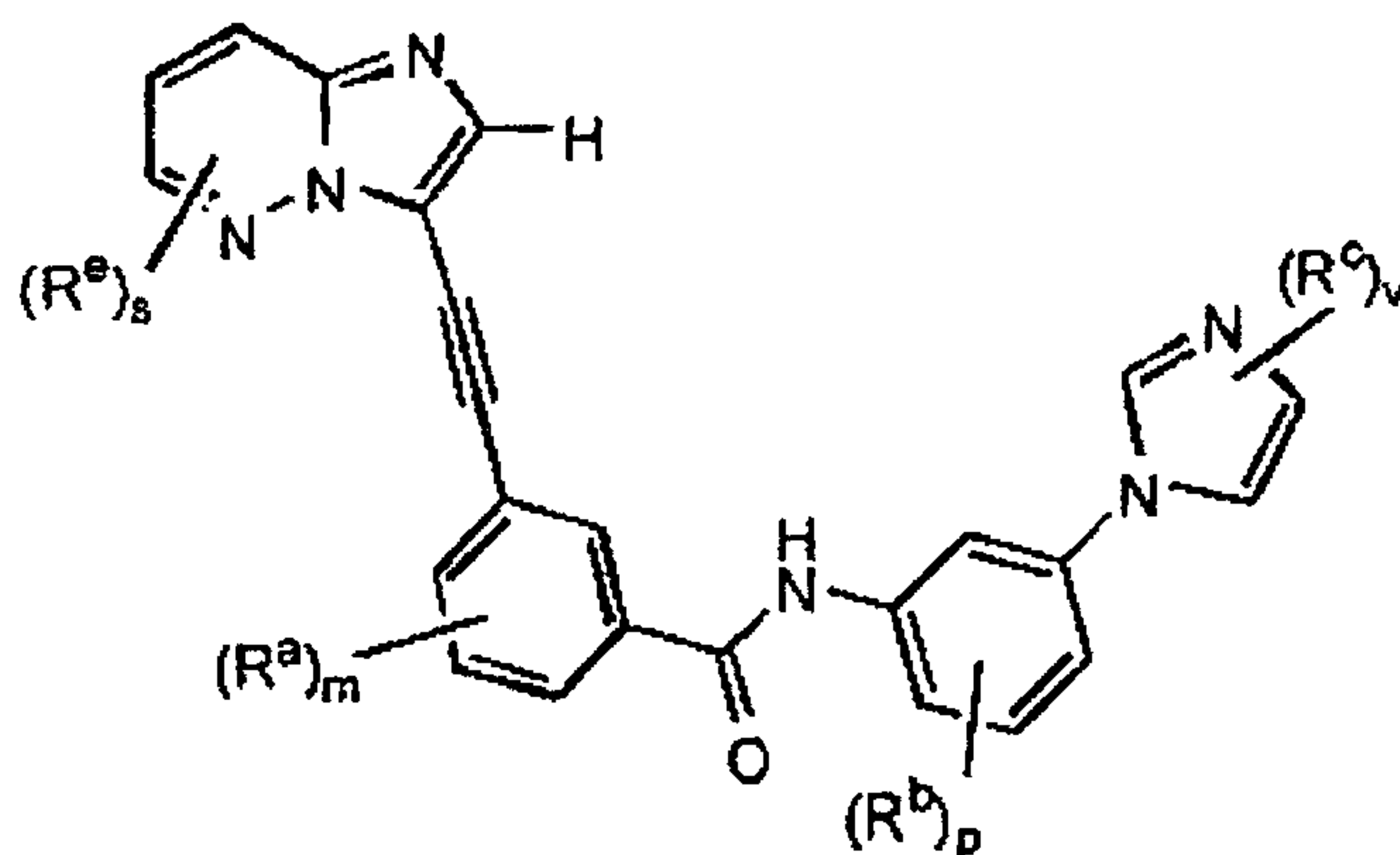
Formula IIc
