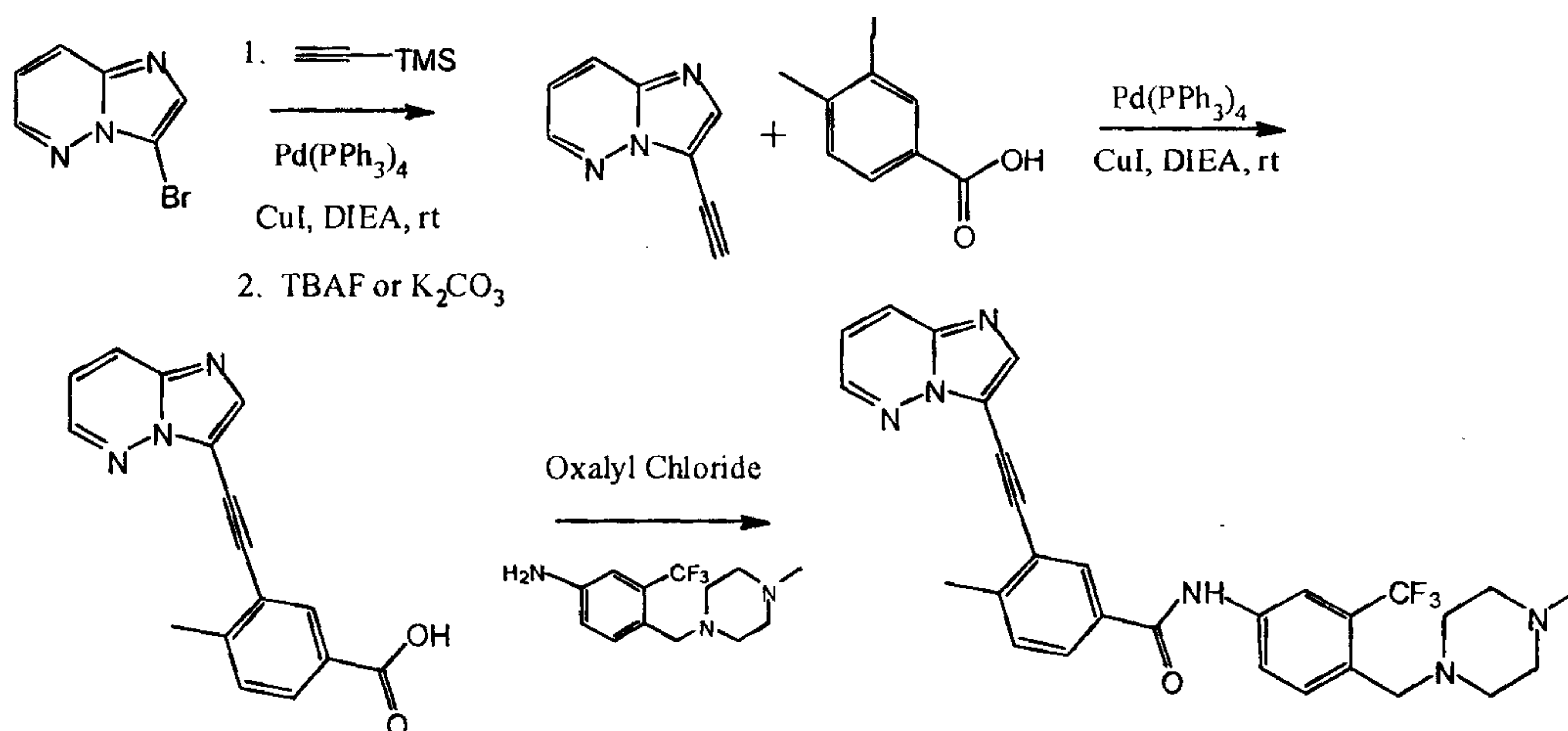
Scheme XVIII
