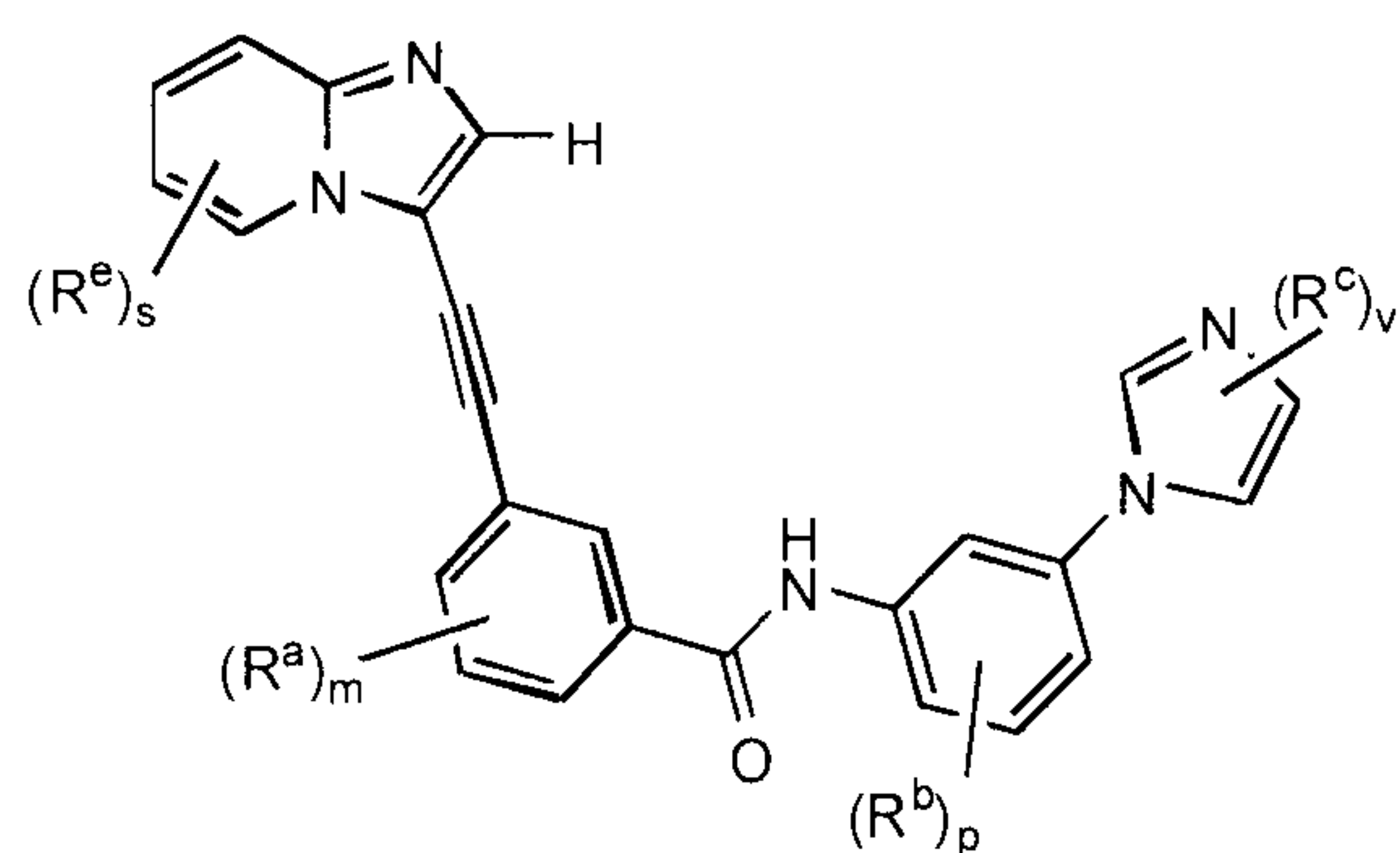
Formula IIb
