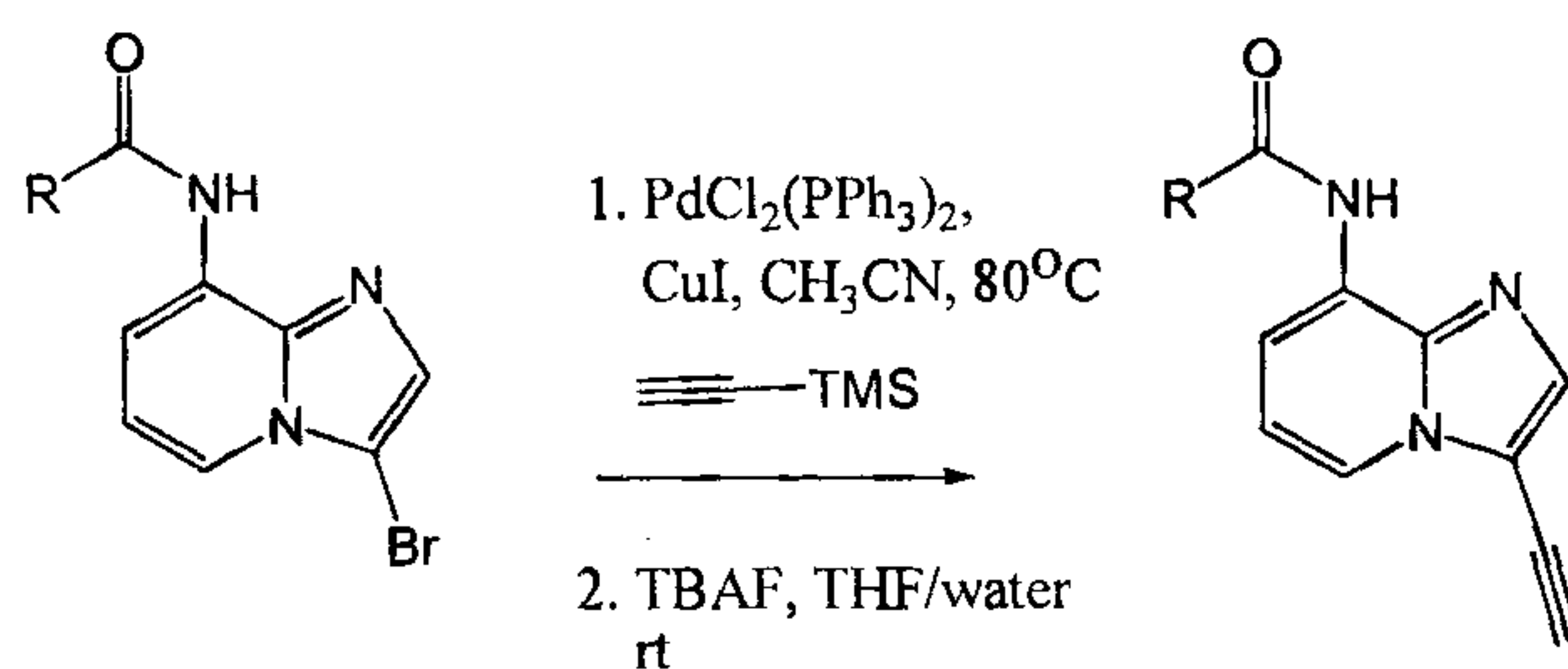
Scheme VII: Preparation of C-8 substituted 3-Ethynylimidazo[1,2-a]pyridines
