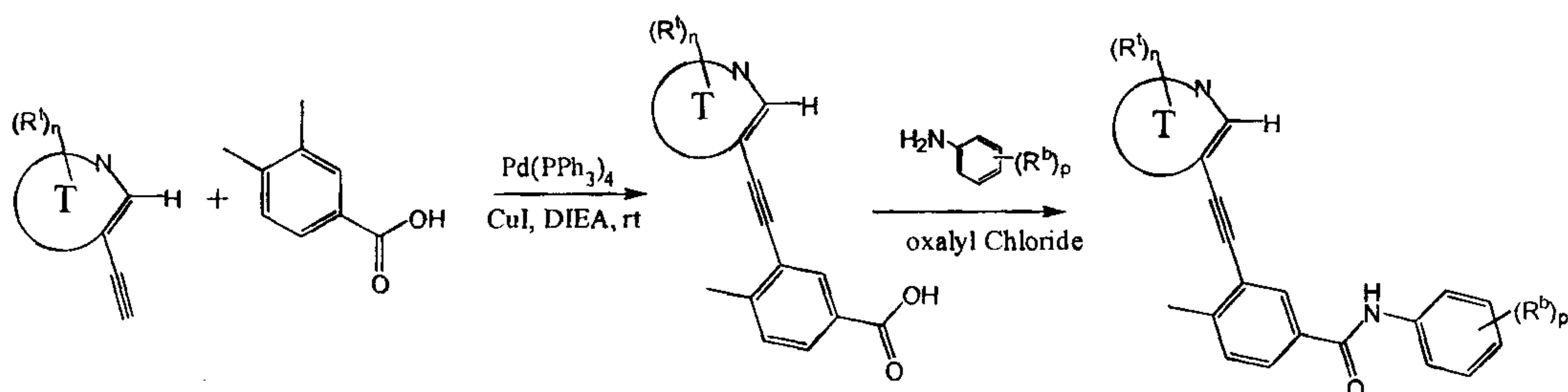
Scheme XVII
