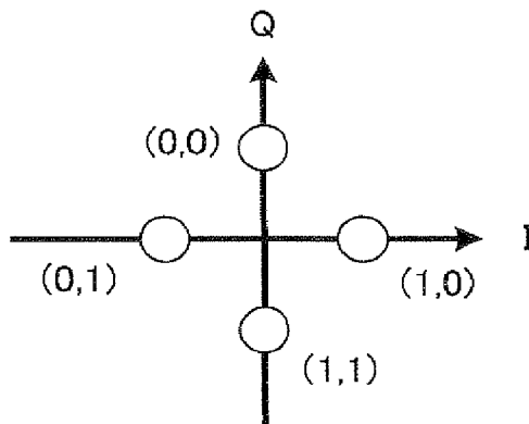
S1(i)' SIGNAL POINT ARRANGEMENT
