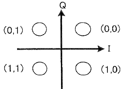
FIG. 11A S1(i) SIGNAL POINT ARRANGEMENT
