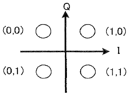
S1(i)' SIGNAL POINT ARRANGEMENT
