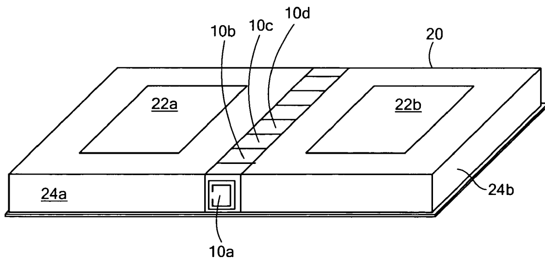
FIG. 2 PRIOR ART
