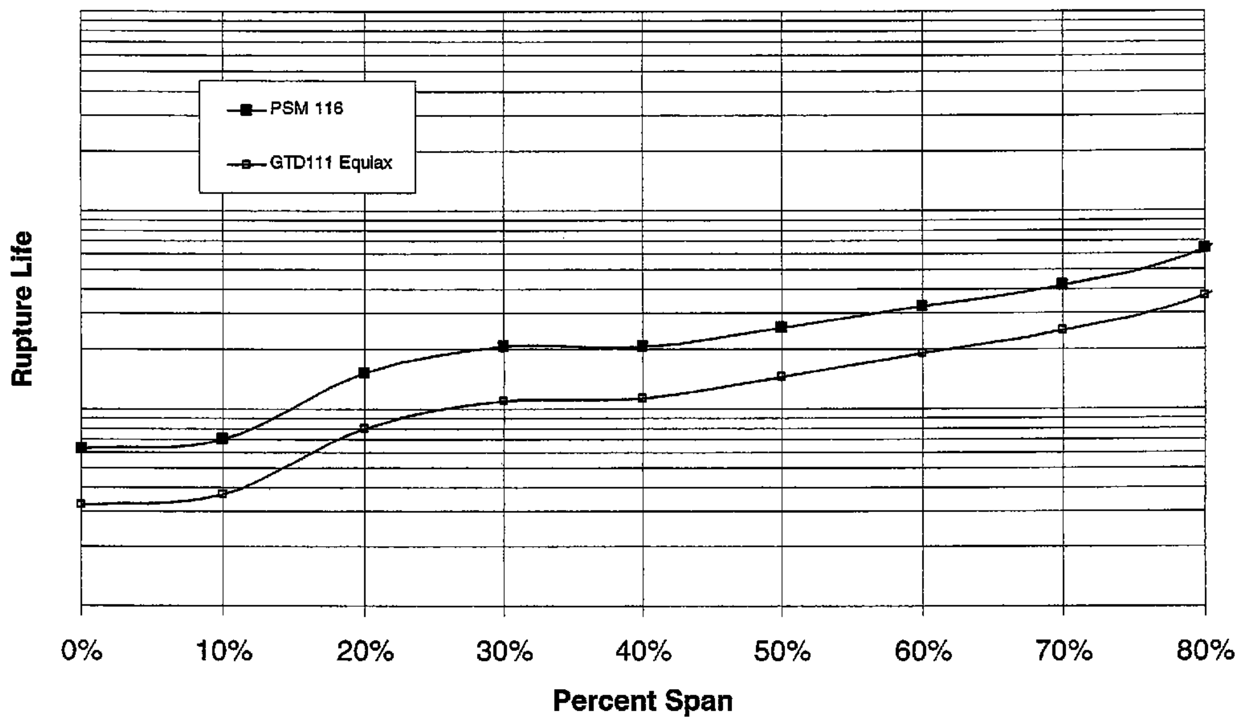
Typical Blade Creep Rupture Life (Equiaxed)
