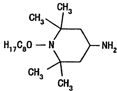
Compound 11
