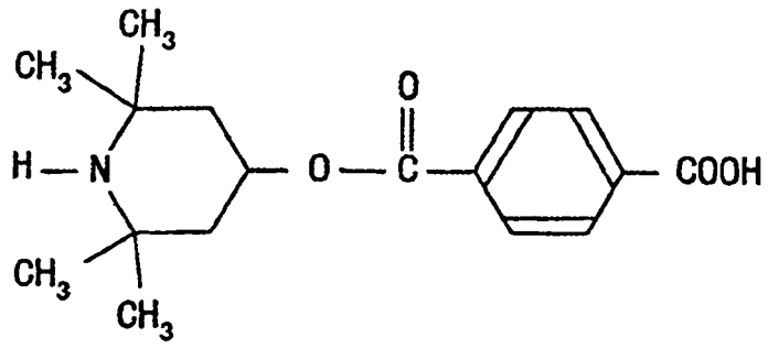
Compound 13
