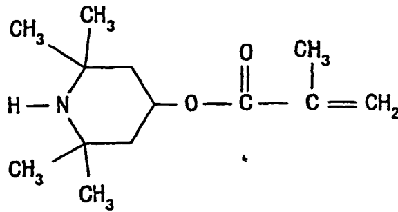
Compound 6
