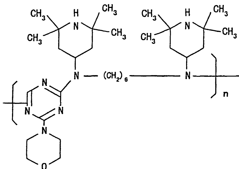
Compound 16
