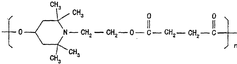
Compound 17
