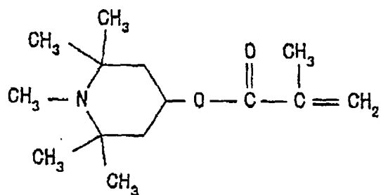
Compound 5
