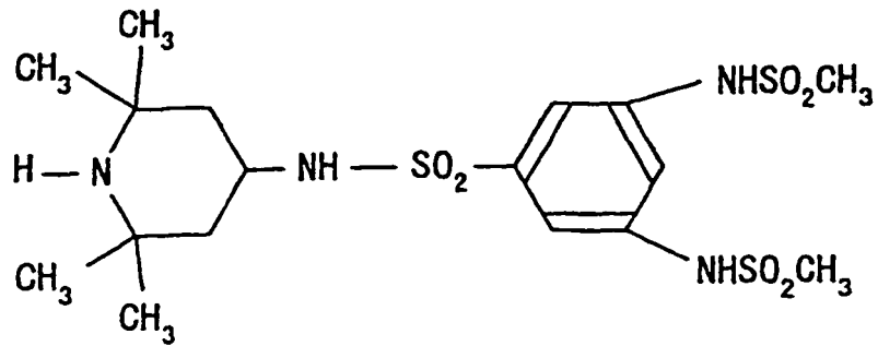
Compound 8
