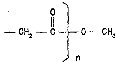
Compound 19
