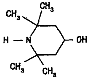
Compound 19
