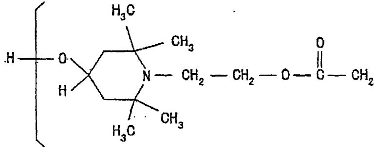
Compound 18
