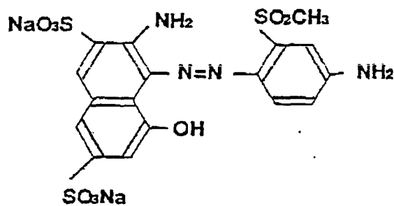
Compound b
