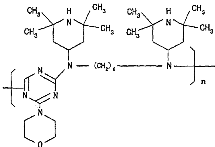
Compound 16
