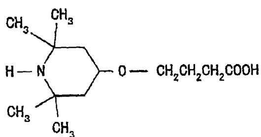
Compound 15
