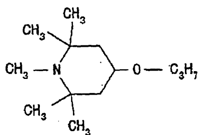
Compound 14
