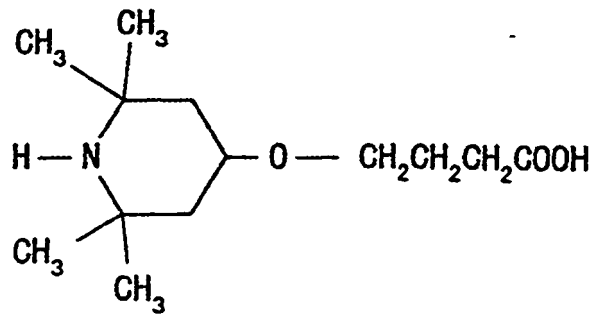
Compound 15
