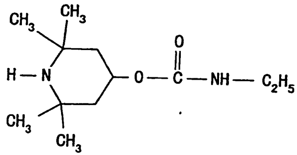
Compound 10
