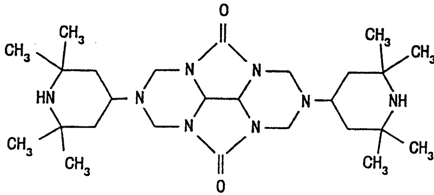
Compound 4
