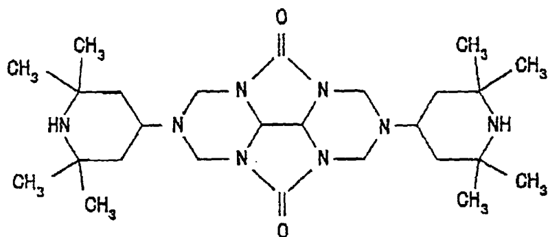
Compound 4
