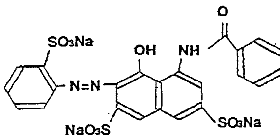
Compound c
