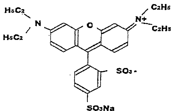
Compound a
