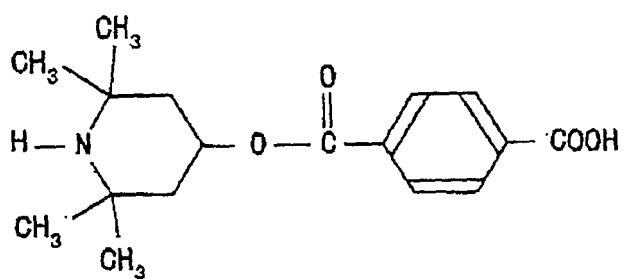
Compound 13
