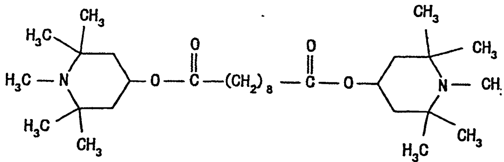
Compound 7
