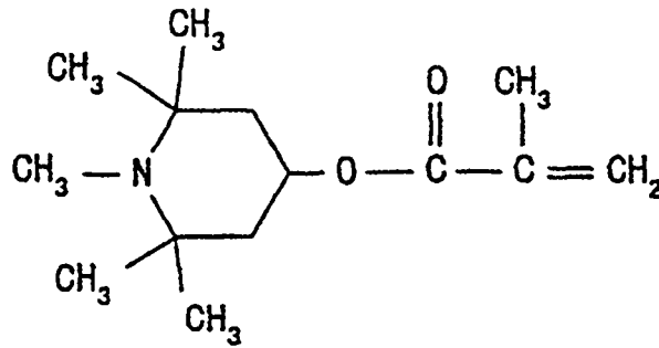
Compound 5
