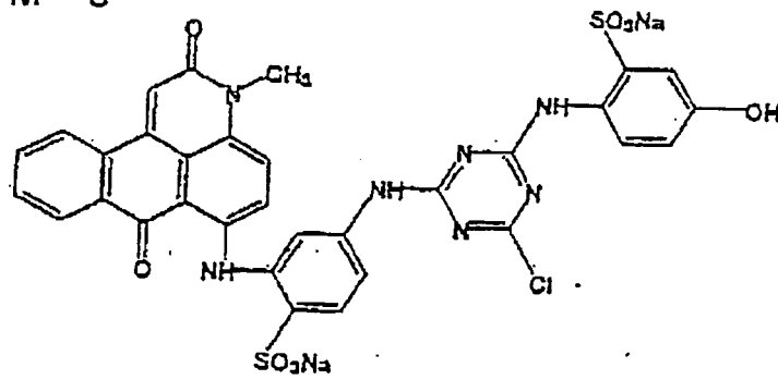
M-8
