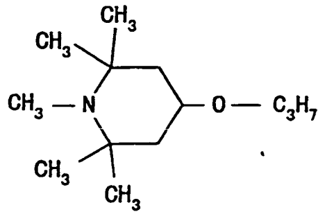
Compound 14
