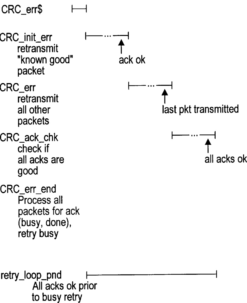
Retry Loop timing diagram - Send port
