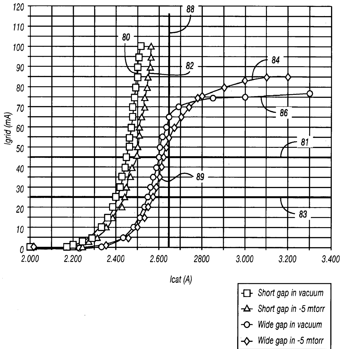
Cathode Current - Grid Current Characteristics
