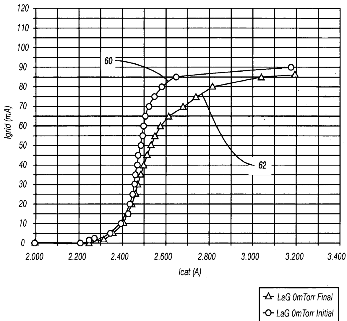
Cathode Test Cells #09 Initial versus Final Igrid vs Icat
