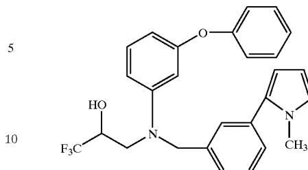
3-[(3-phenoxyphenyl)[[3-(1-methyl-1H-pyrrol-2-yl)phenyl]methyl]amino]-1,1,1-trifluoro-2-propanol
