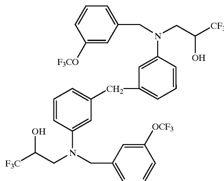
1,1'-[methylenebis[3,1-phenylene]]bis[3-(trifluoromethoxy)phenyl]methyl]imino]]bis[3,3,3-trifluoro-2-propanol]
