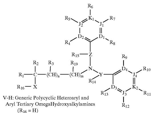
Scheme 17
