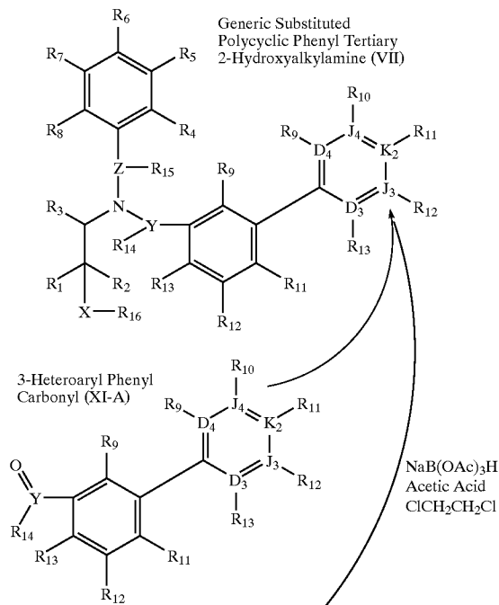
Scheme 56
