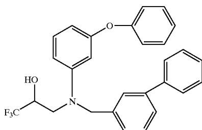
3-[(3-phenoxyphenyl)[[1,1'-biphenyl]-3-ylmethyl]amino]-1,1,1-trifluoro-2-propanol
