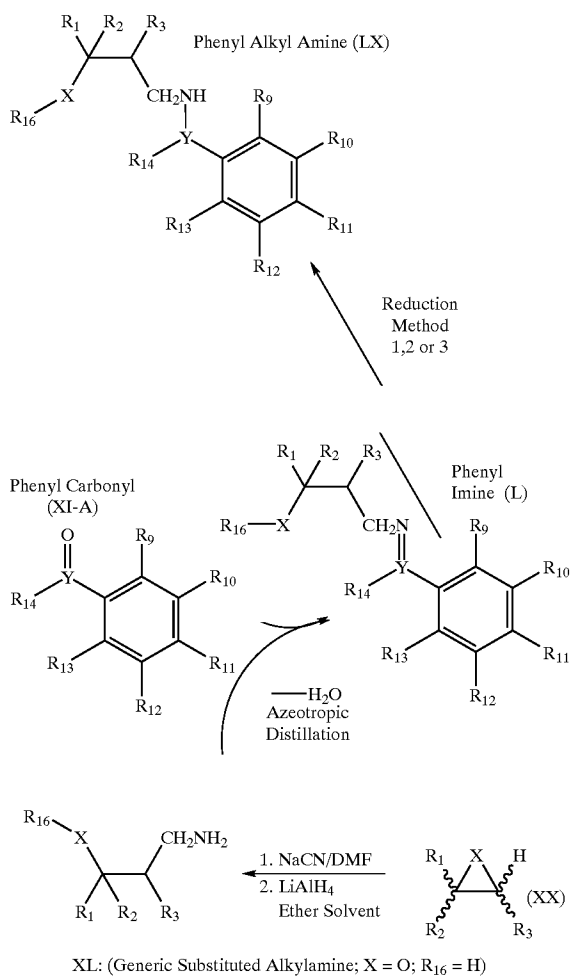
Scheme 33
