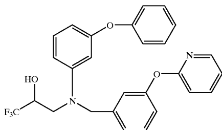
3-[(3-phenoxyphenyl)[[3-(2-pyrimidinyl-oxy)phenyl]methyl]amino]-1,1,1-trifluoro-2-propanol
