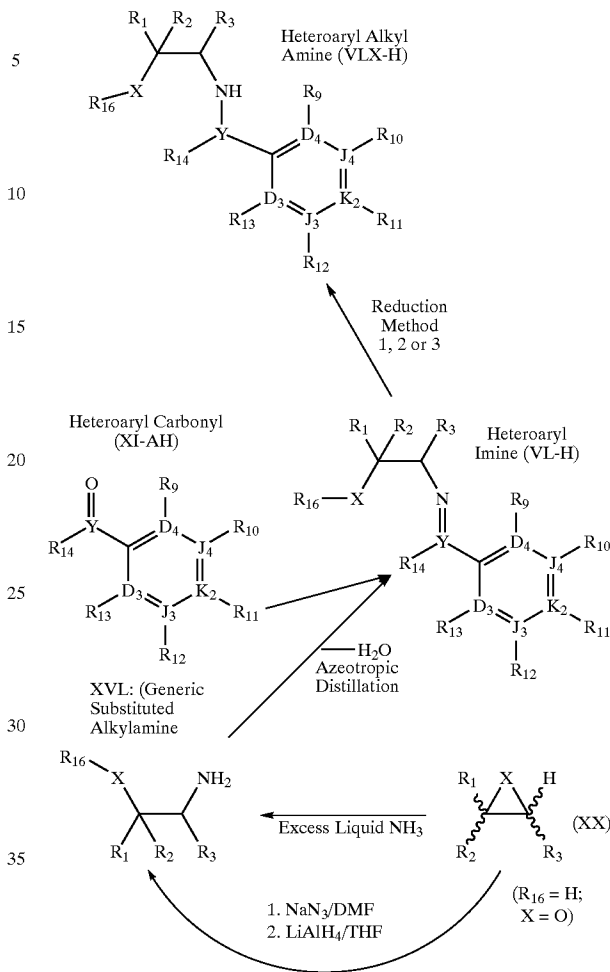
Scheme 45
