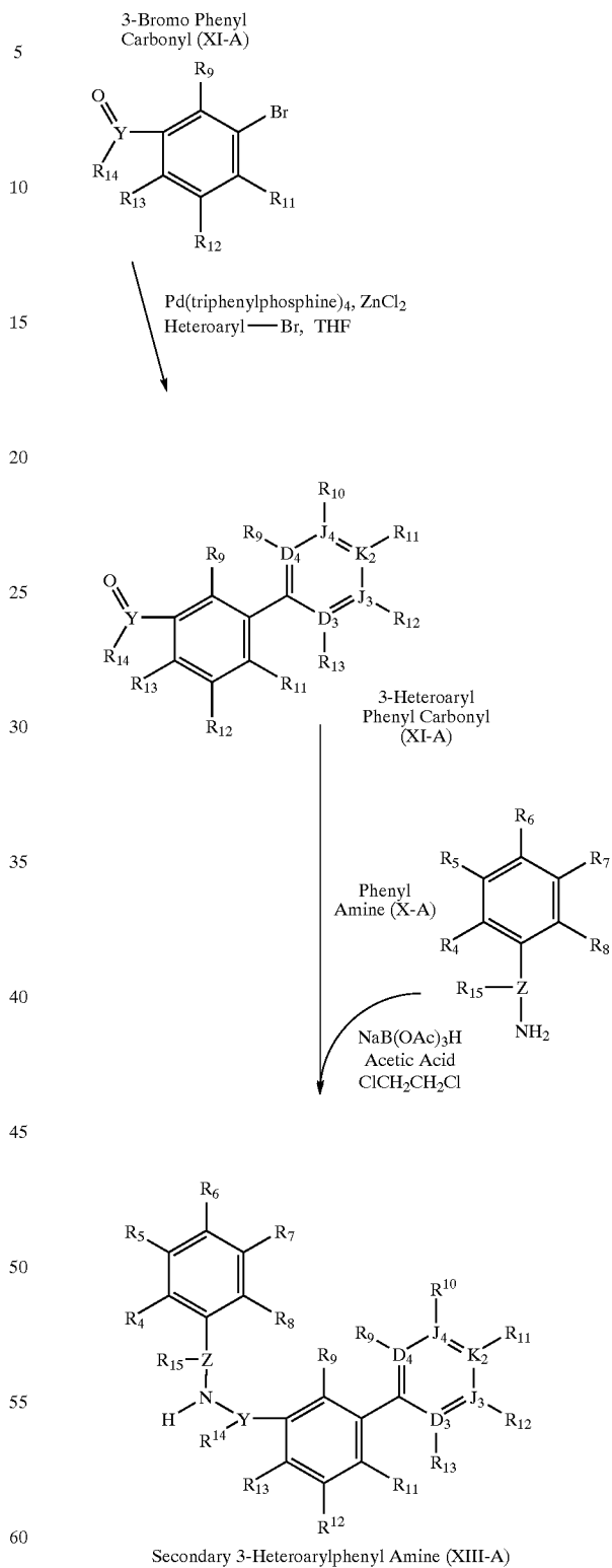
Scheme 43
