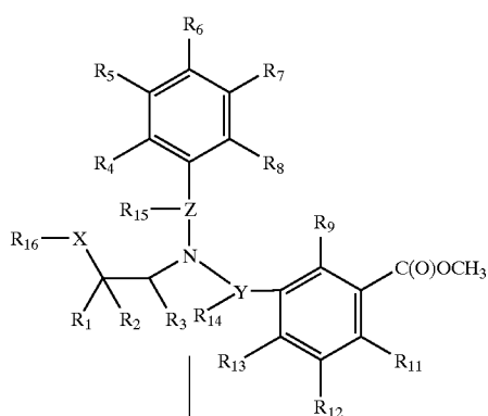
Scheme 39
