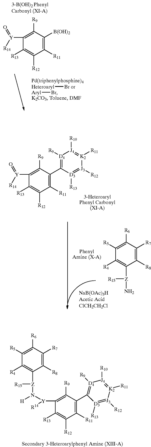
Scheme 44
