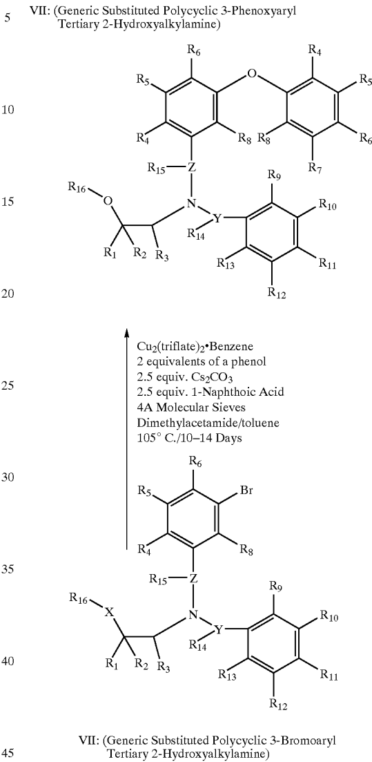
Scheme 8
