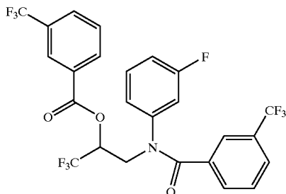
2,2,2-trifluoro-1-[[[(3-fluorophenyl)[3-(trifluoromethyl)benzoyl]amino]-methyl]ethyl]3-trifluoromethylbenzoate
