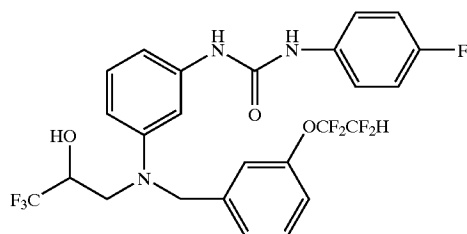
N-(4-fluorophenyl)-N'-[3-[[[3-(1,1,2,2-tetrafluoroethoxy)phenyl]methyl]amino]-1,1,1-trifluoro-2-hydroxypropyl]phenyl]urea
