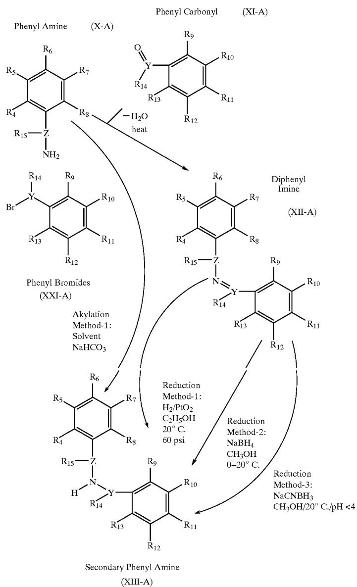
Scheme 2
