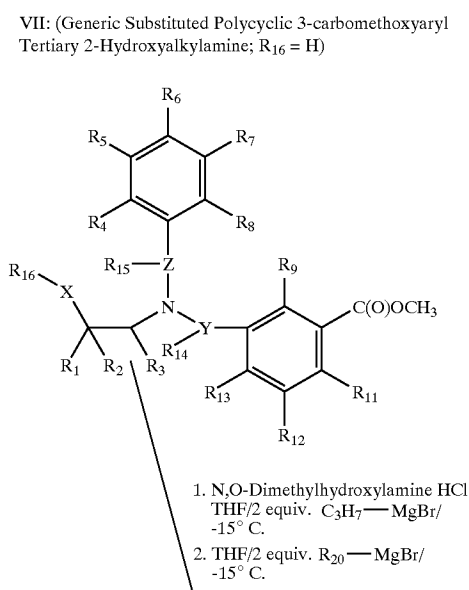
Scheme 55
