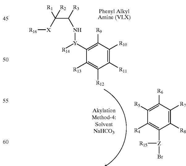
Scheme 49
