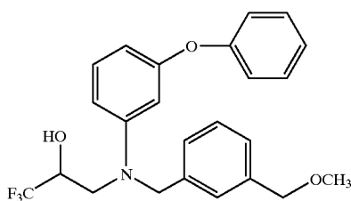
3-[[3-(3-phenoxyphenyl)(3,3,3-trifluoro-2-hydroxypropyl)amino]methyl]methoxymethylbenzene
