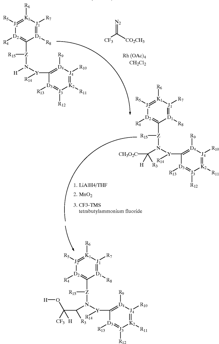
Scheme 57
