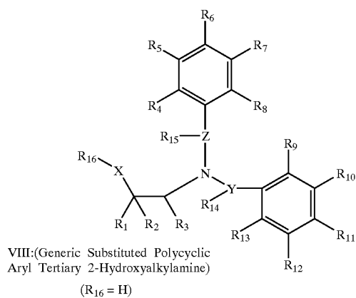
Scheme 18
