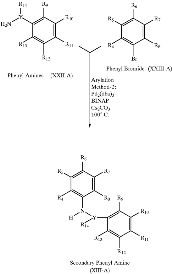
Scheme 10
