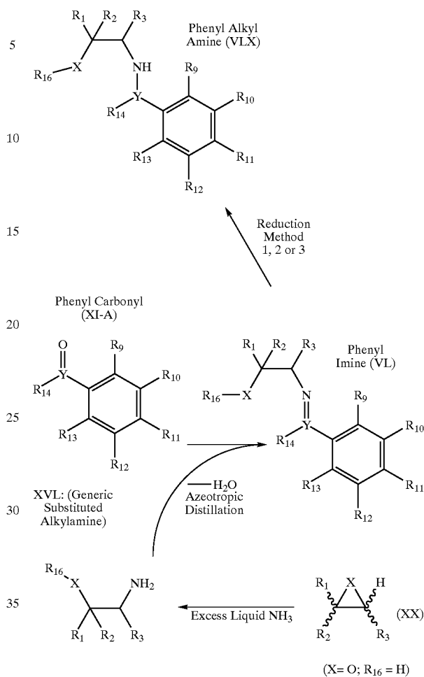
Scheme 48
