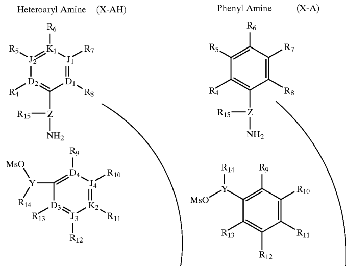
Scheme 4
