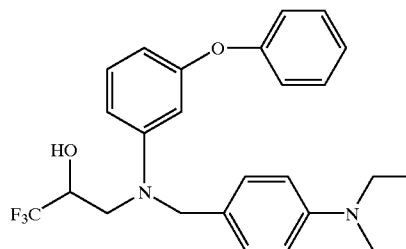
3-[(3-phenoxyphenyl)[4-(N,N-diethylamino)phenyl]methyl]amino]-1,1,1-trifluoro-2-propanol
