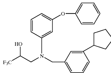
3-[(3-phenoxyphenyl)[3-cyclopentylphenyl]methyl]amino]-1,1,1-trifluoro-2-propanol
