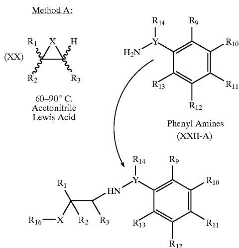
Scheme 58
