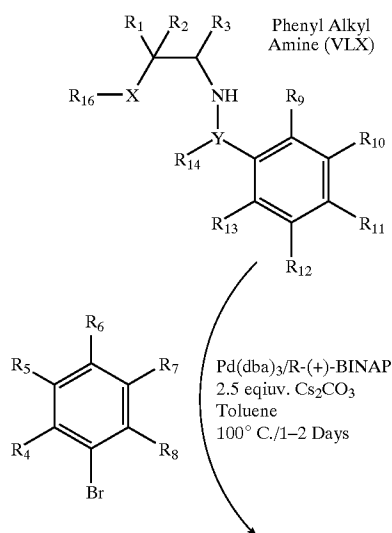
Scheme 50
