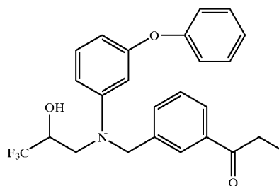
1-[3-[[3-(phenoxyphenyl)(3,3,3-trifluoro-2-hydroxypropyl)-amino]methyl]phenyl]-1-propanone
