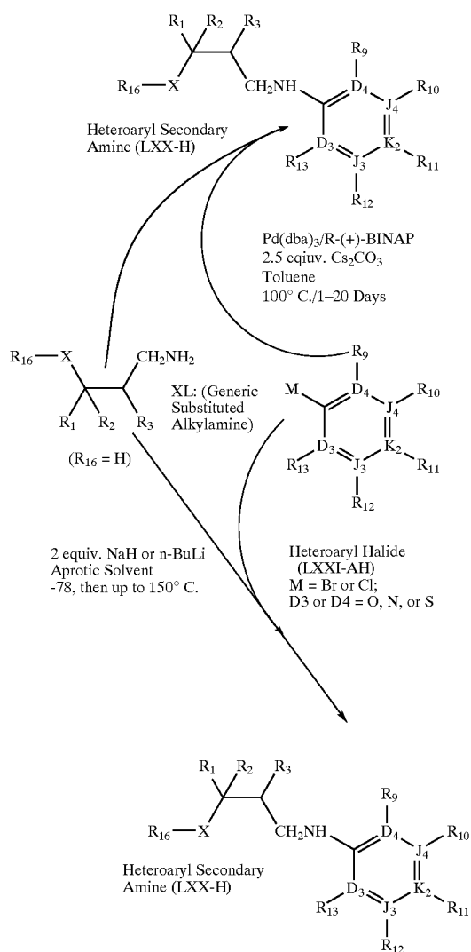
Scheme 53
