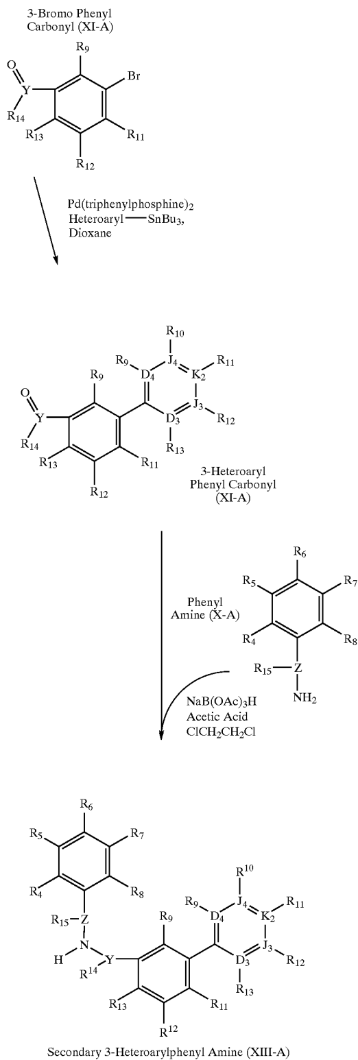
Scheme 42
