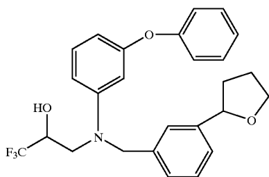
3-[(3-phenoxyphenyl)[[3-(tetrahydro-2-furanyl)phenyl]methyl]amino]-1,1,1-trifluoro-2-propanol
