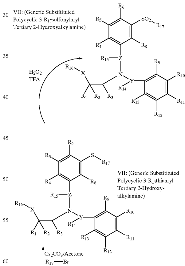
Scheme 19
