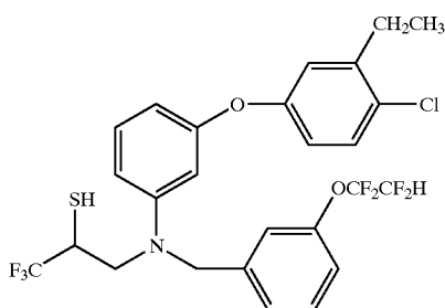
3-[[3-(4-chloro-3-ethylphenoxy)phenyl]-[[3-(1,1,2,2-tetrafluoroethoxy)phenyl]methyl]amino]-1,1,1-trifluoro-2-propanethiol
