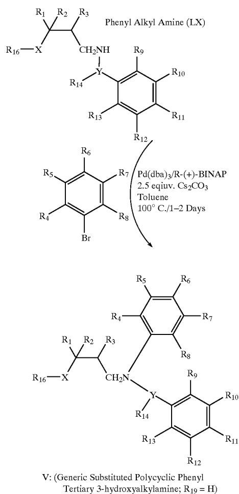
Scheme 35
