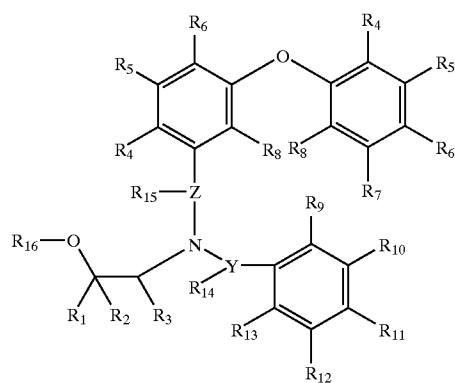
Scheme 14
