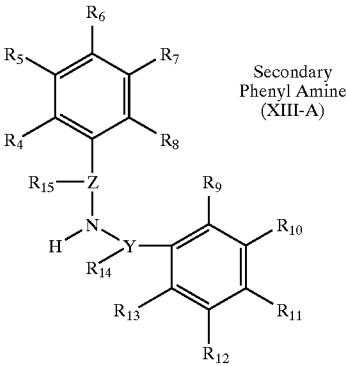
Scheme 11
