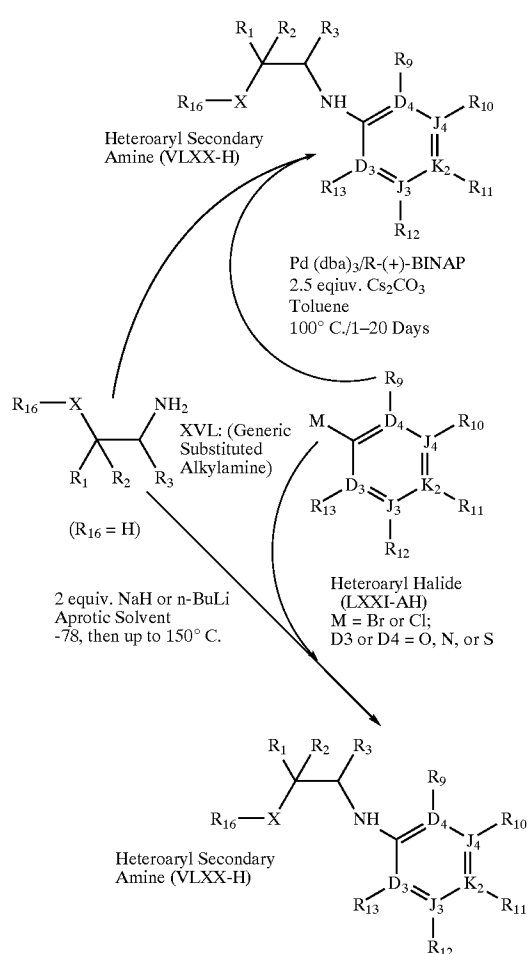
Scheme 51
