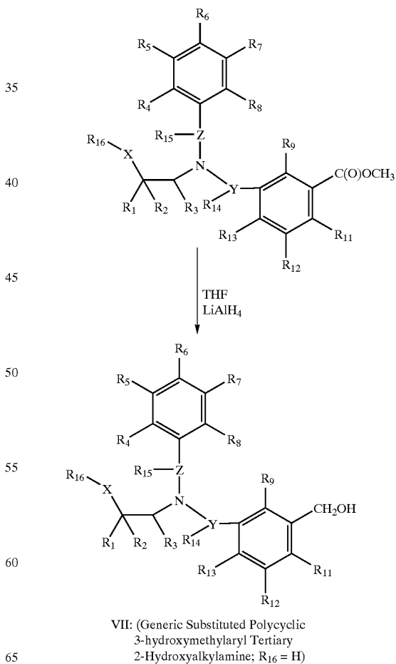
Scheme 38
