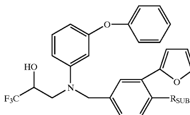
3-[(3-phenoxyphenyl)[[4-substituted-3-(2-furanyl)-phenyl]methyl]amino]-1,1,1-trifluoro-2-propanols.
