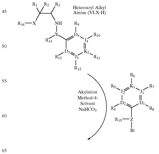
Scheme 46
