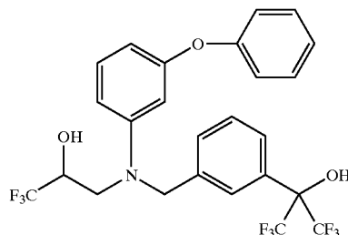
\alpha,\alpha -bis(trifluoromethyl)-3-[[3-(phenoxyphenyl)(3,3,3-trifluoro-2-hydroxypropyl)amino]methyl]benzenemethanol
