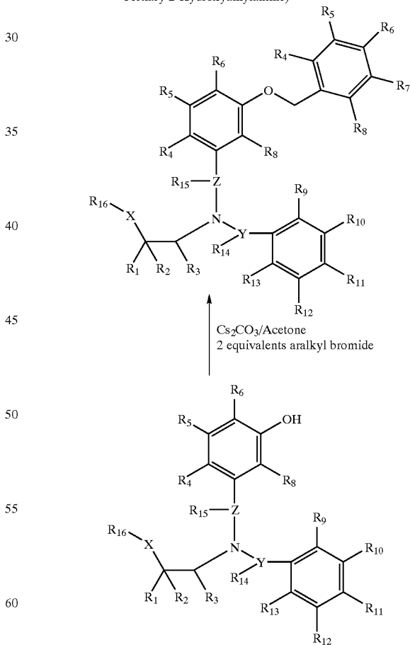
Scheme 16
