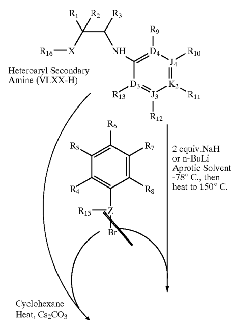
Scheme 52
