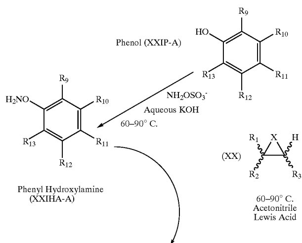
Scheme 59
