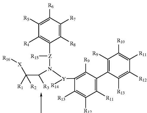
Scheme 40
