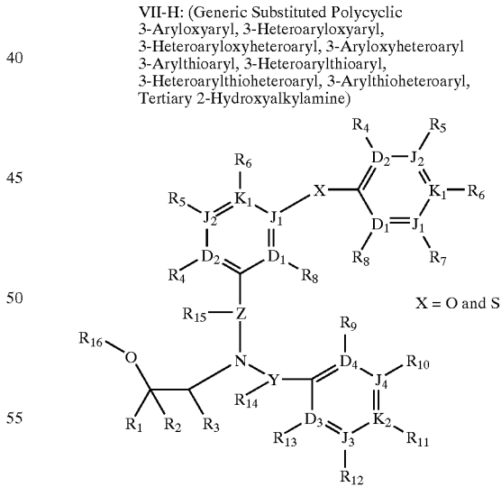
Scheme 12
