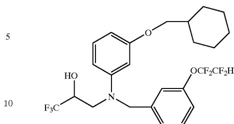
3-[[3-(cyclohexylmethoxy)phenyl][[3-(1,1,2,2-tetrafluoroethoxy) phenyl]-methyl]amino]-1,1,1-trifluoro-2-propanol
