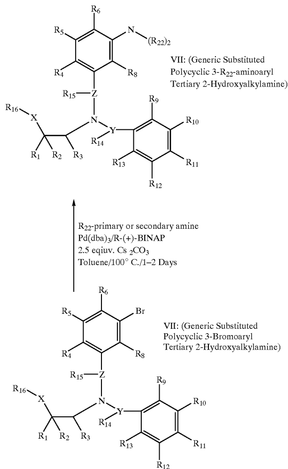
Scheme 23
