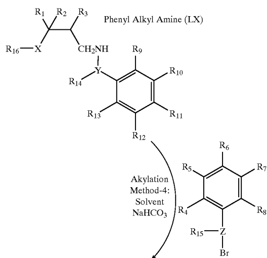
Scheme 34
