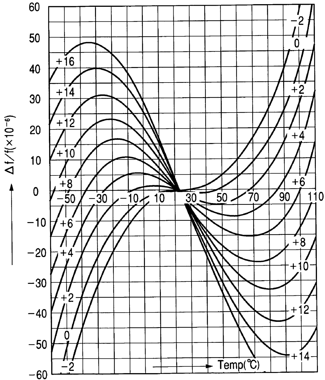
EXAMPLE OF FREQUENCY-TEMPERATURE CHARACTERISTIC OF AT-CUT
