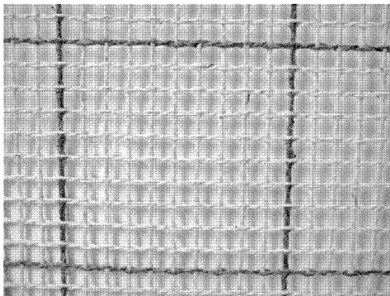
Figure 1. Fiber Mesh Support with 5 mm Open Mesh Size
