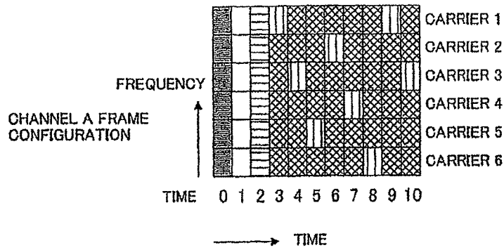
BASE STATION TRANSMIT SIGNAL FRAME CONFIGURATION
