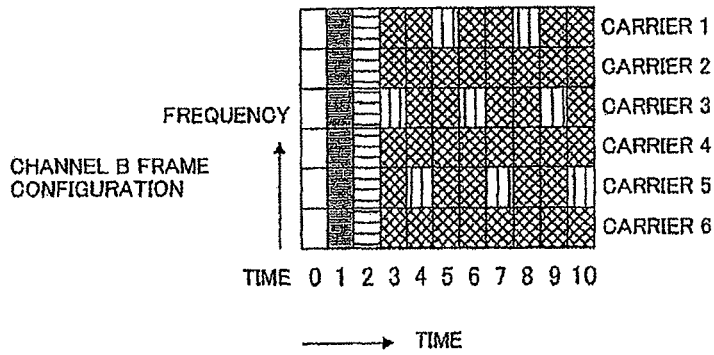
BASE STATION TRANSMIT SIGNAL FRAME CONFIGURATION
