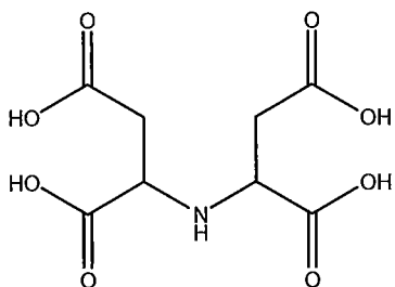
2,2'-Imidosuccinate CAS 7408-20-0, 70543-06-5 (stereospecific)
