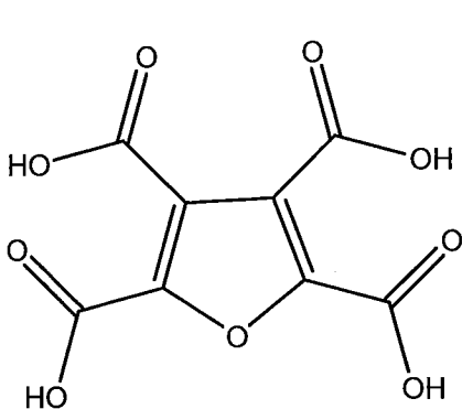
Furan tetracarboxylic acid CAS 20416-04-0
