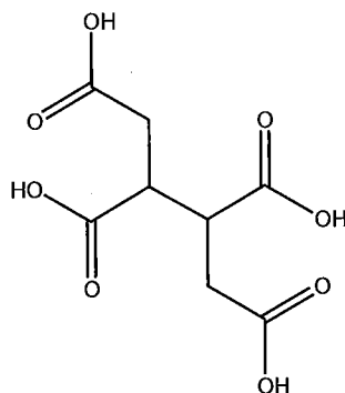
1,2,3,4-Butane tetracarboxylic acid CAS 1703-58-8
