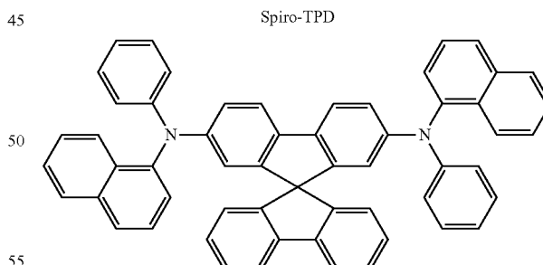
Spiro-NPB
