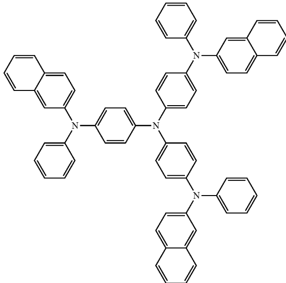
2-TNATA
