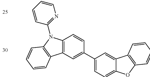
Formula 2A
