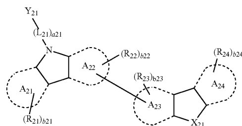
Formula 2
