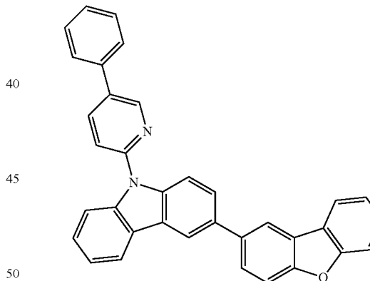
Formula 2B
