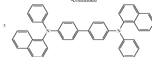
NPB
