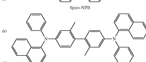
\alpha -NPB
