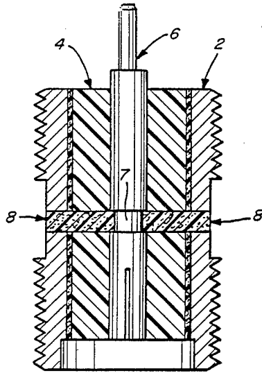
Fig. 1 (PRIOR ART)
