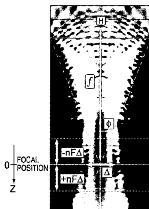
CROSS-SECTIONAL VIEW PARALLEL TO OPTICAL AXIS
