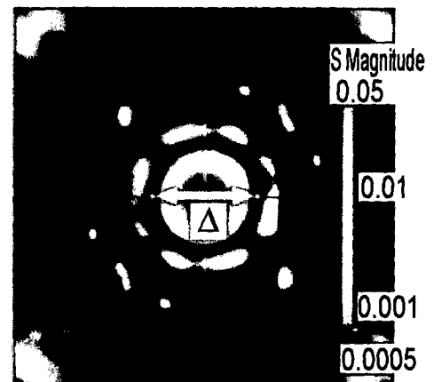
CROSS-SECTIONAL VIEW PERPENDICULAR TO OPTICAL AXIS
