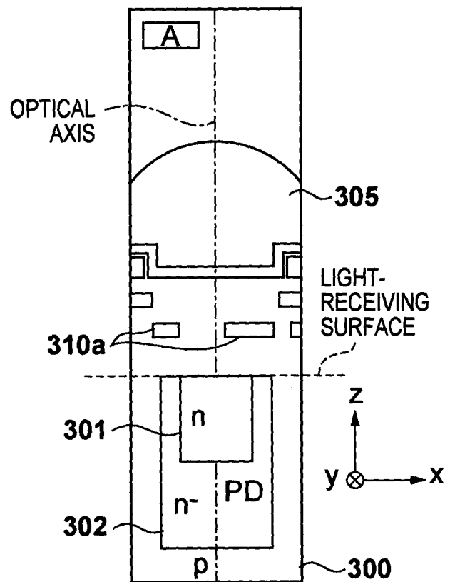
a-a CROSS-SECTIONAL VIEW
