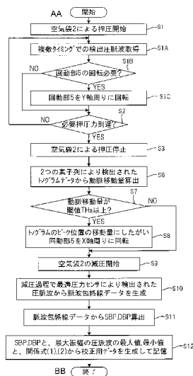
FIG. 6: S1 Start pressing by air bag 2 S1A Acquire pressure pulse waves detected at a plurality of timings S1B Is rotation by rotation unit 5 necessary? S1C Rotate rotation unit 5 about Y axis S2 Has necessary pressing force been reached? S3 Stop pressing by air bag 2 S6 Calculate amount of artery movement from tonogram data detected by two element rows S7 Is amount of artery movement equal to or greater than threshold value THa? S8 Rotate rotation unit 5 about X axis in accordance with amount of movement of tonogram peak position S9 Start reducing pressure of air bag 2 S10 Generate pulse wave envelope data from pressure pulse wave detected by optimum pressure sensor as pressure is reduced S11 Calculate SBP, DBP from pulse wave envelope data S12 Generate calibration data from SBP and DBP, maximum and minimum values of largest-amplitude pressure pulse wave, and relational expressions (1) and (2), and store calibration data AA Start BB End
