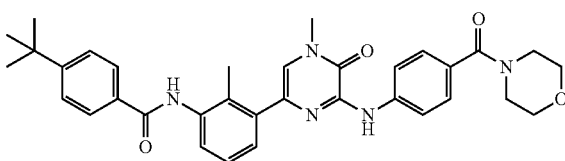
CGI-1746
