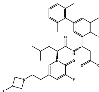
(S)-3-(4-fluoro-2',5,6'-trimethyl-[1,1'-biphenyl]-3-yl)-3-((S)-2-(3-fluoro-5-(2-(3-fluoroazetidin-1-yl)ethyl)-2-oxopyridin-1(2H)-yl)-4-methylpentanamido)propanoic acid
