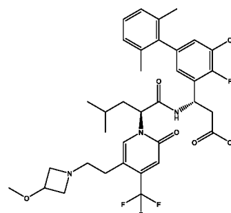
(S)-3-(5-chloro-4-fluoro-2',6'-dimethyl-[1,1'-biphenyl]-3-yl)-3-((S)-2-(5-(2-(3-methoxyazetidin-1-yl)ethyl)-2-oxo-4-(trifluoromethyl)pyridin-1(2H)-yl)-4-methylpentanamido)propanoic acid;
