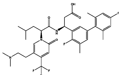
(S)-3-(4,4'-difluoro-2',5,6'-trimethyl-[1,1'-biphenyl]-3-yl)-3-((S)-2-(5-(2-(dimethylamino)ethyl)-2-oxo-4-(trifluoromethyl)pyridin-1(2H)-yl)-4-methylpentanamido)propanoic acid;
