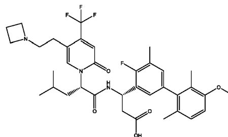
(S)-3-((S)-2-(5-(2-(azetidin-1-yl)ethyl)-2-oxo-4-(trifluoromethyl)pyridin-1(2H)-yl)-4-methylpentanamido)-3-(4-fluoro-3'-methoxy-2',5,6'-trimethyl-[1,1'-biphenyl]-3-yl)propanoic acid;
