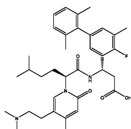
(S)-3-((S)-2-(5-(2-(dimethylamino)ethyl)-4-methyl-2-oxopyridin-1(2H)-yl)-5-methylhexanamido)-3-(4-fluoro-2',5,6'-trimethyl-[1,1'-biphenyl]-3-yl)propanoic acid;
