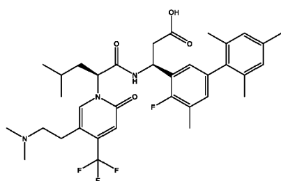
(S)-3-((S)-2-(5-(2-(dimethylamino)ethyl)-2-oxo-4-(trifluoromethyl)pyridin-1(2H)-yl)-4-methylpentanamido)-3-(4-fluoro-2',4',5,6'-tetramethyl-[1,1'-biphenyl]-3-yl)propanoic acid;
