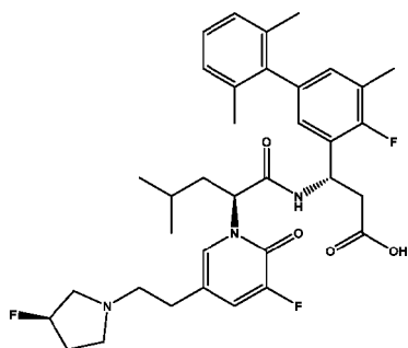
(S)-3-(4-fluoro-2',5,6'-trimethyl-[1,1'-biphenyl]-3-yl)-3-((S)-2-(3-fluoro-5-(2-((R)-3-fluoropyrrolidin-1-yl)ethyl)-2-oxopyridin-1(2H)-yl)-4-methylpentanamido)propanoic acid
