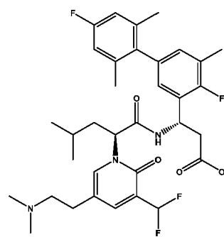
(S)-3-(4,4'-difluoro-2',5,6'-trimethyl-[1,1'-biphenyl]-3-yl)-3-((S)-2-(5-(2-(difluoromethyl)-5-(2-(dimethylamino)ethyl)-2-oxopyridin-1(2H)-yl)-4-methylpentanamido)propanoic acid;
