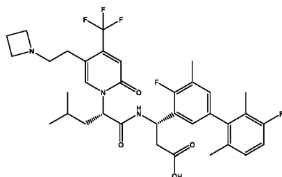
(S)-3-((S)-2-(5-(2-(azetidin-1-yl)ethyl)-2-oxo-4-(trifluoromethyl)pyridin-1(2H)-yl)-4-methylpentanamido)-3-(3',4-difluoro-2',5,6'-trimethyl-[1,1'-biphenyl]-3-yl)propanoic acid;
