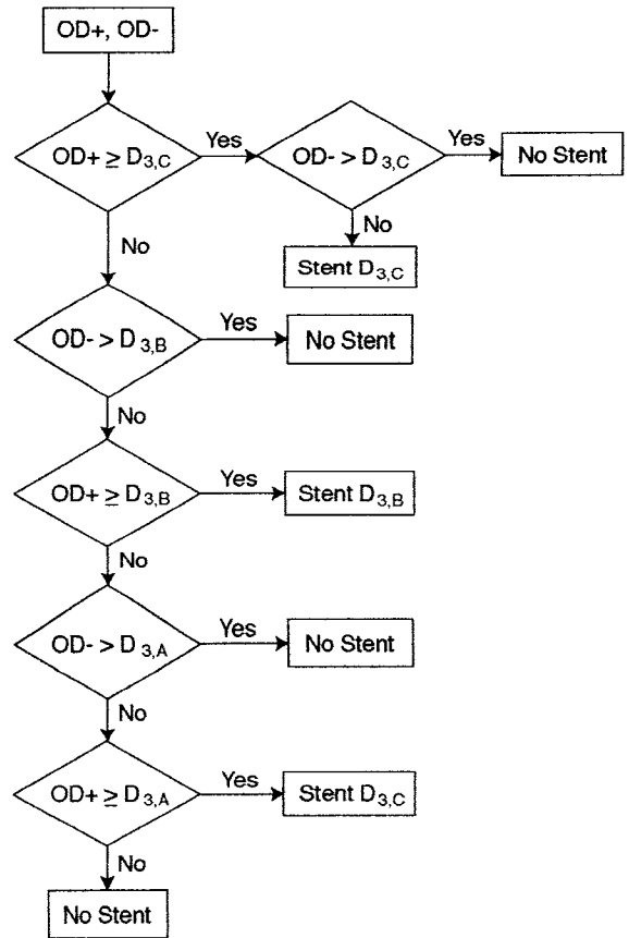
Algorithm 2 (largest stent)
