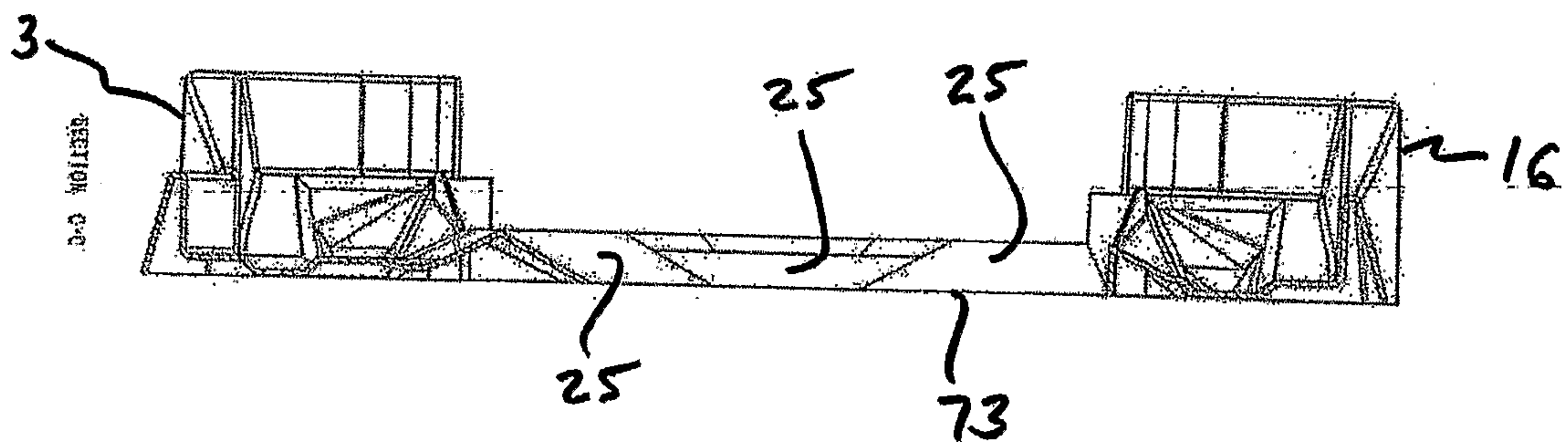
Cross Section C-C
