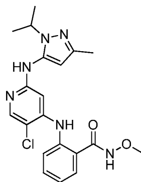
Formula (I-c2)
