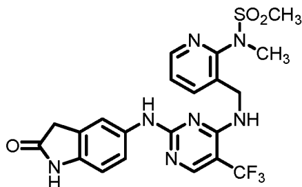
Formula (I-e)
