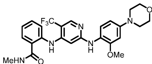
Formula (I-a)
