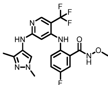
Formula (I-f)
