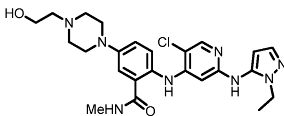
Formula (I-c3)
