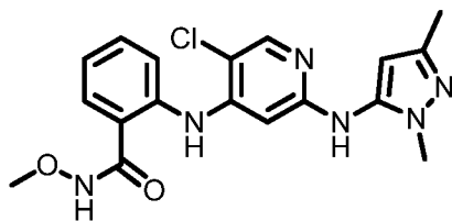
Formula (I-c5)
