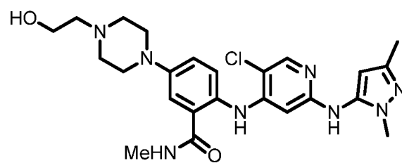
Formula (I-c4)
