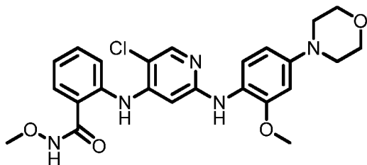
Formula (I-c1)
