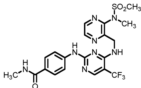
Formula (I-d)
