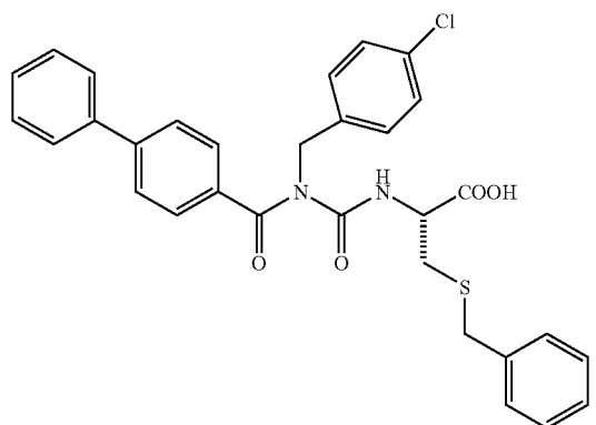
71A: N-(4-chloro)-benzyl-4-phenylbenzamide
