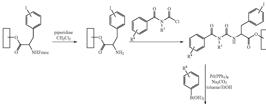
Scheme 13: Introduction of diversity via Suzuki coupling on 4- or 3-iodophenylalanine.
