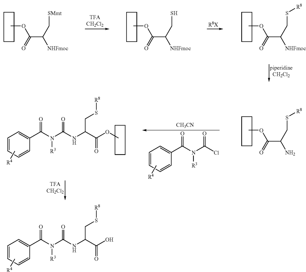
Scheme 11: Solid phase synthesis where the amino acid is a cysteine or derivative thereof.
