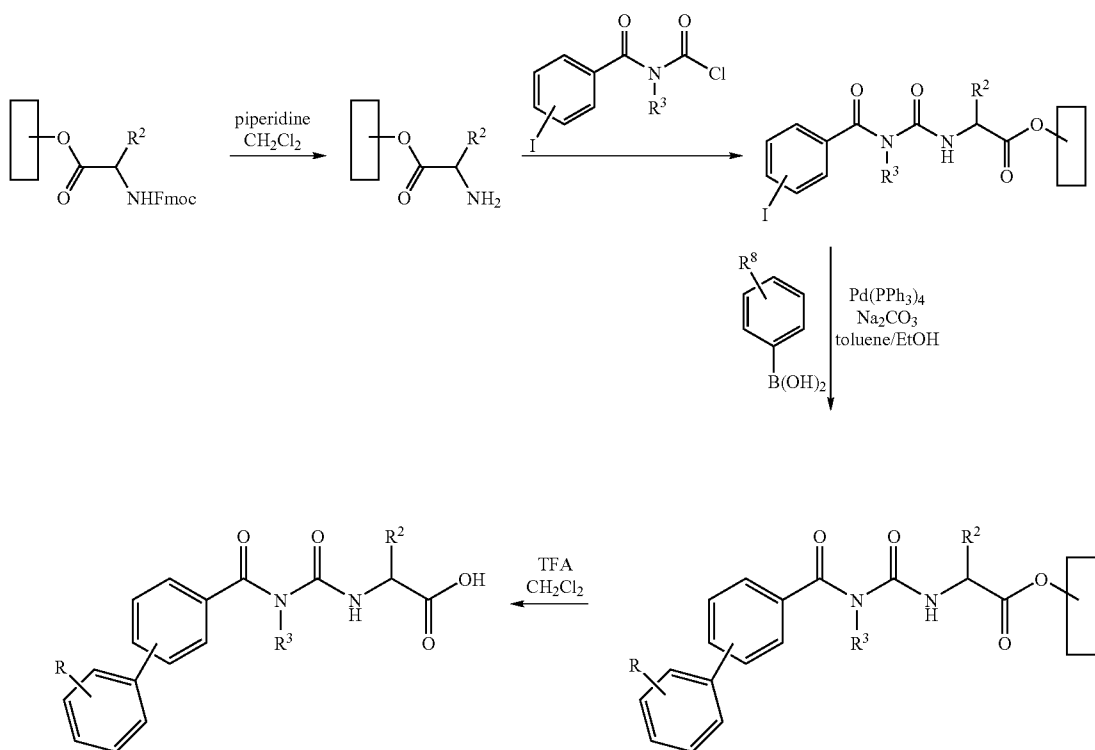
Scheme 14: Introduction of diversity via Suzuki coupling on a 3- or 4-iodobenzoylurea; where R is one or more optional substituents
