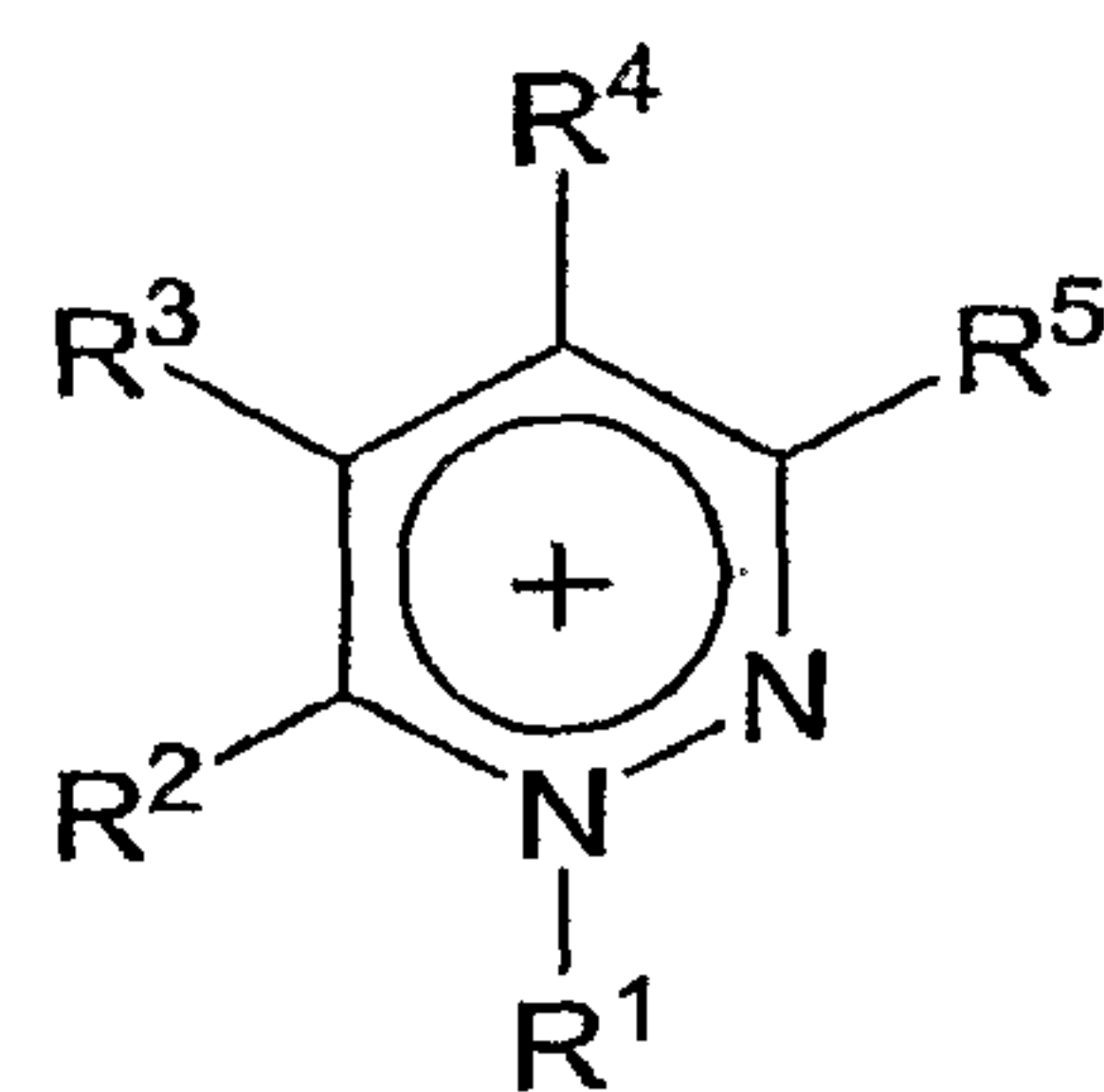
Pyridazinium
