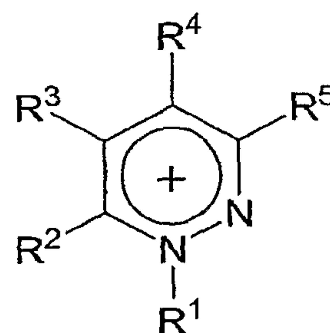
Pyridazinium
