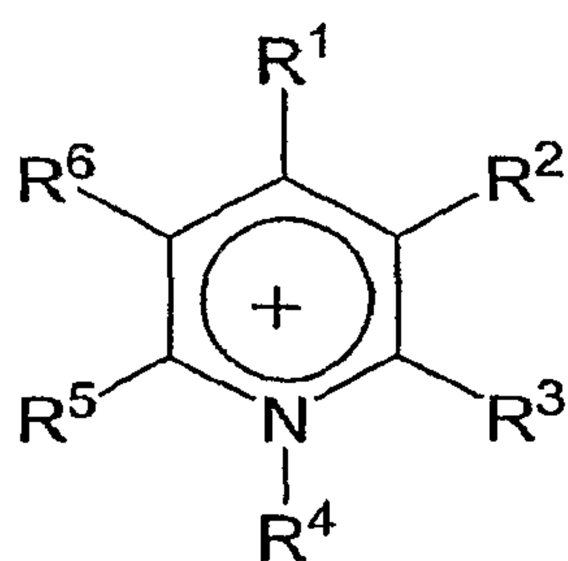
Pyridinium
