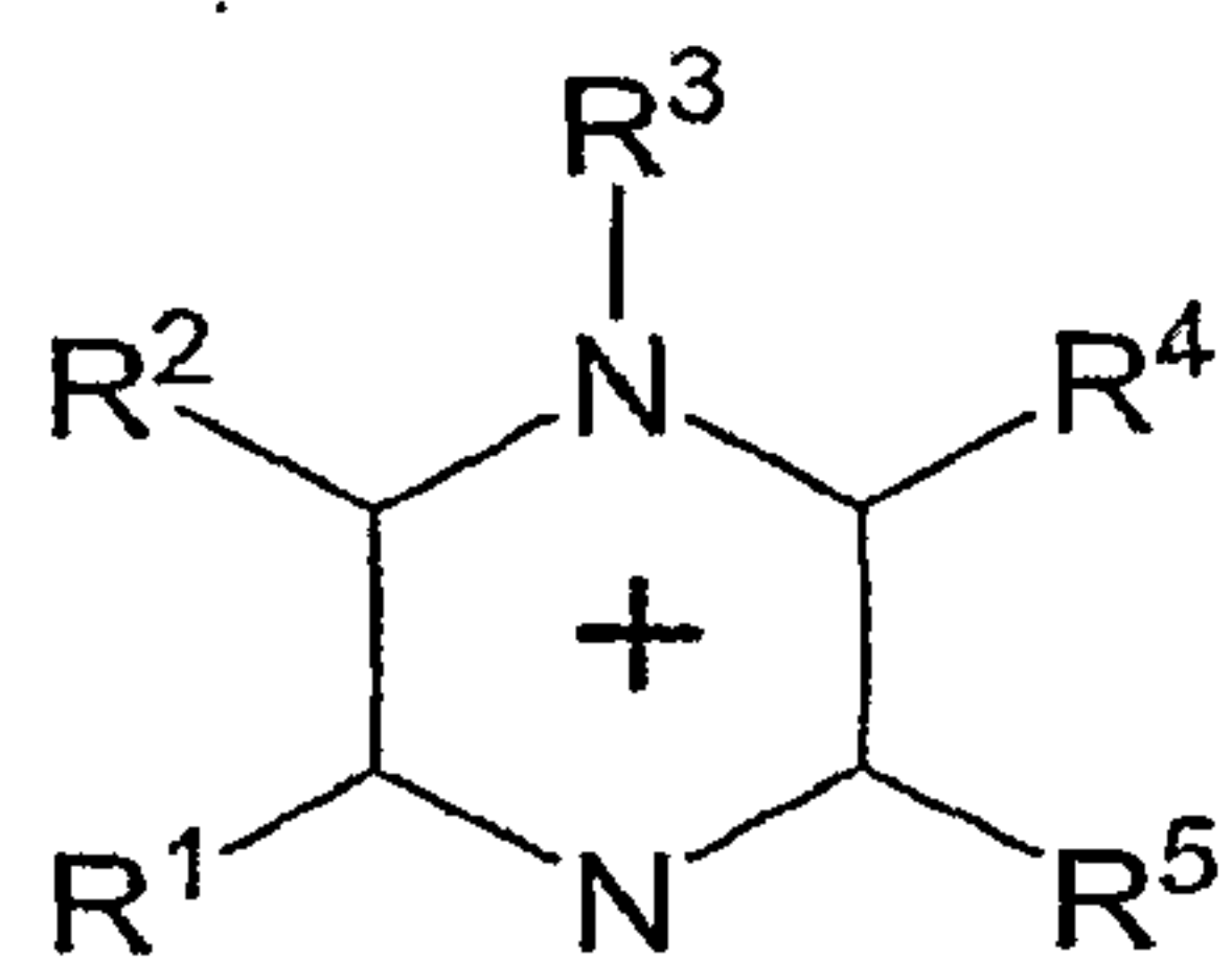
Pyrimidinium
