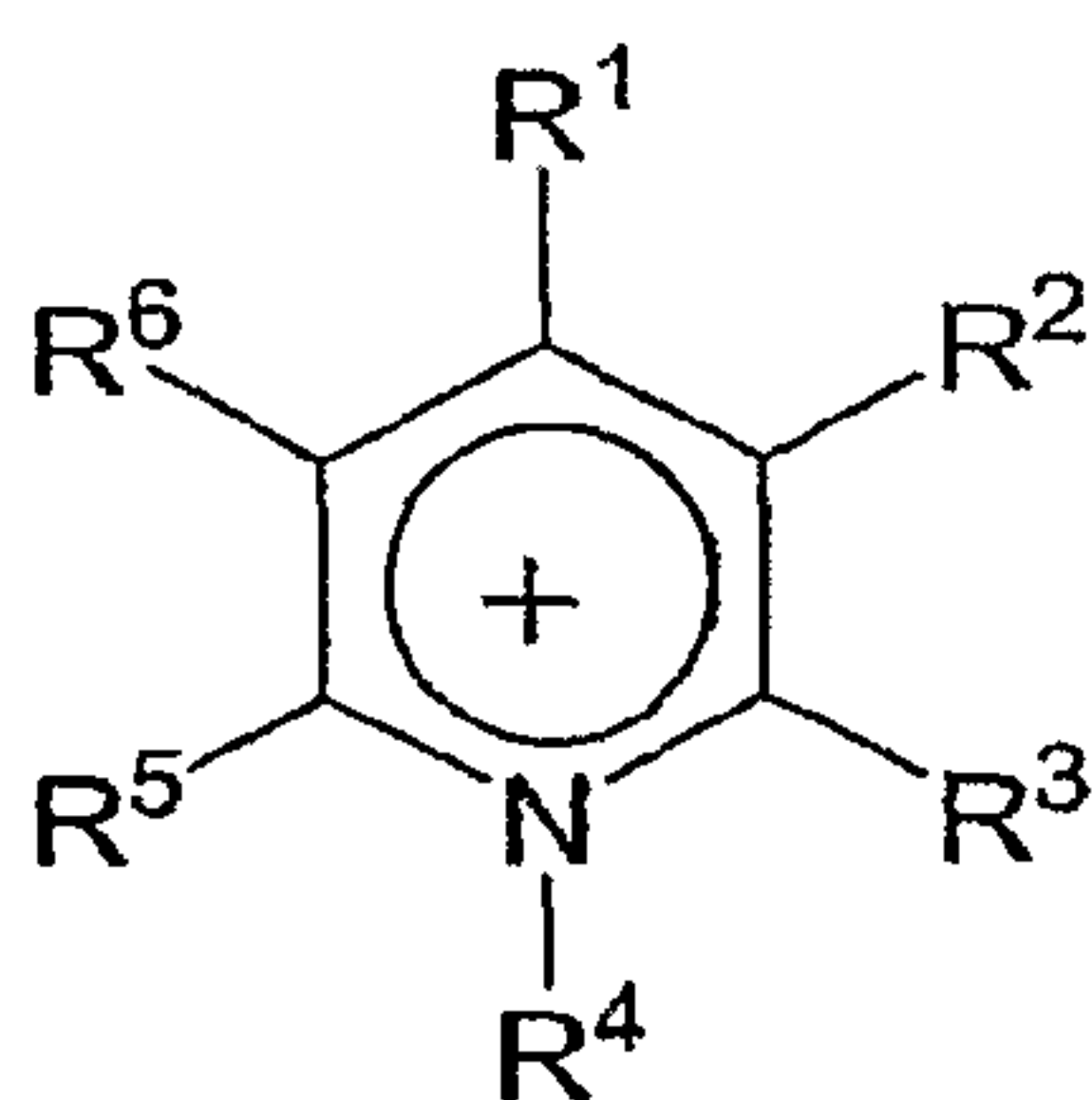
Pyridinium
