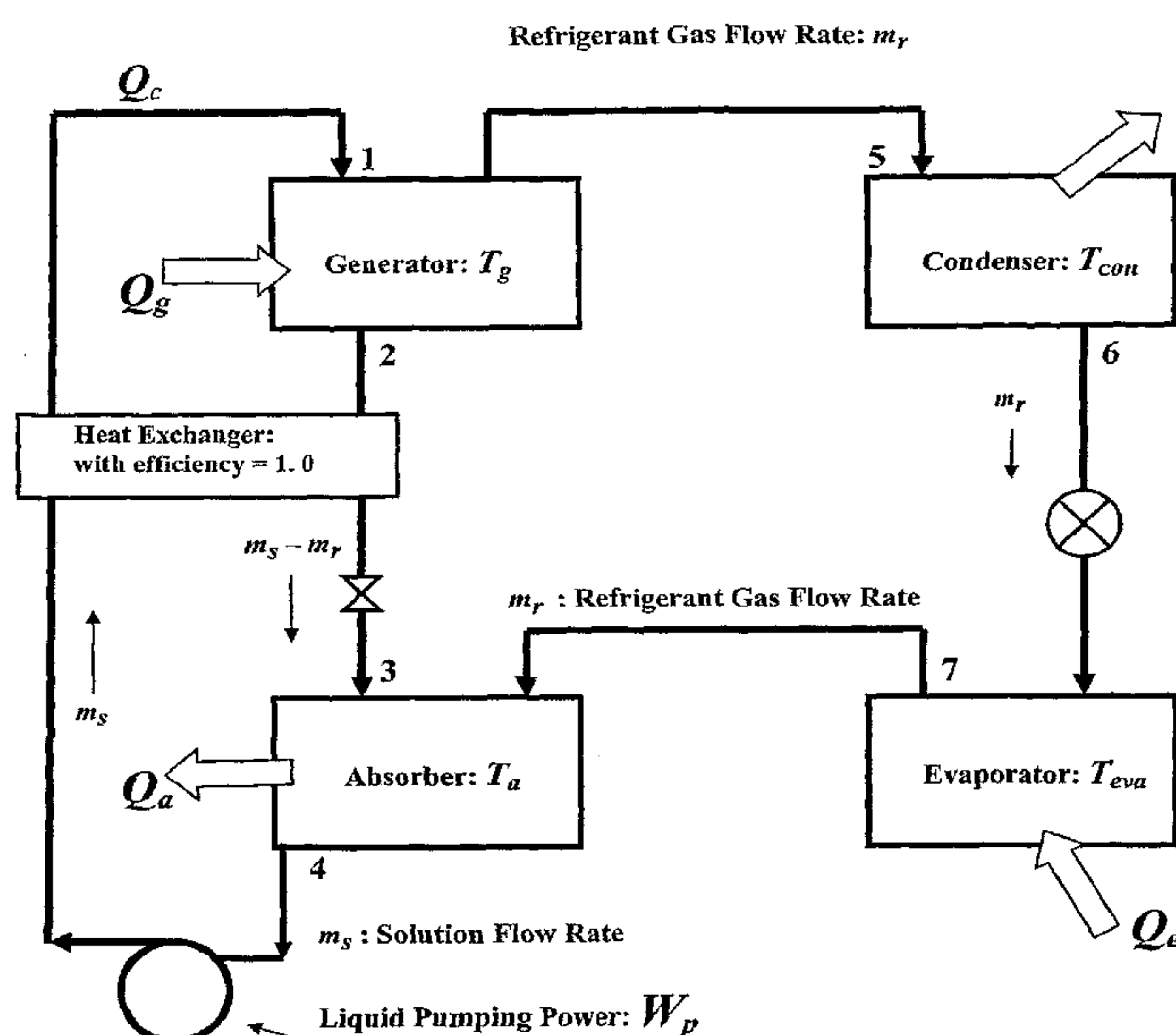
A schematic diagram of a simple absorption refrigeration cycle
